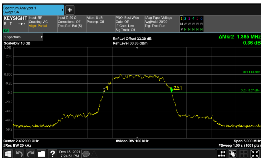
Figure 110 - Core 1 (B) 2402 MHz (CH0) 20 dB Bandwidth
