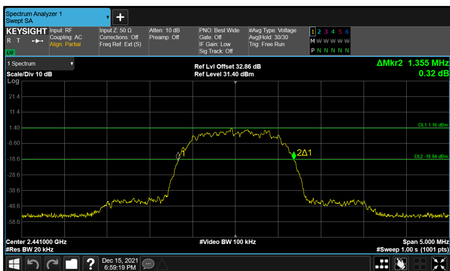
Figure 101 - Core 0 (A) 2441 MHz (CH39) 20 dB Bandwidth
