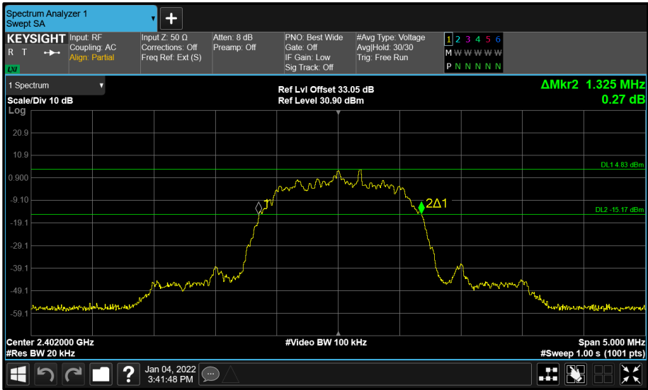
Figure 103 - Core 2 (C) 2402 MHz (CH0) 20 dB Bandwidth
