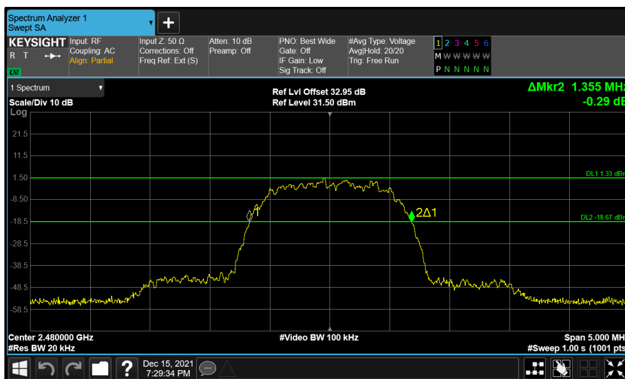
Figure 119 - Core 0 (A) 2480 MHz (CH78) 20 dB Bandwidth
