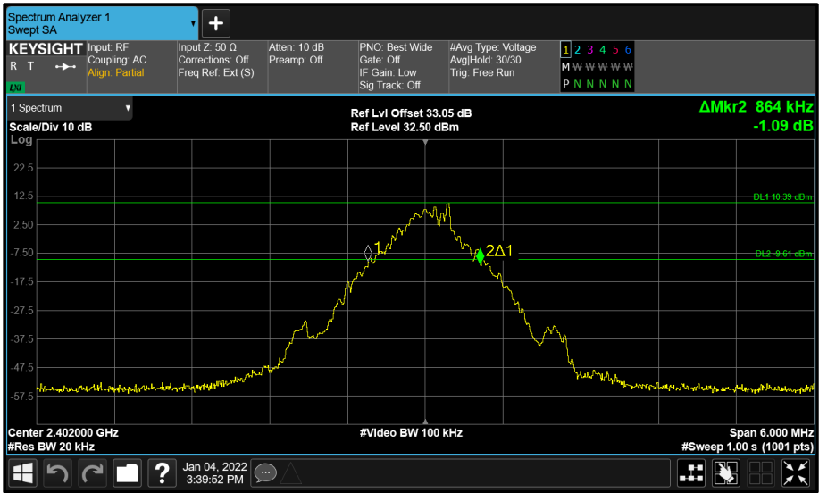
Figure 88 - Core 2 (C) 2402 MHz (CH0) 20 dB Bandwidth
