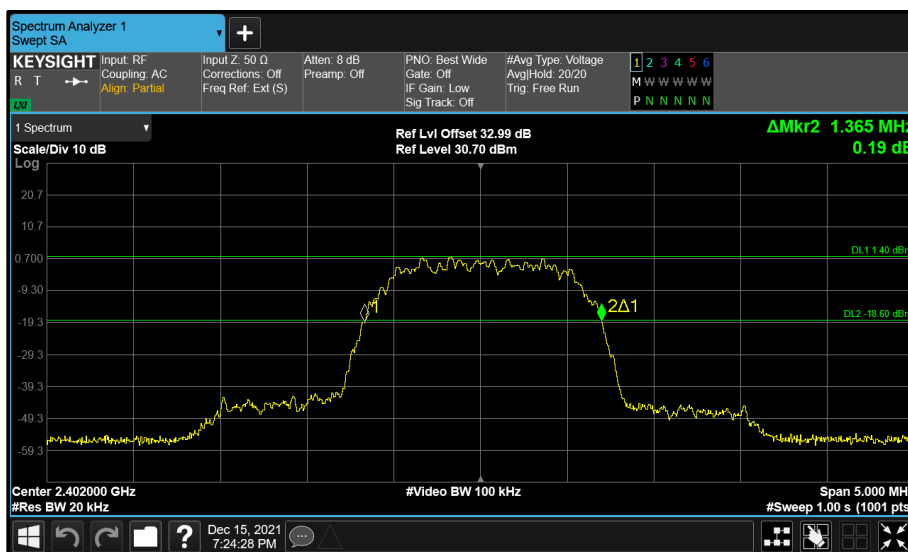
Figure 109 - Core 0 (A) 2402 MHz (CH0) 20 dB Bandwidth
