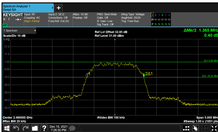
Figure 113 - Core 0 (A) 2480 MHz (CH78) 20 dB Bandwidth
