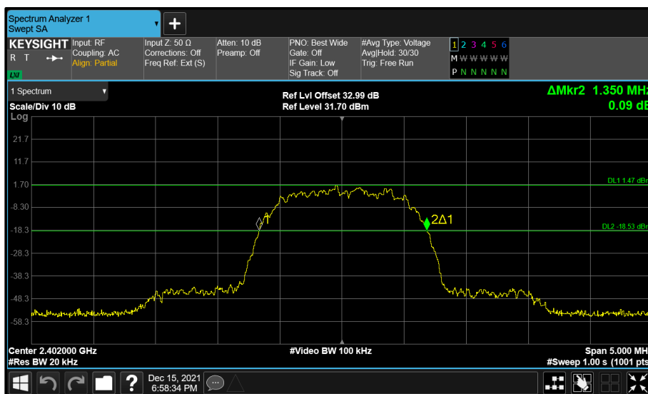
Figure 100 - Core 0 (A) 2402 MHz (CH0) 20 dB Bandwidth
