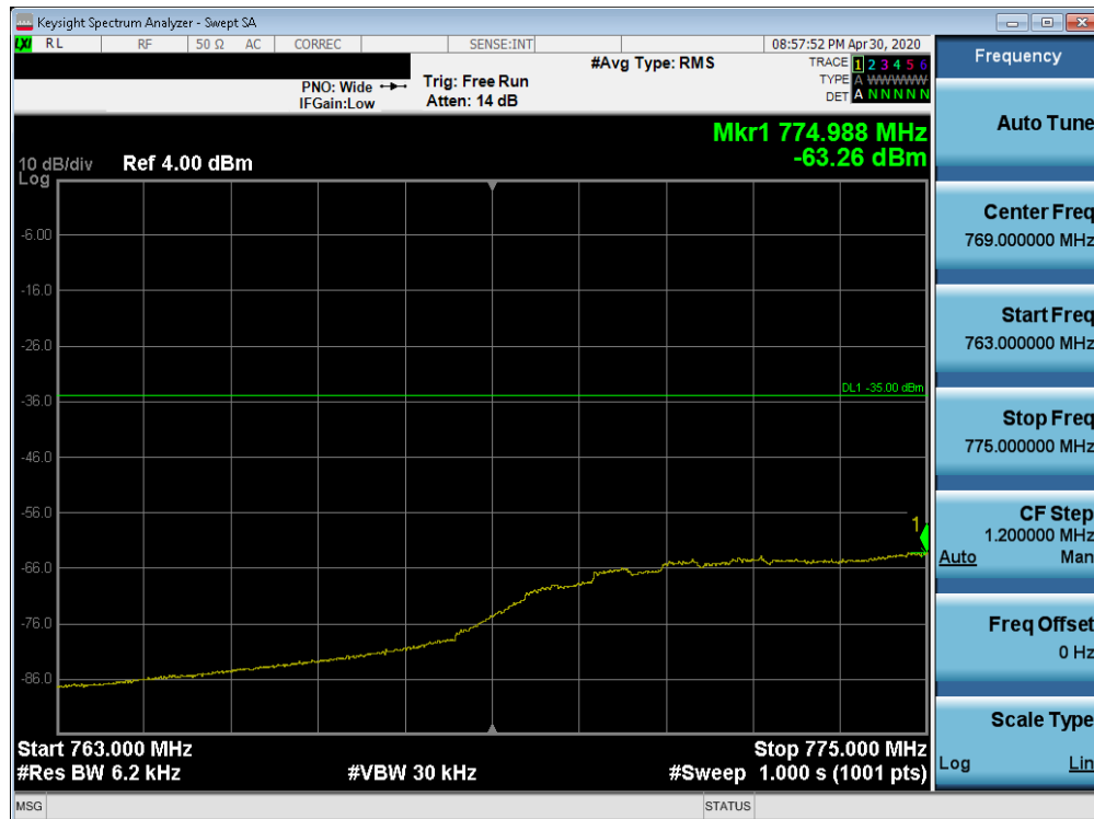
Plot 7-141. Lower Emission Mask Edge Plot (Band 13 - 10.0MHz QPSK - Full RB Configuration)
