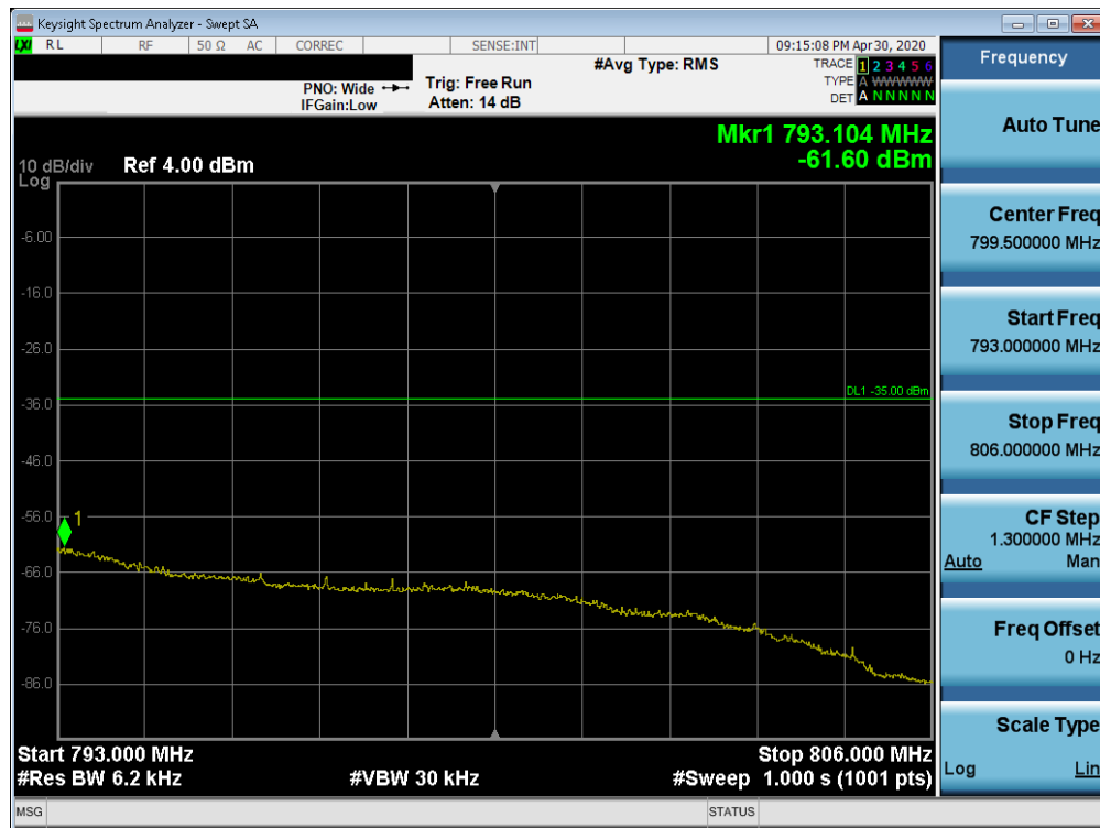
Plot 7-139. Higher Emission Mask Edge Plot (Band 13 - 5.0MHz QPSK - Full RB Configuration)
