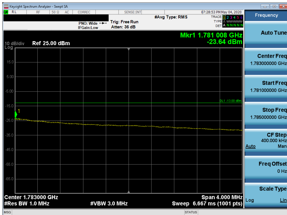
Plot 7-179. Upper Extended Band Edge Plot (Band 66 - 15.0MHz QPSK - Full RB Configuration)
