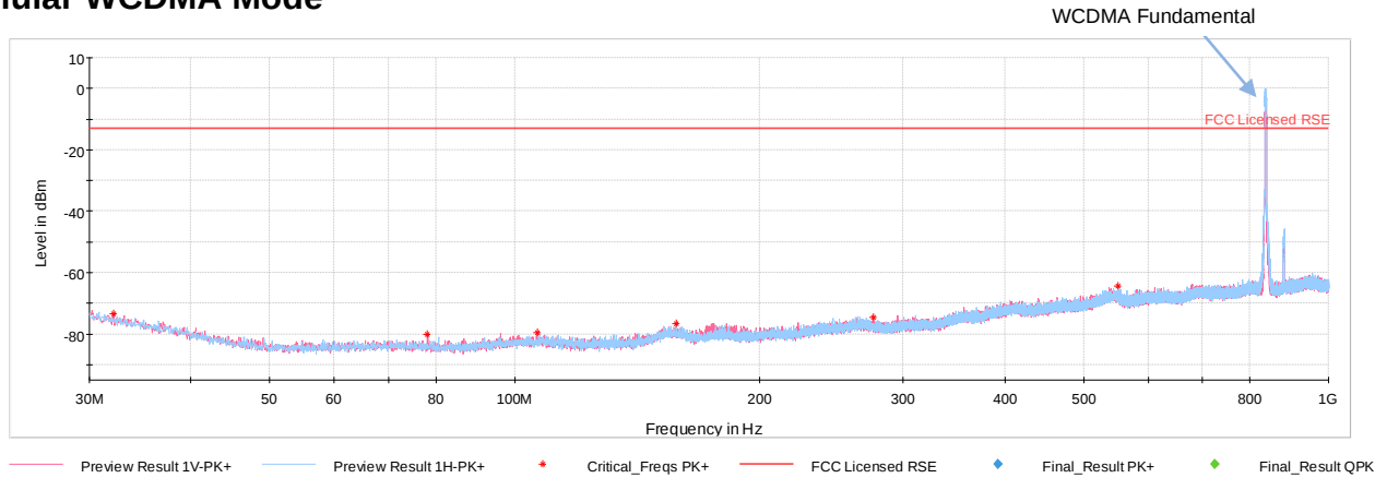
Plot 7-44. Radiated Spurious Emissions below 1GHz (Cellular WCDMA Mode – Ch. 4183)
