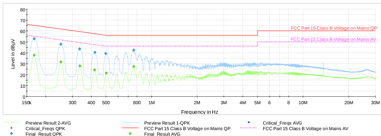
Plot 7-13. AC Line-Conducted Test Plot (N, with WCP + AC/DC Adapter)
