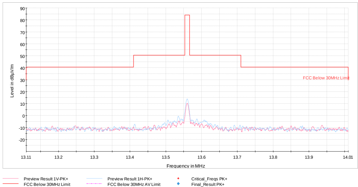
Plot 7-7. In Band Radiated Spurious Emissions (Reader 10% Ask 1 out of 256, with WCP + AC/DC Adapter)
