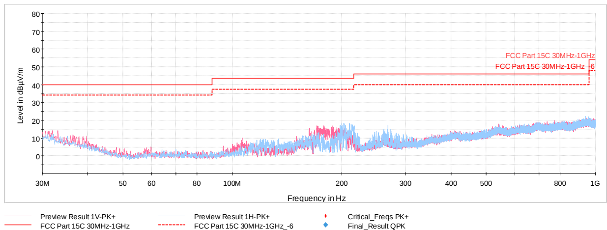
Plot 7-11. Radiated Spurious Emissions 30MHz – 1GHz (Reader 10% Ask 1 out of 256, with WCP + AC/DC Adapter)
