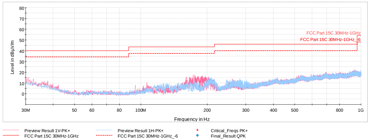
Plot 7-10. Radiated Spurious Emissions 30MHz – 1GHz (CE A 848kbps, with WCP + AC/DC Adapter)
