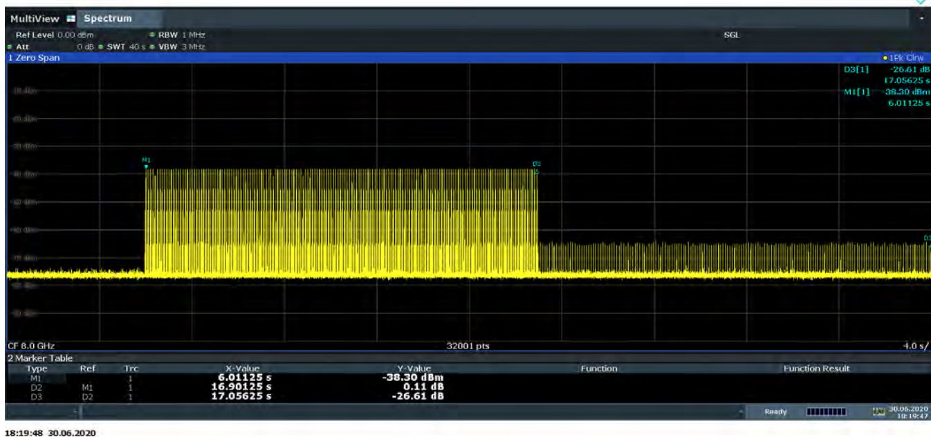
Plot 7-84. Cessation Time – Mode1 (Ch. 9, 8 GHz)
