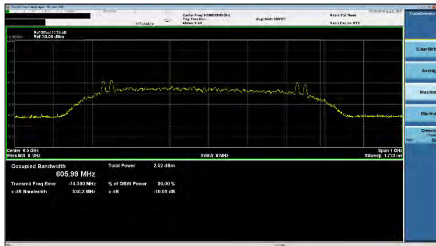
Plot 7-23. ISSED Occupied Bandwidth (Ch. 5, Config 0/Payload 125)
