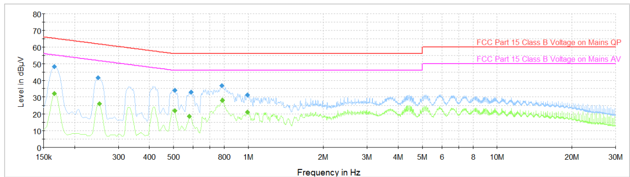
Plot 7-40. AC Line-Conducted Plot – GFSK ePA Ch.39 (N, with WCP + AC/DC Adapter)
