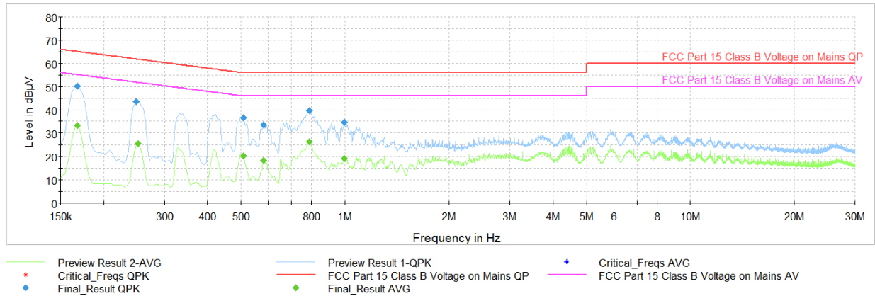
Plot 7-39. AC Line-Conducted Plot – GFSK ePA Ch.39 (L1, with WCP + AC/DC Adapter)
