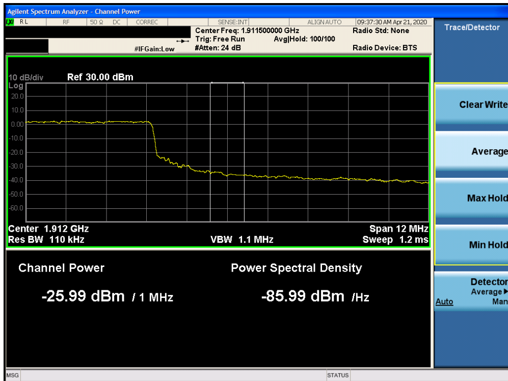
Plot 7-251. Upper Extended Band Edge Plot (Band 2 - 15.0MHz QPSK - Full RB Configuration)
