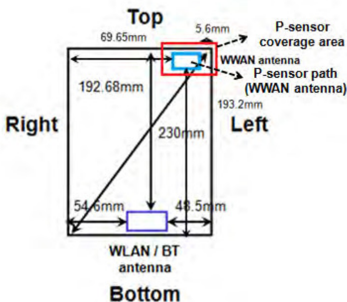
Back view of the tablet
