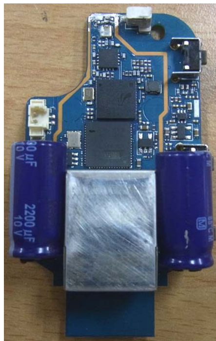
PCB Top without Shield
