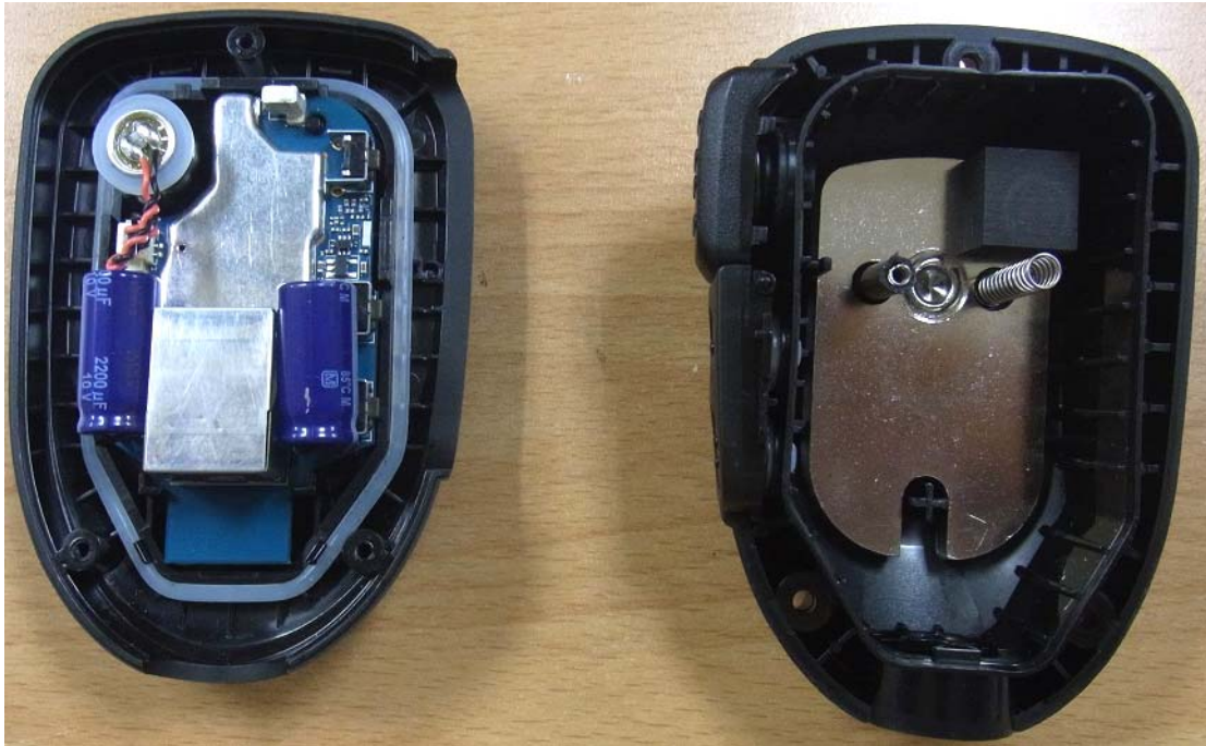
Overall Internal Assembly
