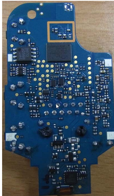
PCB Bottom without Shield
