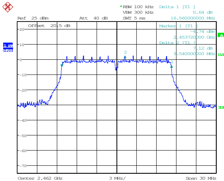
Figure 7.2.2-8: 6dB BW - Middle Channel
