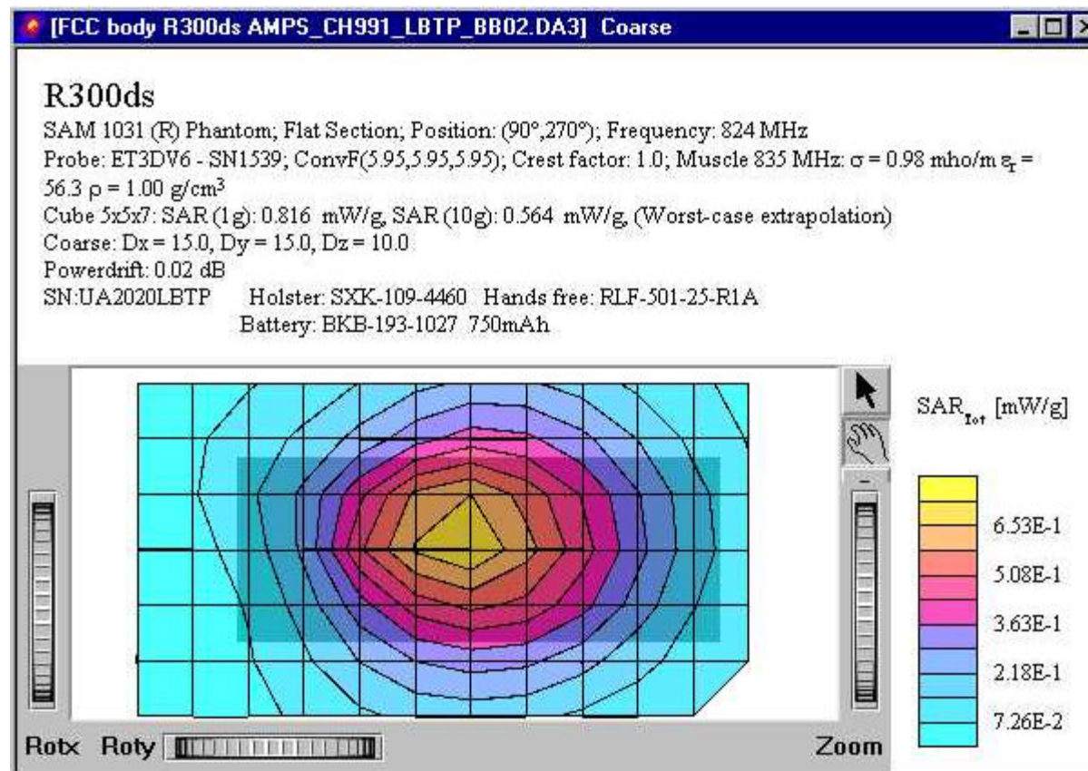
Distribution of maximum SAR in 800 AMPS band. Measured against the body using
