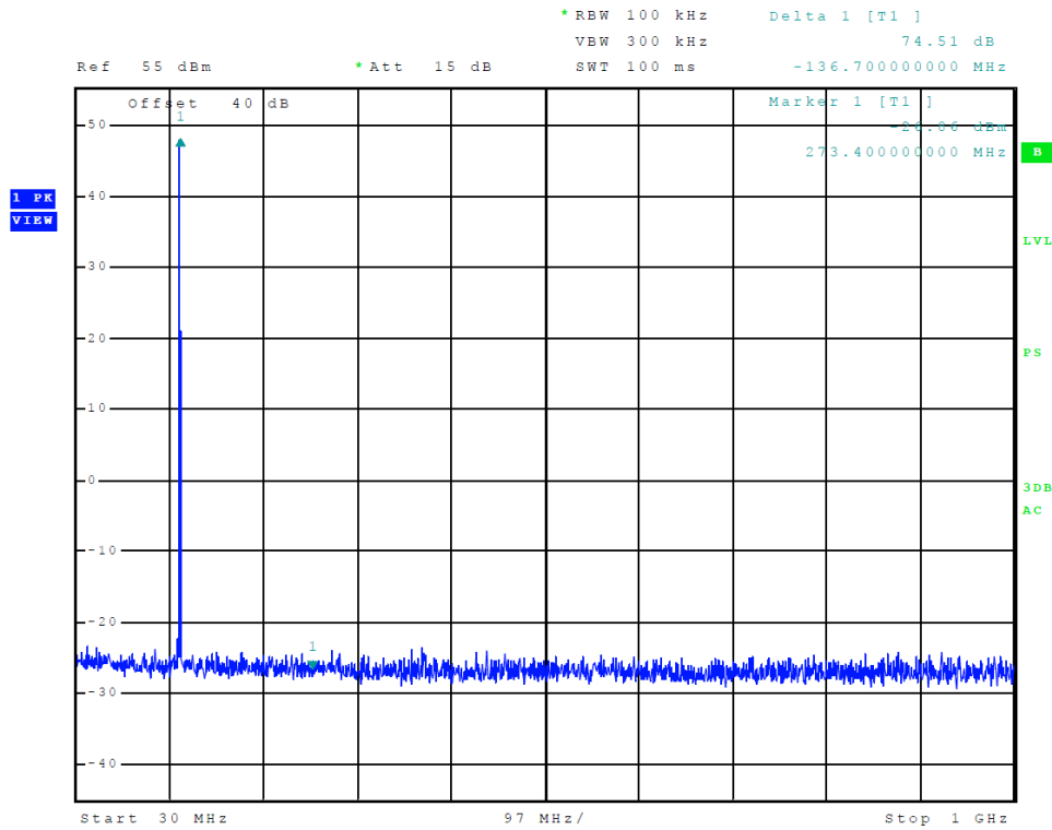
Figure 9 Spurious Emissions at Antenna Terminal 118-136.975 MHz (25 kHz)
