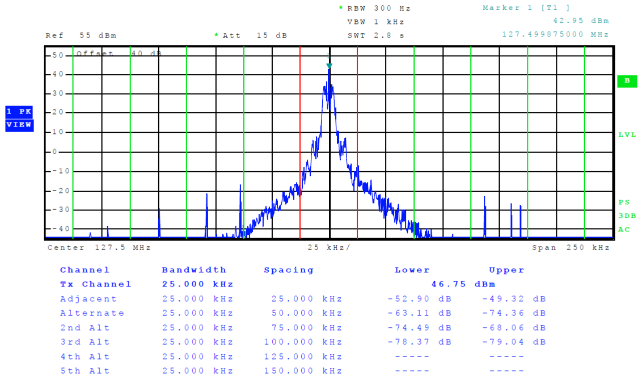
Figure 16 Adjacent Channel Power (ACARS)
