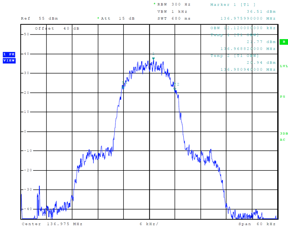
Figure 8 Occupied Band Width (VDL mode 2, 118.000-136.975 MHz)
