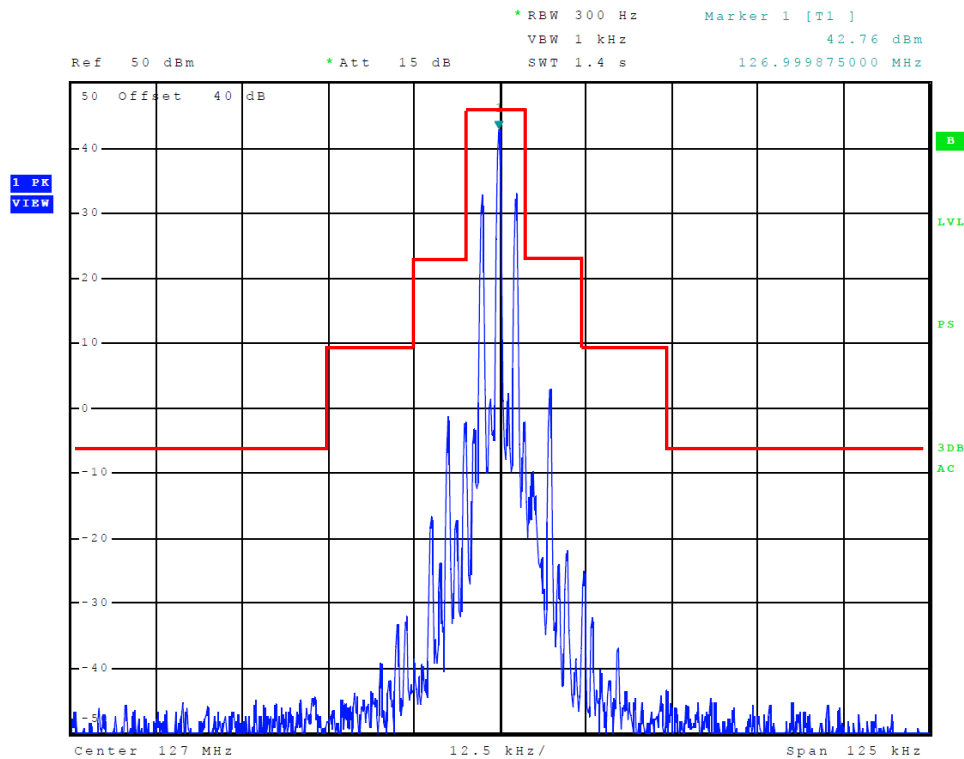
Figure 12 Emission Mask at Antenna Terminal 118-136.992 MHz (8.33 kHz)
