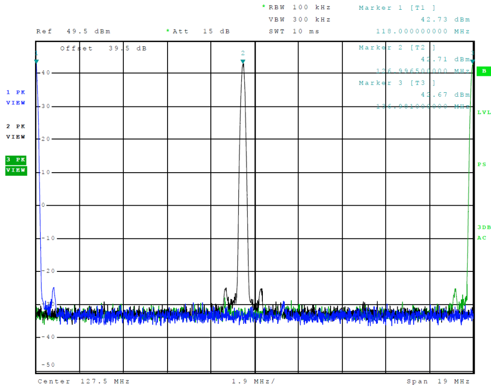
Figure 1 Power Output Across Frequency Band 118-136.975 MHz (25 kHz mode)
