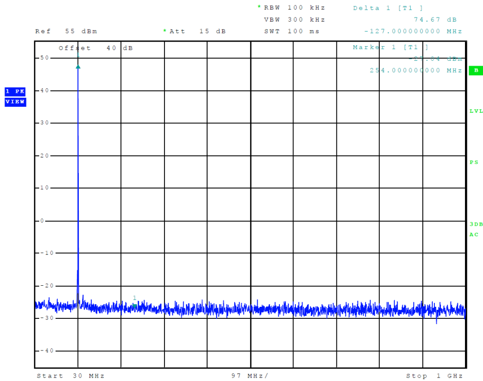
Figure 11 Spurious Emissions at Antenna Terminal 118-136.992 MHz (8.33 kHz)
