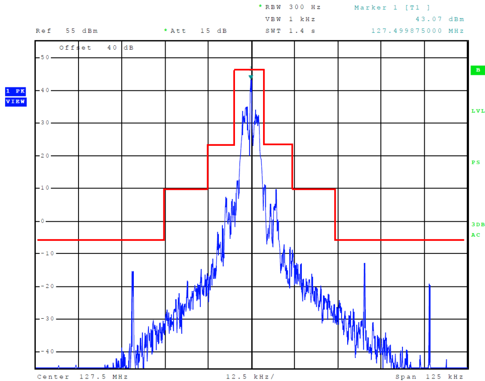
Figure 14 Emission Mask at Antenna Terminal 118-136.975 MHz (ACARS 25 kHz)
