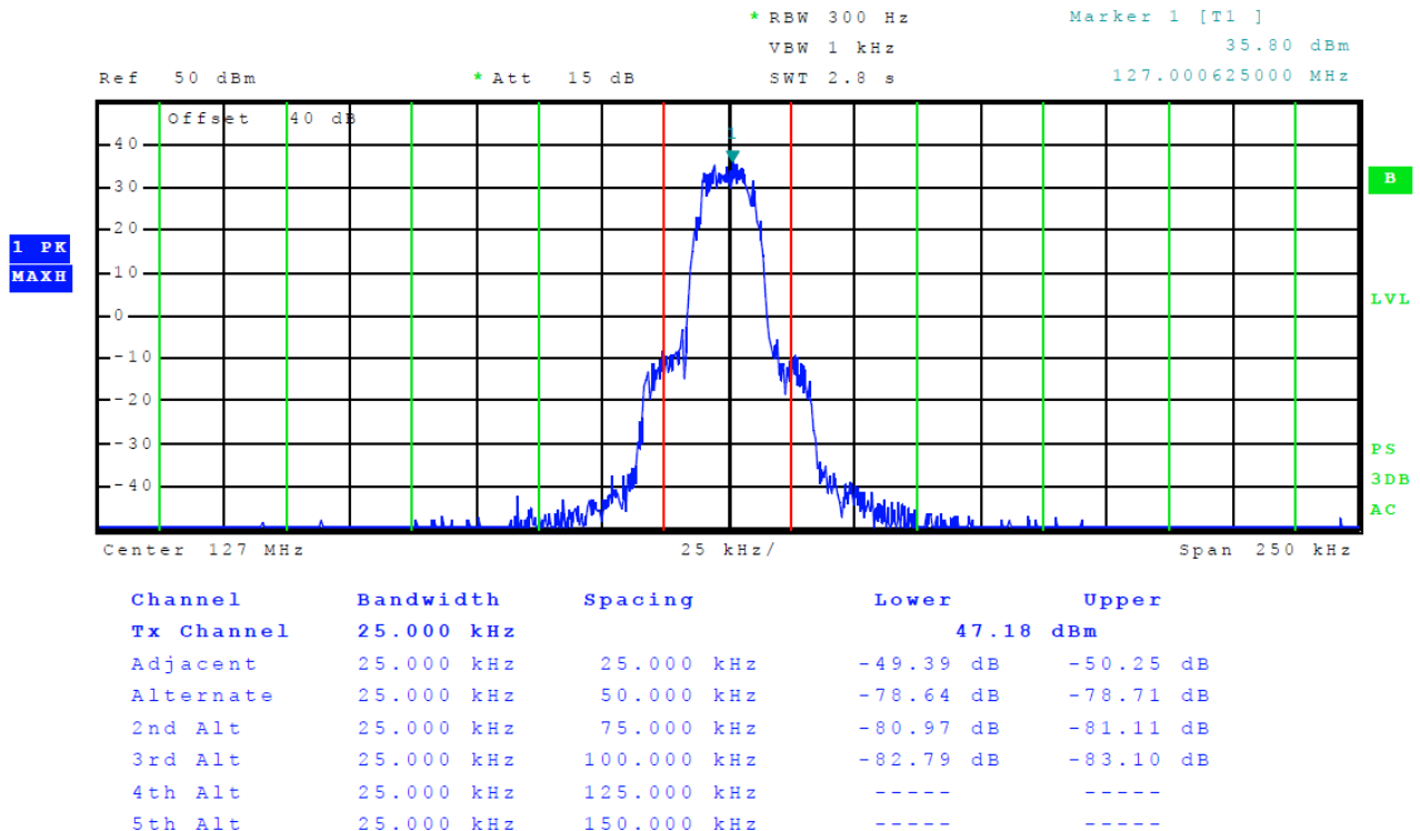
Figure 17 Adjacent Channel Power (VDL Mode 2)
