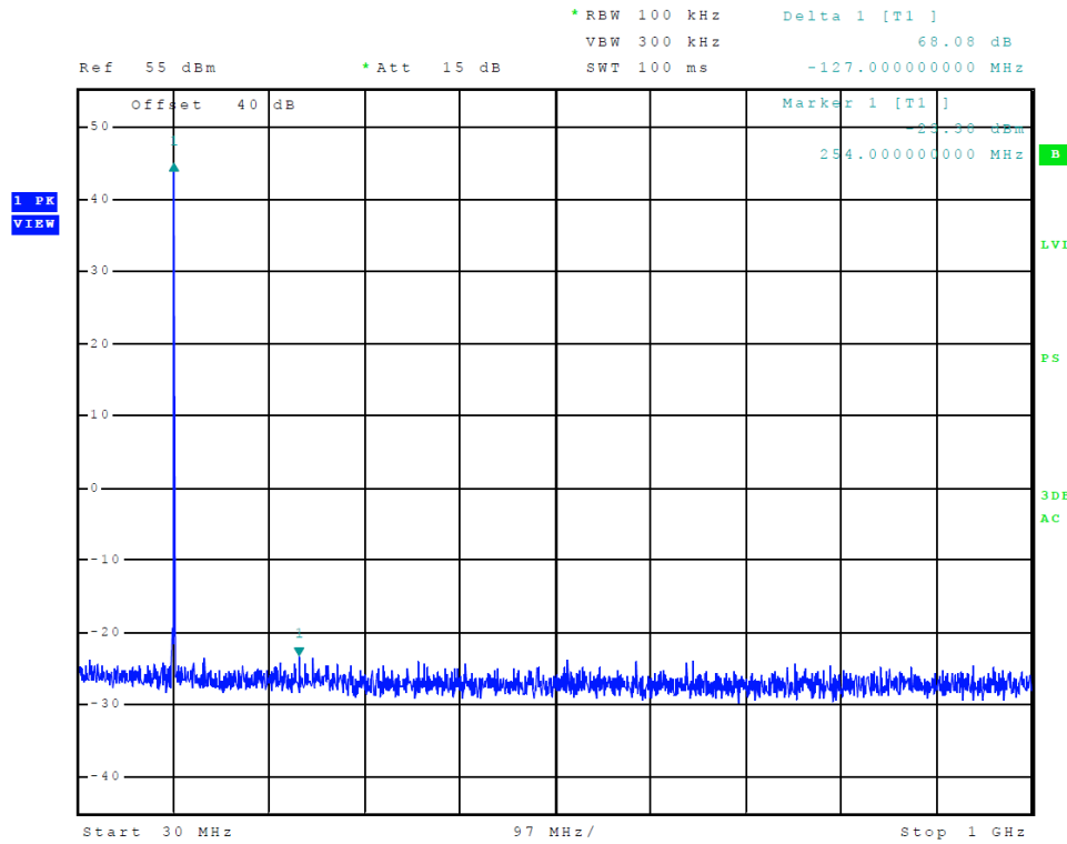
Figure 15 Spurious Emissions at Antenna Terminal 118-136.975 MHz (VDL Mode 2, 25 kHz)
