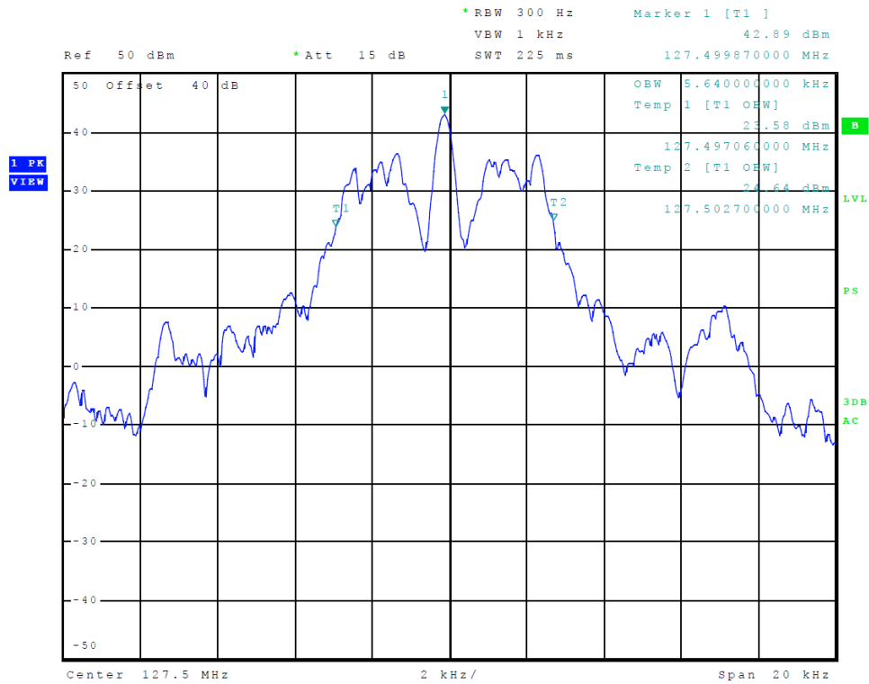
Figure 7 Occupied Band Width (ACARS mode, 118.000-136.975 MHz)
