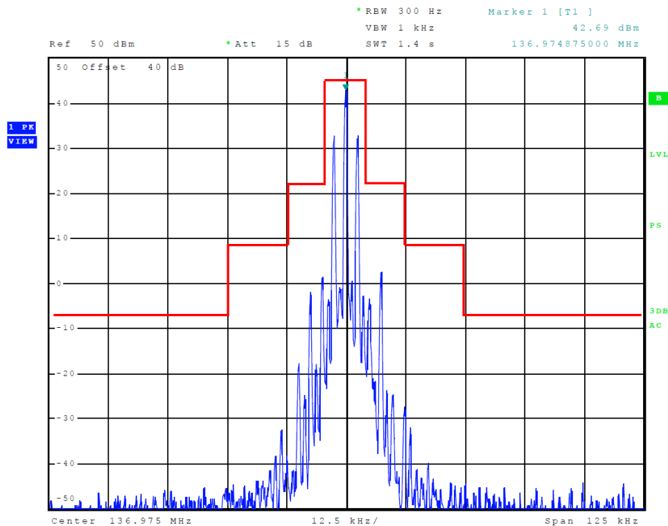
Figure 10 Emission Mask at Antenna Terminal 118-136.975 MHz (25 kHz)
