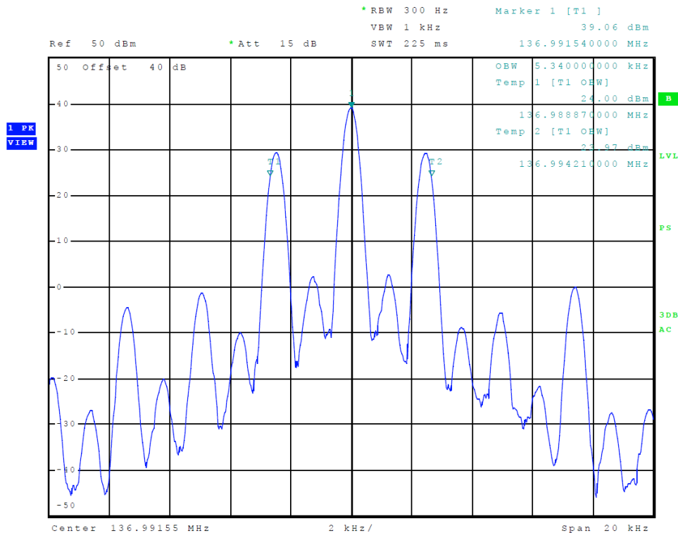
Figure 6 Occupied Band Width (8.33 kHz channels 118.000-136.992 MHz)
