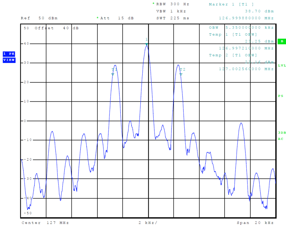
Figure 5 Occupied Band Width (25 kHz channels 118.000-136.975 MHz)
