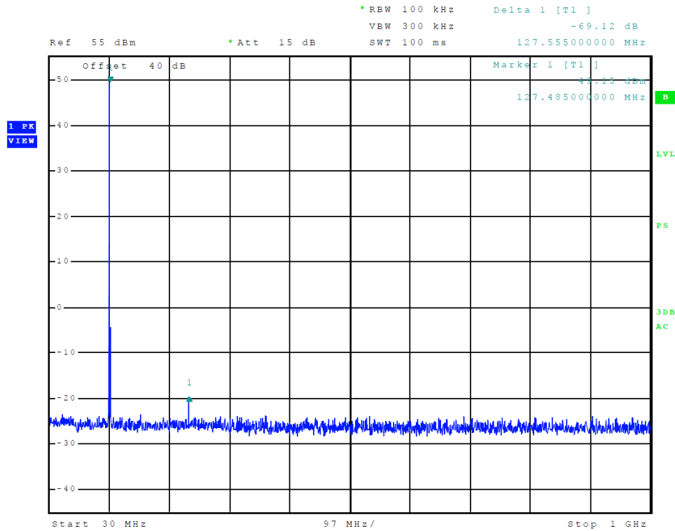
Figure 13 Spurious Emissions at Antenna Terminal 118-136.975 MHz (ACARS, 25 kHz)
