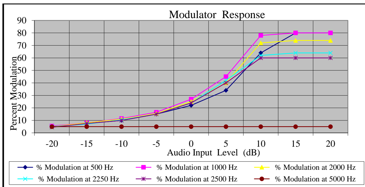
Figure 3 Modulation Characteristics
