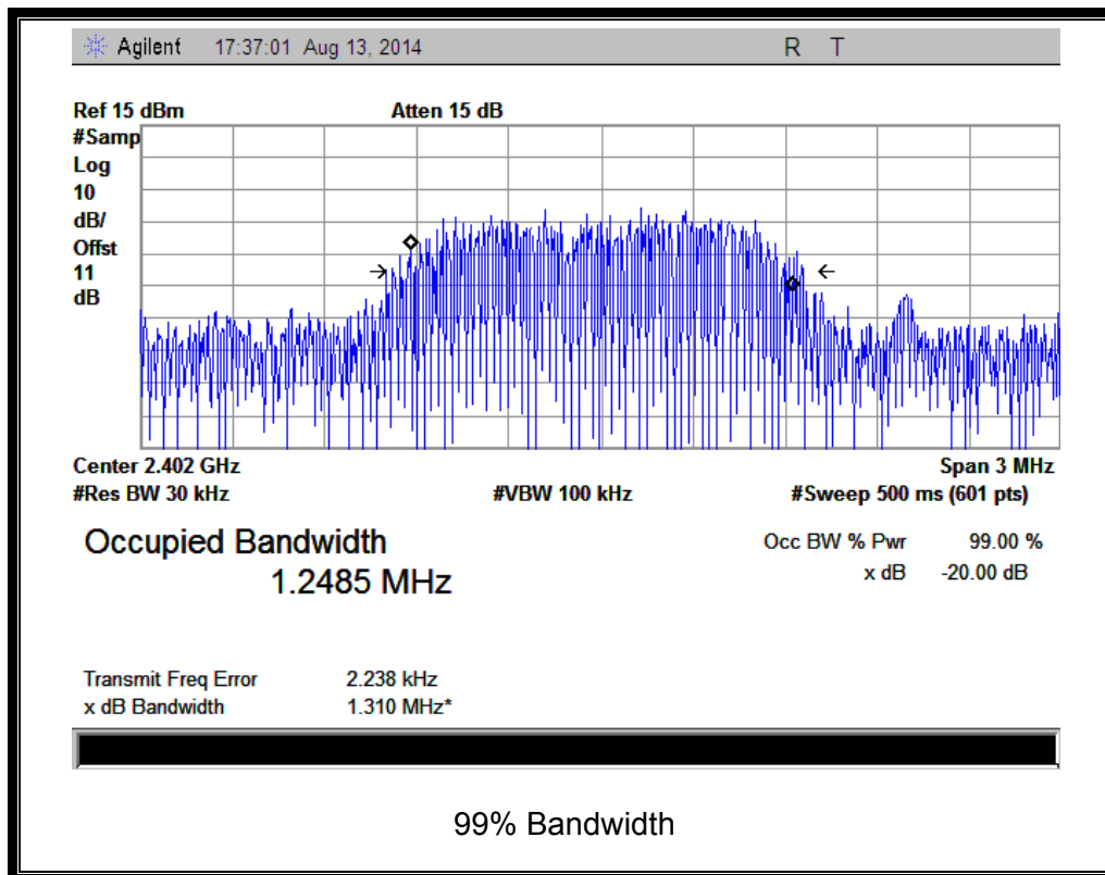
(Plot A: Channel = 2402 @ \pi/4 -DQPSK)
