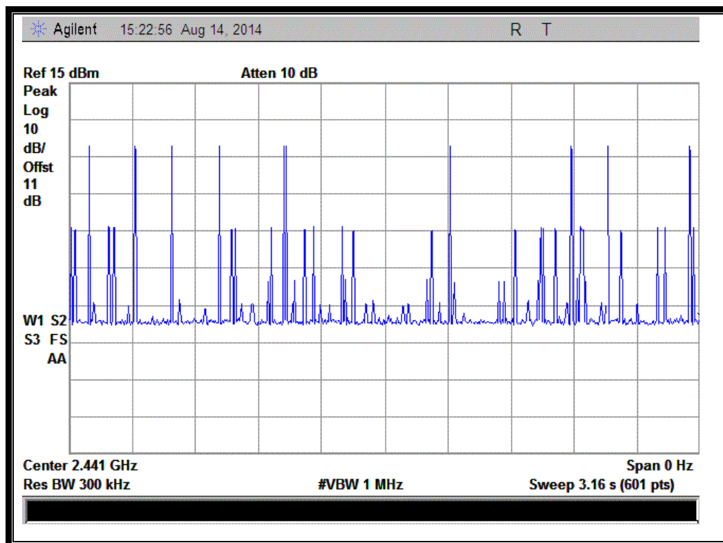
(Plot C: DH5 @ 8-DPSK)
