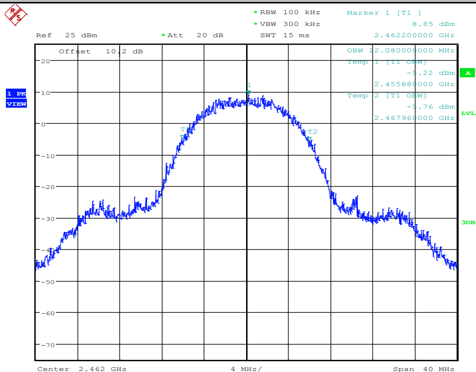
99% Occupied Bandwidth_11B_2462_Ant1
