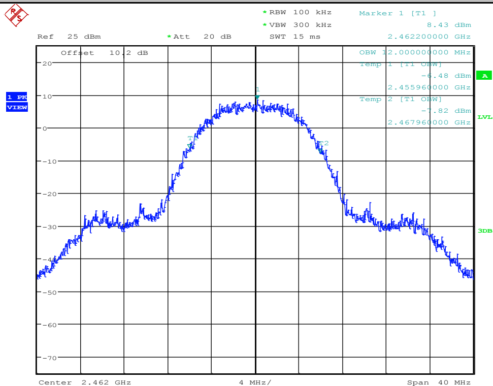
99% Occupied Bandwidth_11B_2462_Ant2
