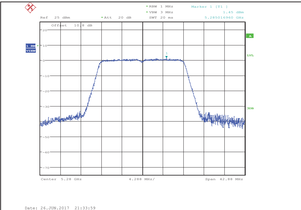
Maximum Power Spectral Density_TNVN_11N20MIMO_5280_Ant1+Ant2
