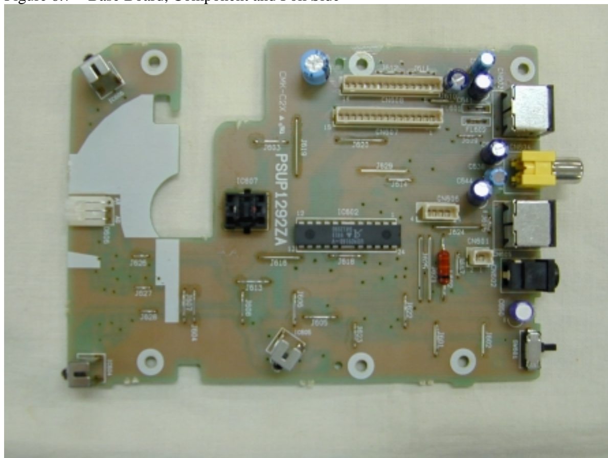
Figure 8.7 Base Board, Component and Foil Side
