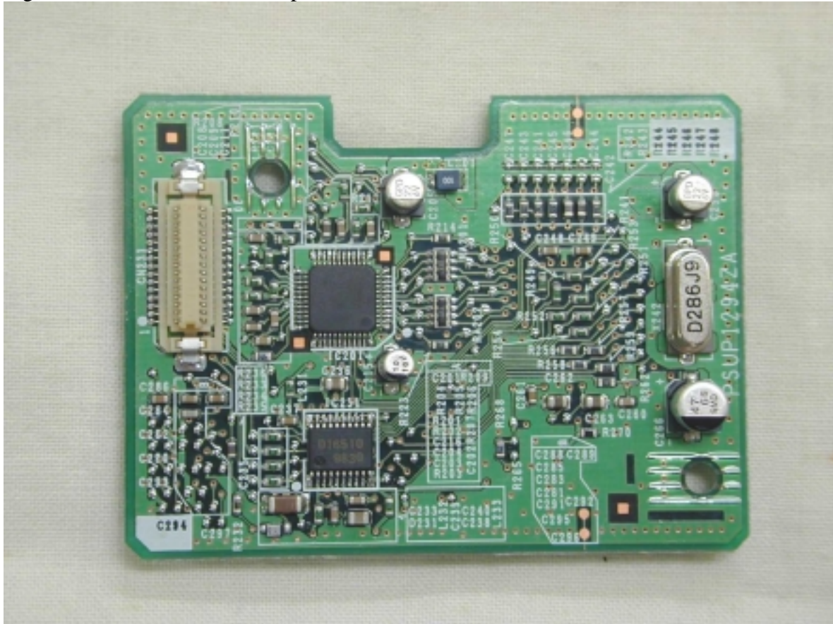
Figure 8.9 Video Board, Component and Foil Side
