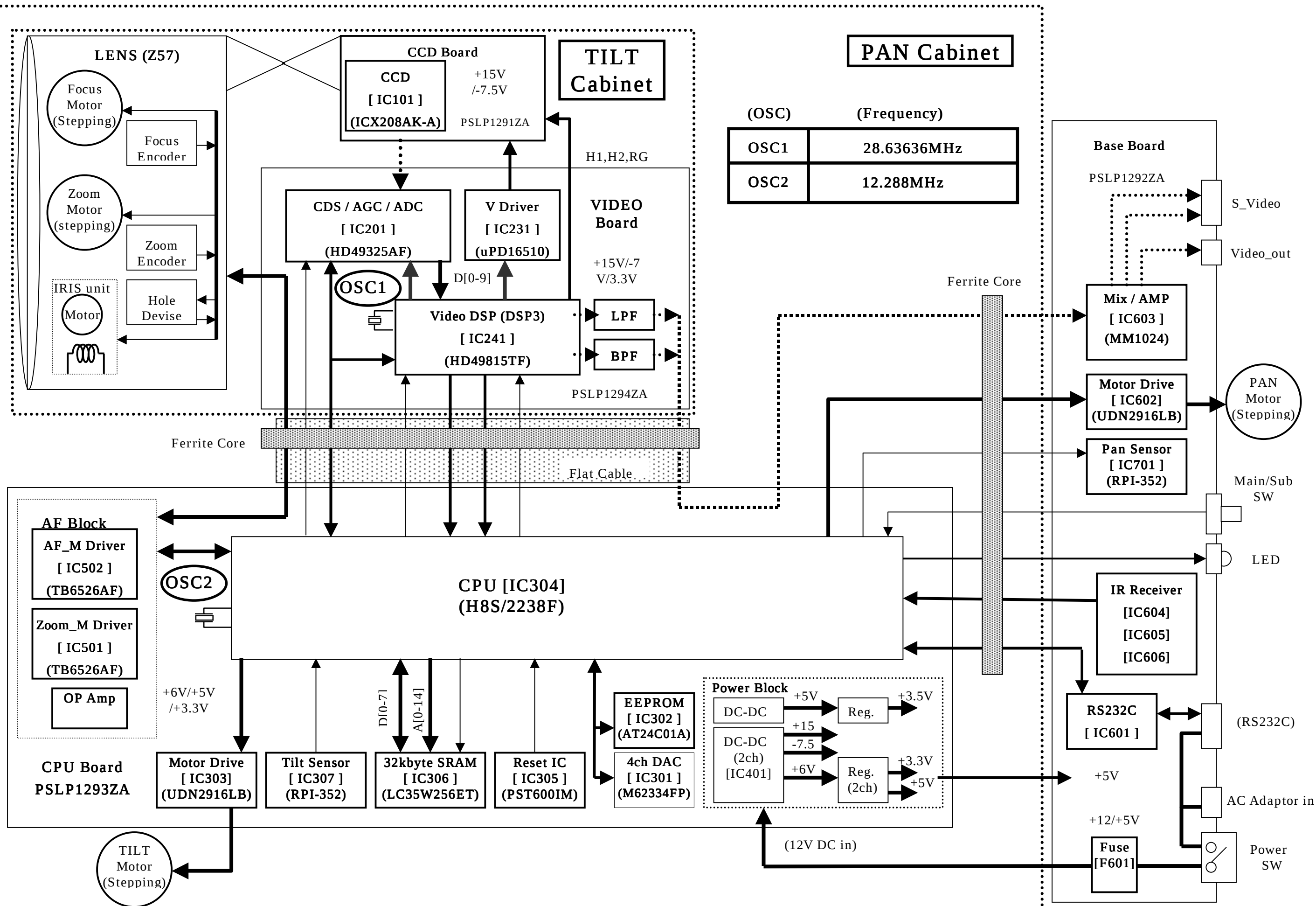
KX-DP702 Block Diagram
