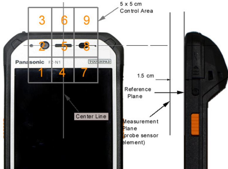
Figure 18-5 5x5 Scan grid above WD
