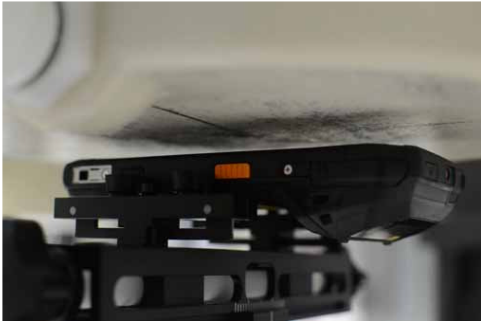
SAR Test Setup Photo 14 – Front Side at 1.0 cm with Standard Battery
