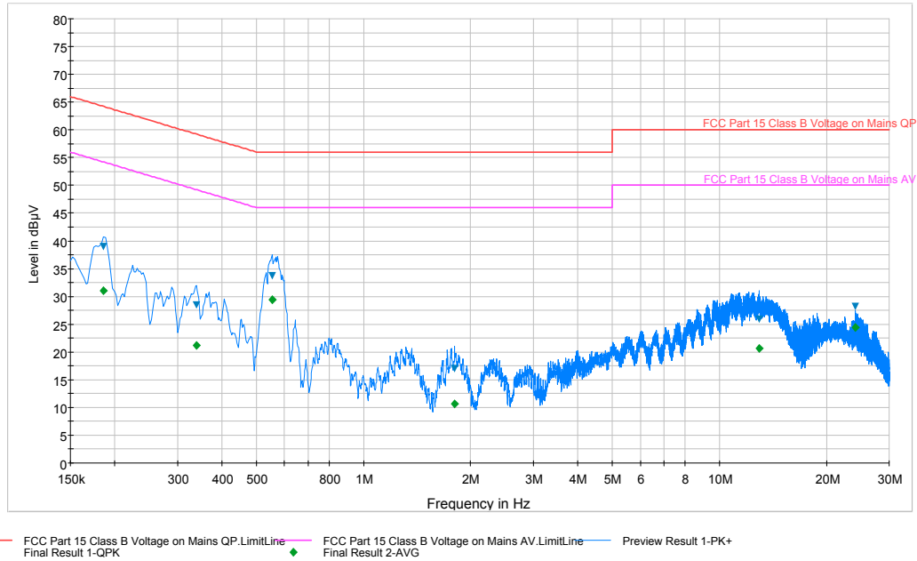
Plot 6-120. Line Conducted Plot with 802.11a UNII Band 3 (L1)
