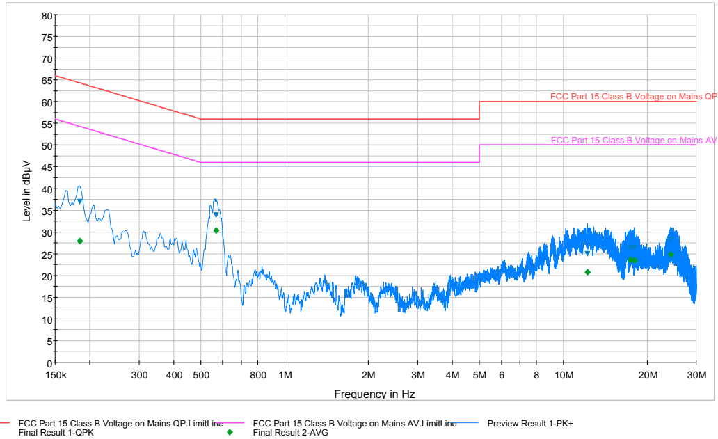
Plot 6-116. Line Conducted Plot with 802.11a UNII Band 2A (L1)
