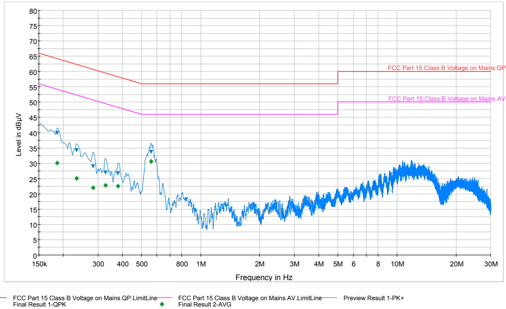
Plot 6-115. Line Conducted Plot with 802.11a UNII Band 1 (N)
