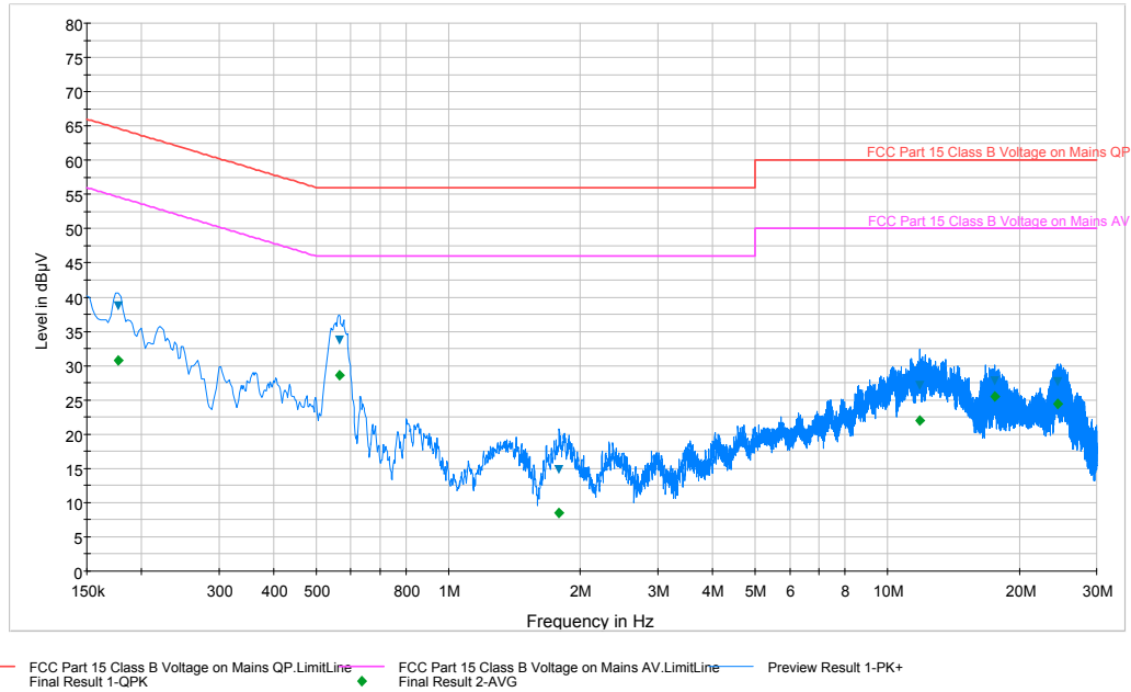
Plot 6-118. Line Conducted Plot with 802.11a UNII Band 2C (L1)
