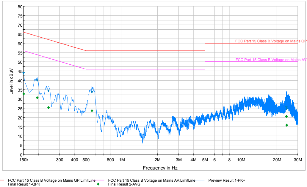
Plot 6-121. Line Conducted Plot with 802.11a UNII Band 3 (N)
