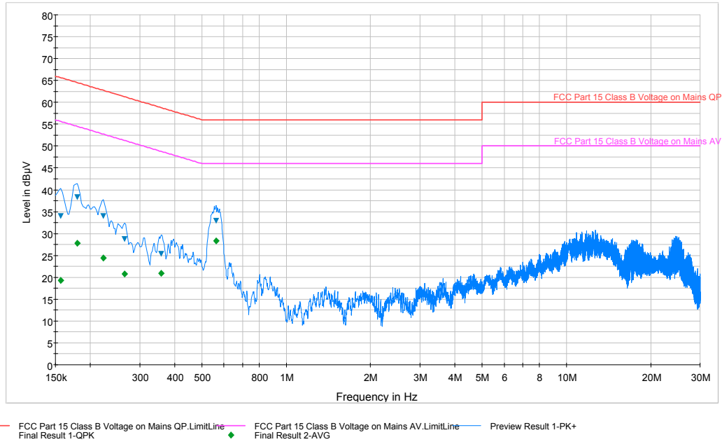
Plot 6-119. Line Conducted Plot with 802.11a UNII Band 2C (N)
