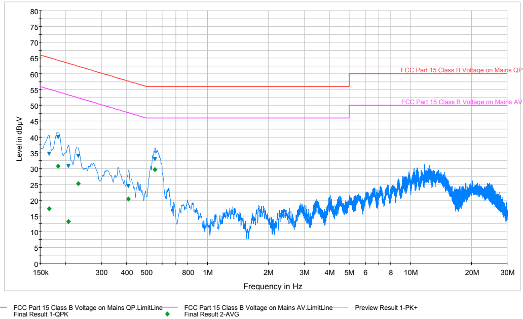
Plot 6-117. Line Conducted Plot with 802.11a UNII Band 2A (N)
