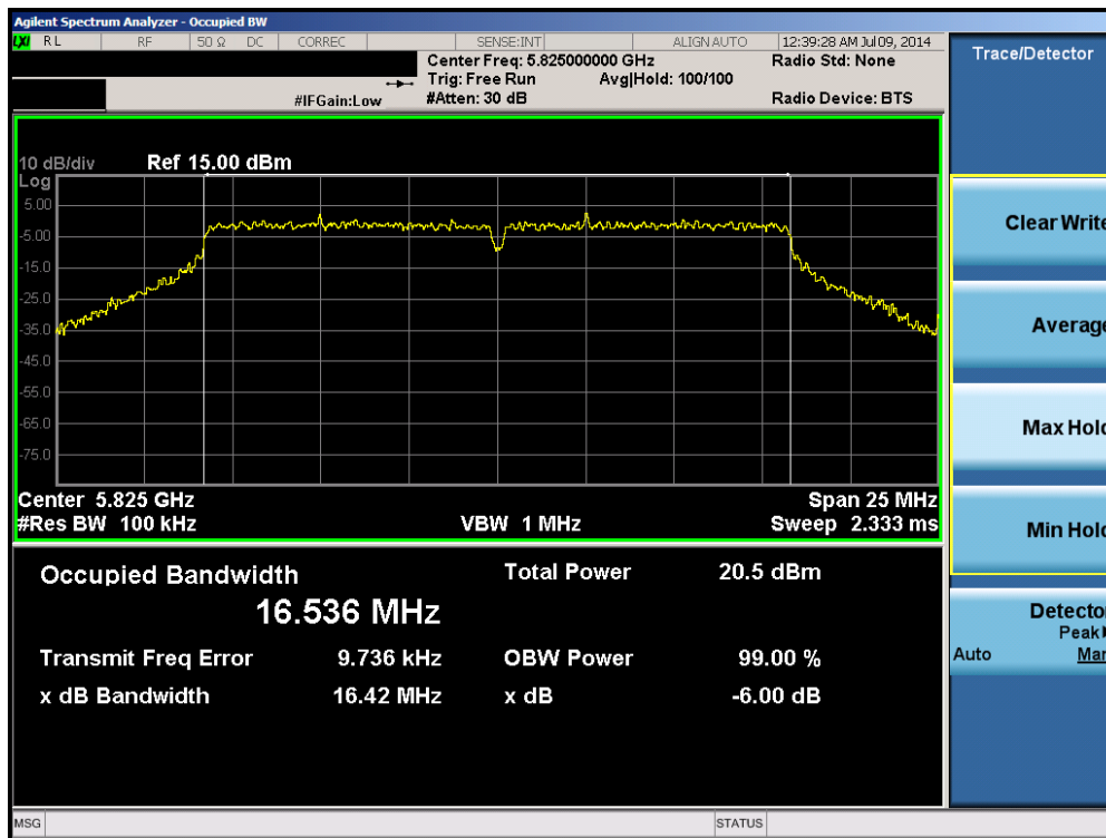
Plot 6-37. 26dB Bandwidth Plot (802.11a (UNII Band 3) – Ch. 165)
