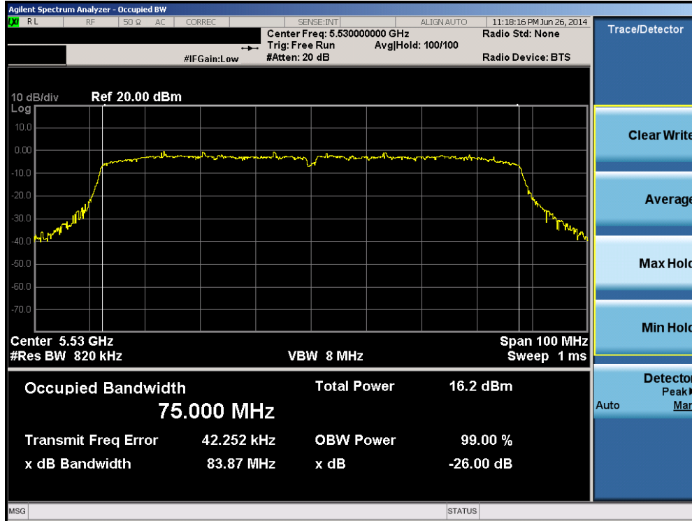
Plot 6-29. 26dB Bandwidth Plot (80MHz BW 802.11ac (UNII Band 2C) – Ch. 106
