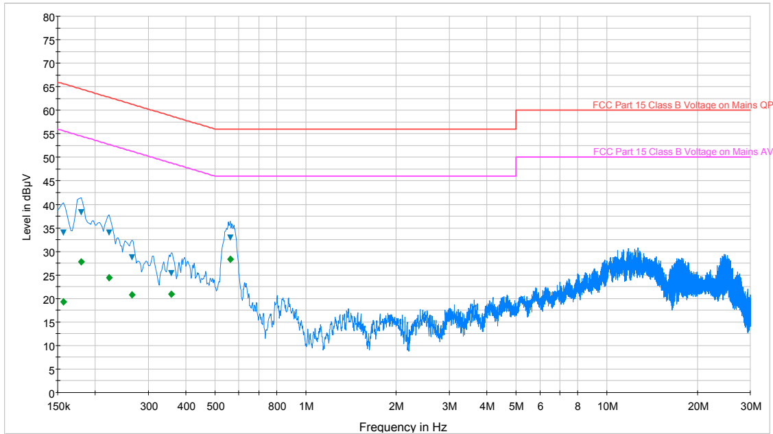
Plot 6-119. Line Conducted Plot with 802.11a UNII Band 2C (N)
