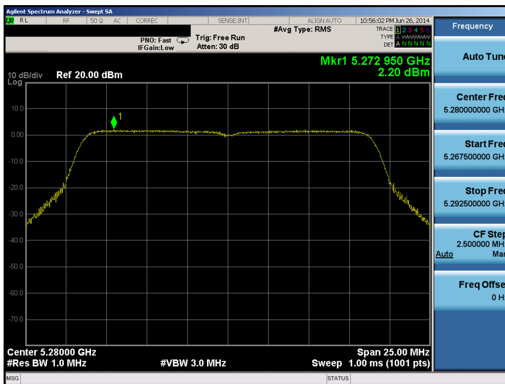
Plot 6-57. Peak Power Spectral Density Plot (20MHz BW 802.11n (UNII Band 2A) – Ch. 56)
