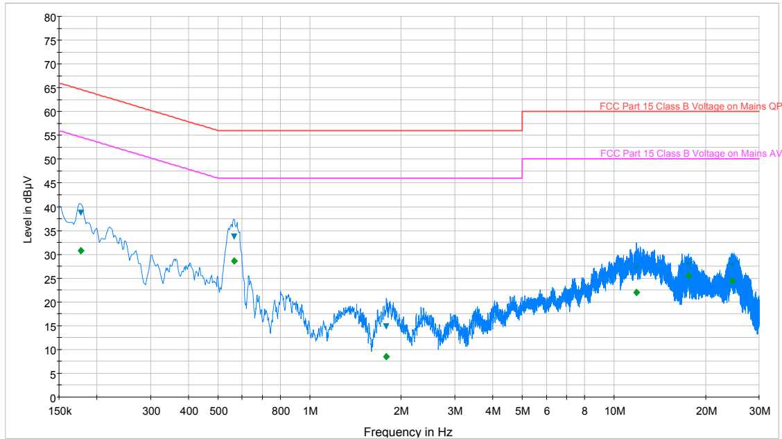
Plot 6-118. Line Conducted Plot with 802.11a UNII Band 2C (L1)
