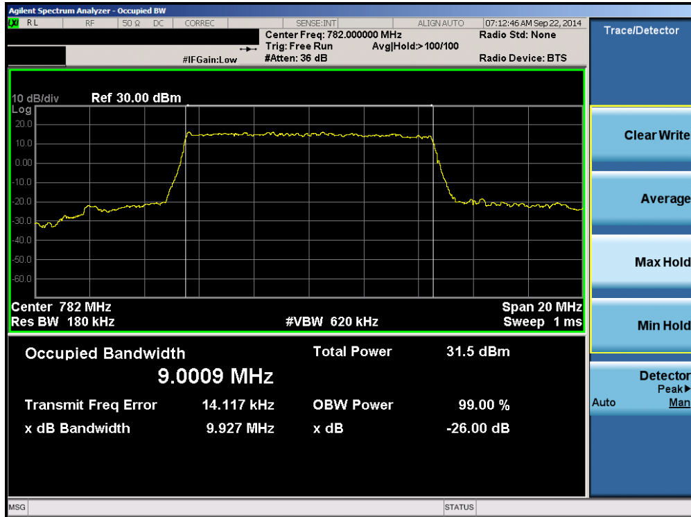
Plot 6-5. Occupied Bandwidth Plot (Band 13 – 10.0MHz QPSK – RB Size 50)
