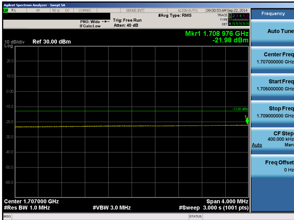
Plot 6-52. Lower Extended Band Edge Plot (Band 4 – 20.0MHz QPSK – RB Size 100)
