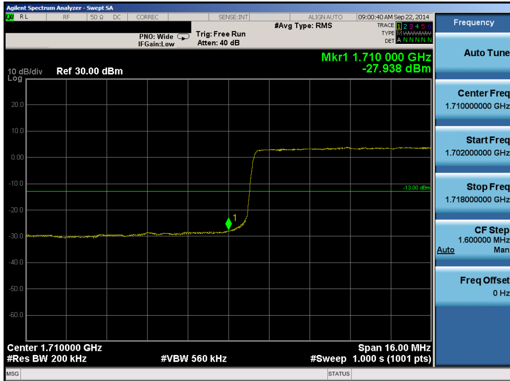
Plot 6-51. Lower Band Edge Plot (Band 4 – 20.0MHz QPSK – RB Size 100)
