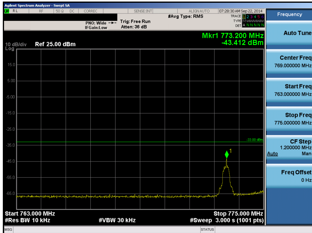
Plot 6-36. Lower Extended Band Edge Plot (Band 13 – 10.0MHz QPSK – RB Size 50)
