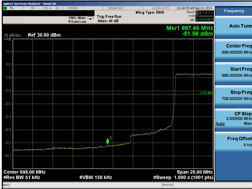
Plot 6-29. Lower Band Edge Plot (Band 17 – 5.0MHz QPSK – RB Size 25)
