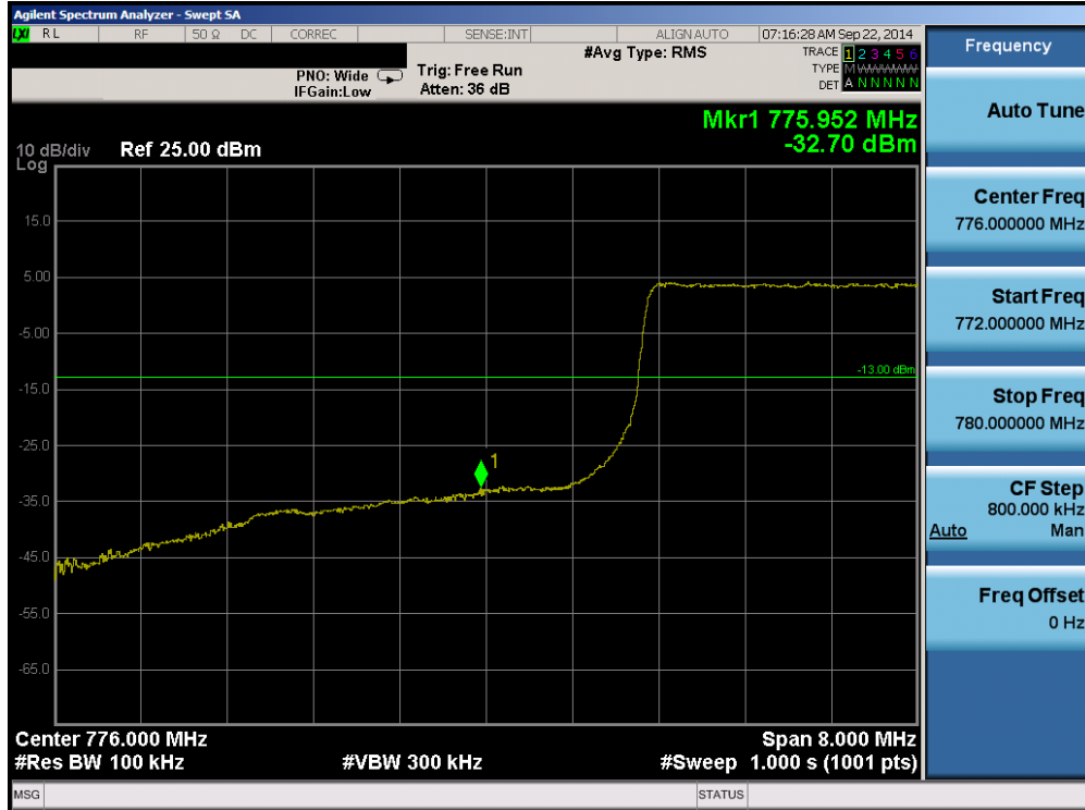
Plot 6-35. Lower Band Edge Plot (Band 13 – 10.0MHz QPSK – RB Size 50)
