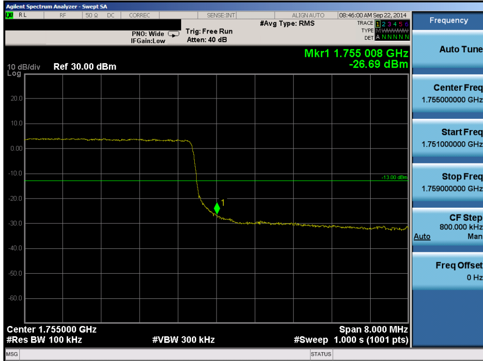
Plot 6-45. Upper Band Edge Plot (Band 4 – 10.0MHz QPSK – RB Size 50)
