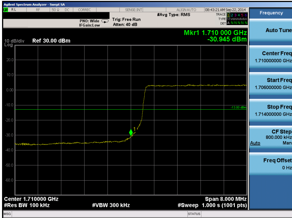
Plot 6-43. Lower Band Edge Plot (Band 4 – 10.0MHz QPSK – RB Size 50)
