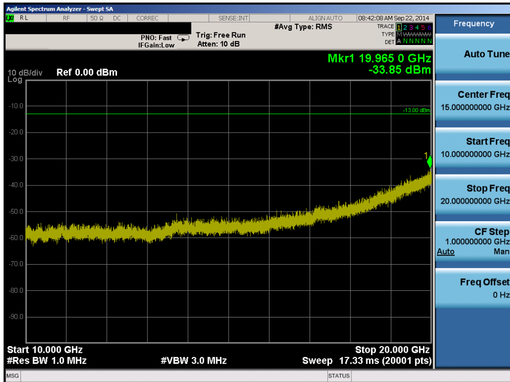
Plot 6-22. Conducted Spurious Plot (Band 4 – 10.0MHz QPSK – RB Size 1, RB Offset 0 – Low Channel)
