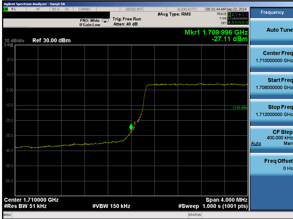
Plot 6-39. Lower Band Edge Plot (Band 4 – 5.0MHz QPSK – RB Size 25)
