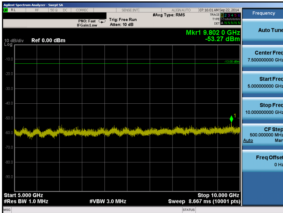
Plot 6-28. Conducted Spurious Plot (Band 13 – 10.0MHz QPSK – RB Size 1, RB Offset 0 – Mid Channel)
