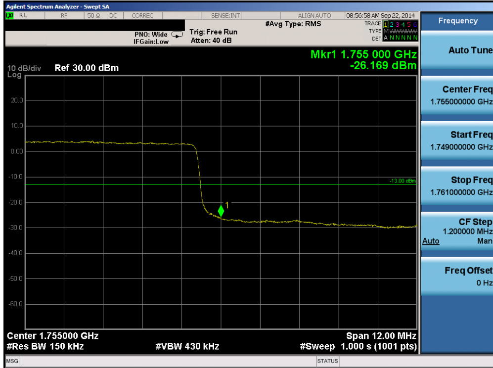
Plot 6-49. Upper Band Edge Plot (Band 4 – 15.0MHz QPSK – RB Size 75)
