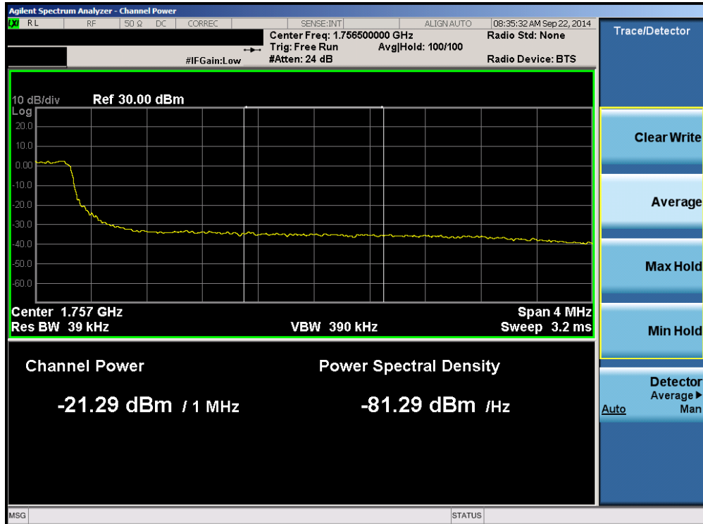
Plot 6-42. Upper Extended Band Edge Plot (Band 4 – 5.0MHz QPSK – RB Size 25)
