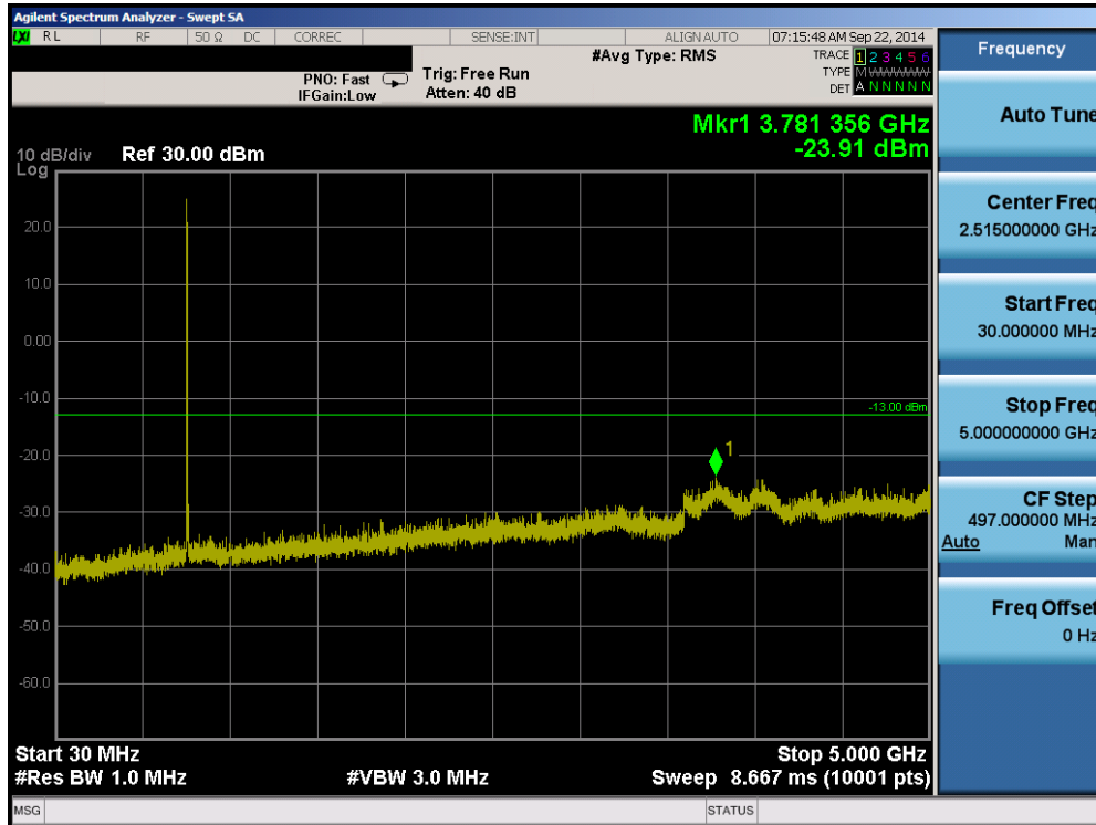
Plot 6-27. Conducted Spurious Plot (Band 13 – 10.0MHz QPSK – RB Size 1, RB Offset 0 – Mid Channel)
