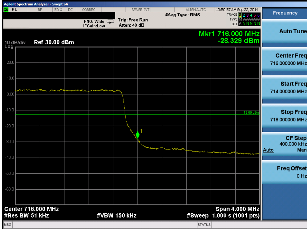
Plot 6-31. Upper Band Edge Plot (Band 17 – 5.0MHz QPSK – RB Size 25)
