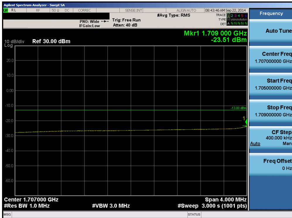
Plot 6-44. Lower Extended Band Edge Plot (Band 4 – 10.0MHz QPSK – RB Size 50)
