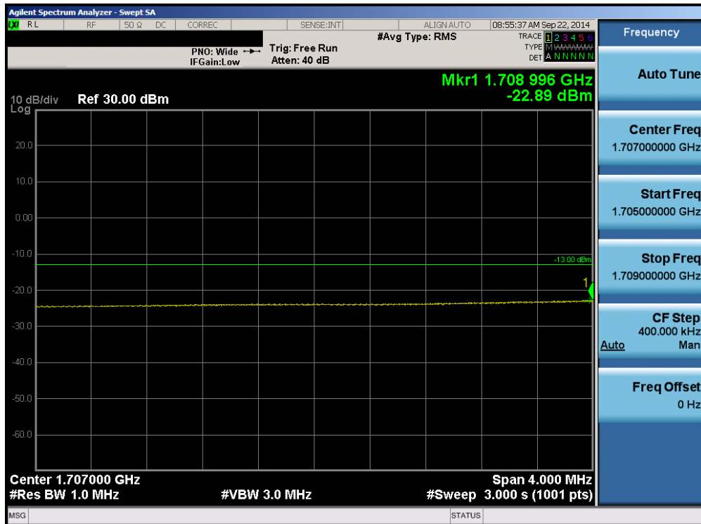
Plot 6-48. Lower Extended Band Edge Plot (Band 4 – 15.0MHz QPSK – RB Size 75)
