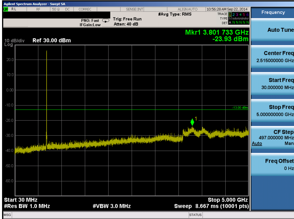
Plot 6-17. Conducted Spurious Plot (Band 17 – 10.0MHz QPSK – RB Size 1, RB Offset 0 – Mid Channel)
