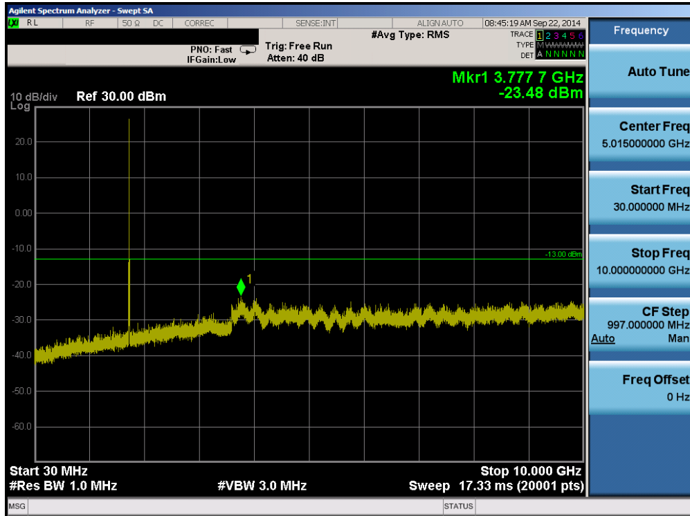
Plot 6-25. Conducted Spurious Plot (Band 4 – 10.0MHz QPSK – RB Size 1, RB Offset 0 – High Channel)
