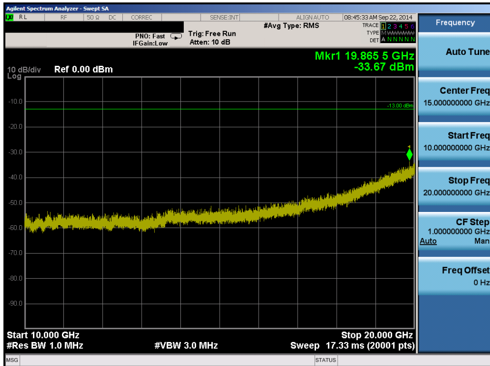
Plot 6-26. Conducted Spurious Plot (Band 4 – 10.0MHz QPSK – RB Size 1, RB Offset 0 – High Channel)
