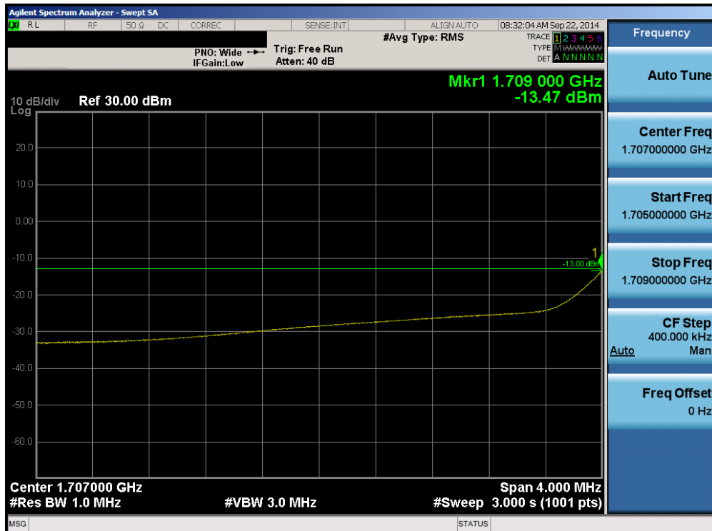
Plot 6-40. Lower Extended Band Edge Plot (Band 4 – 5.0MHz QPSK – RB Size 25)
