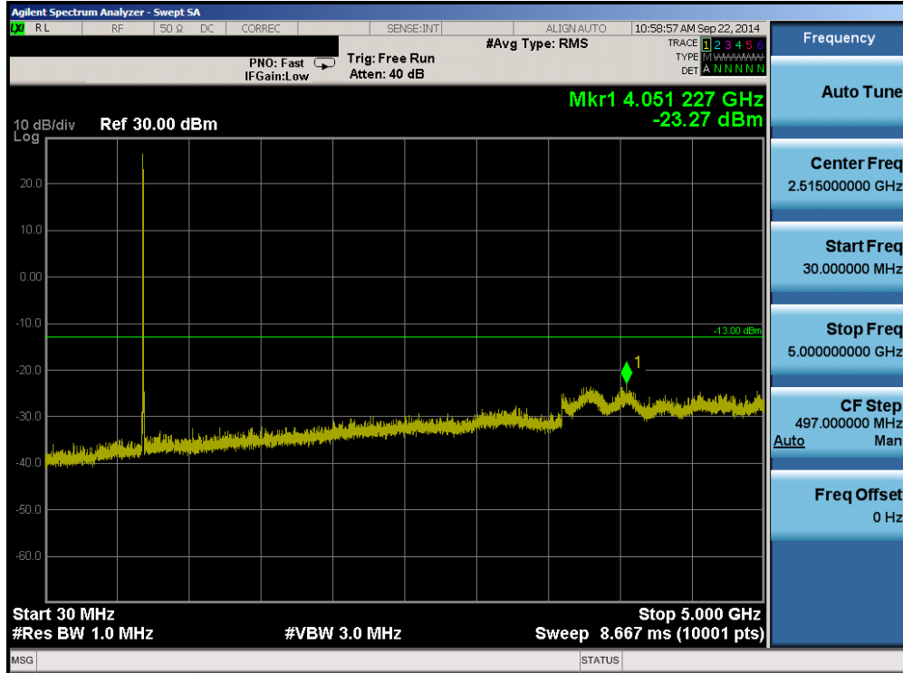
Plot 6-15. Conducted Spurious Plot (Band 17 – 10.0MHz QPSK – RB Size 1, RB Offset 0– Low Channel)
