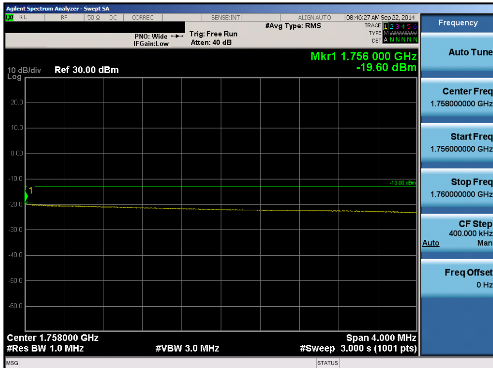
Plot 6-46. Upper Extended Band Edge Plot (Band 4 – 10.0MHz QPSK – RB Size 50)
