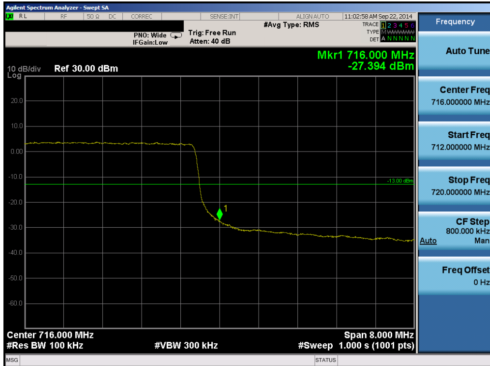
Plot 6-34. Upper Band Edge Plot (Band 17 – 10.0MHz QPSK – RB Size 50)
