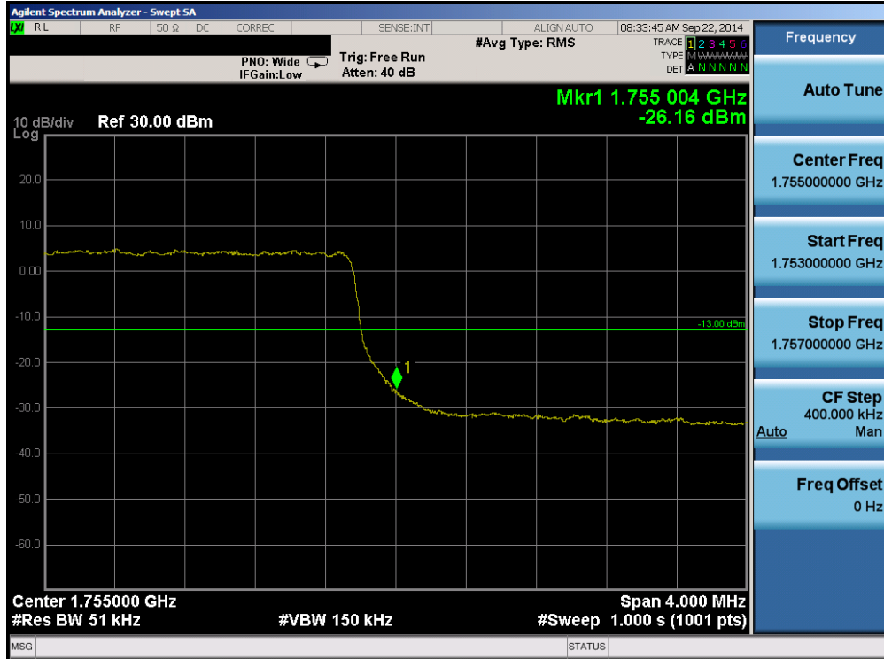
Plot 6-41. Upper Band Edge Plot (Band 4 – 5.0MHz QPSK – RB Size 25)
