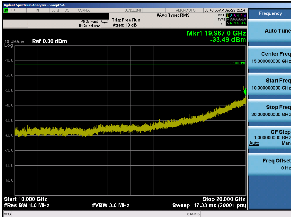
Plot 6-24. Conducted Spurious Plot (Band 4 – 10.0MHz QPSK – RB Size 1, RB Offset 0 – Mid Channel)
