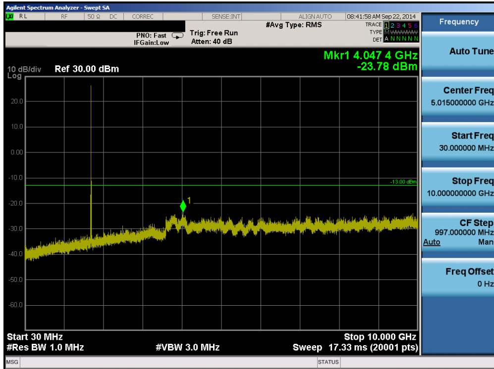
Plot 6-21. Conducted Spurious Plot (Band 4 – 10.0MHz QPSK – RB Size 1, RB Offset 0– Low Channel)
