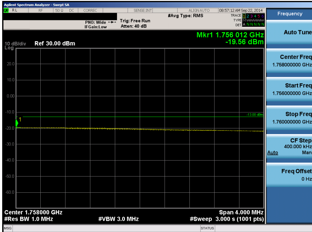
Plot 6-50. Upper Extended Band Edge Plot (Band 4 – 15.0MHz QPSK – RB Size 75)
