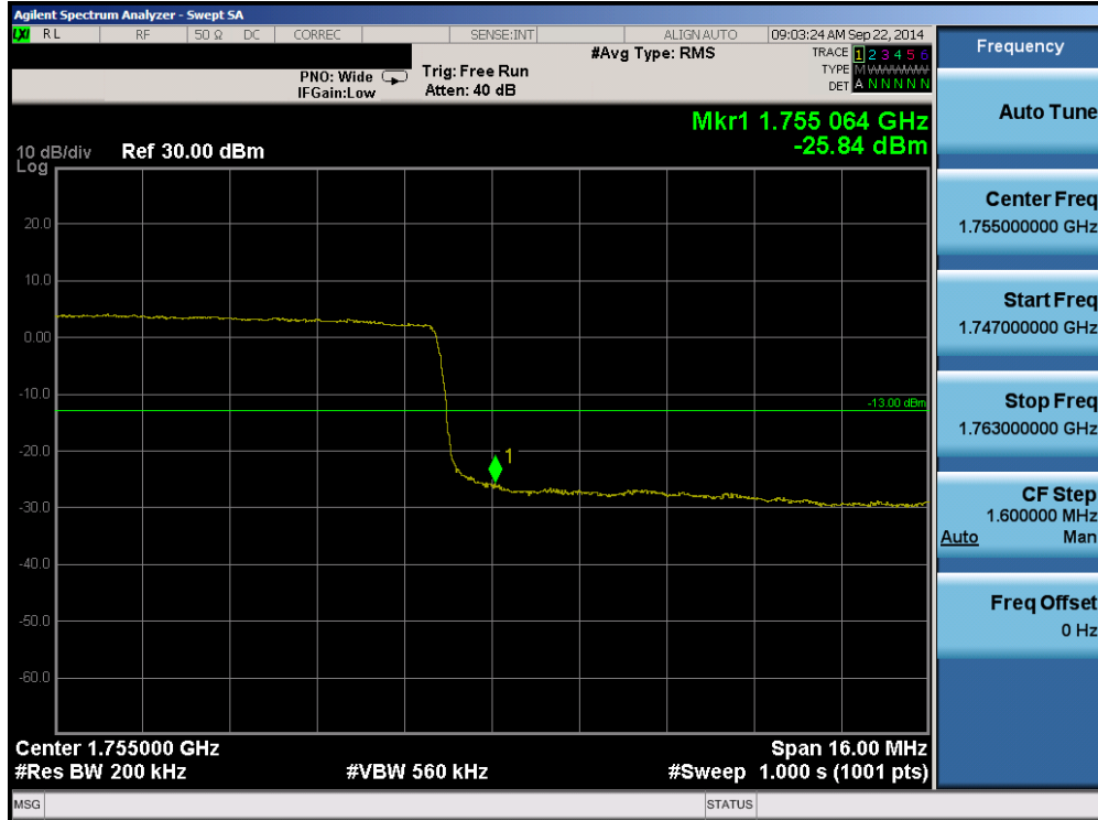
Plot 6-53. Upper Band Edge Plot (Band 4 – 20.0MHz QPSK – RB Size 100)
