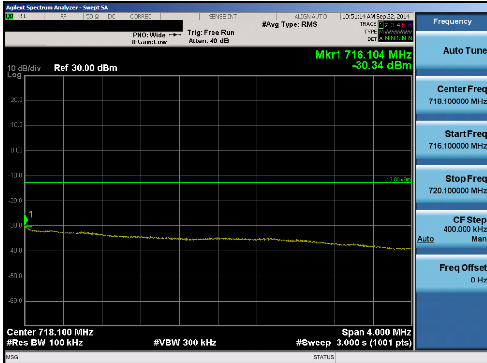
Plot 6-32. Upper Extended Band Edge Plot (Band 17 – 5.0MHz QPSK – RB Size 25)
