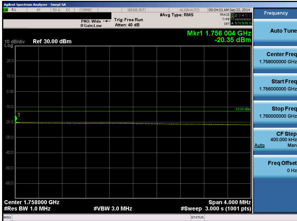
Plot 6-54. Upper Extended Band Edge Plot (Band 4 – 20.0MHz QPSK – RB Size 100)
