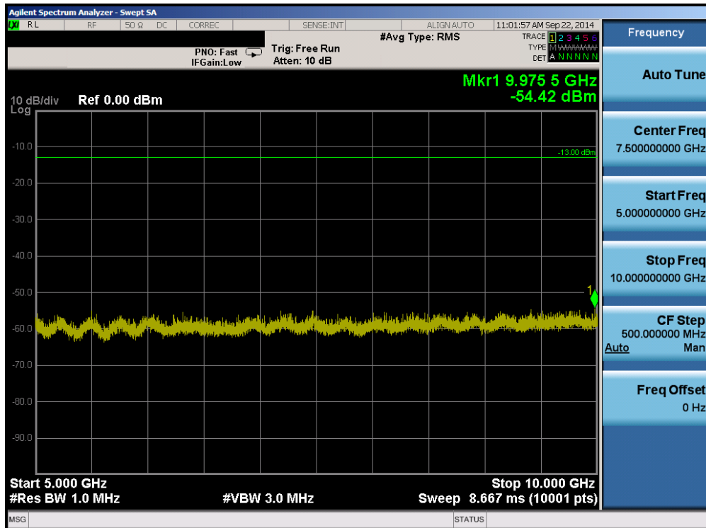
Plot 6-20. Conducted Spurious Plot (Band 17 – 10.0MHz QPSK – RB Size 1, RB Offset 0 – High Channel)
