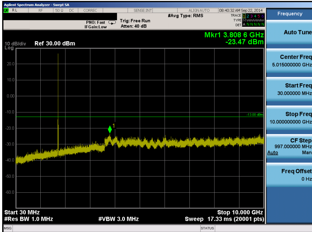
Plot 6-23. Conducted Spurious Plot (Band 4 – 10.0MHz QPSK – RB Size 1, RB Offset 0 – Mid Channel)
