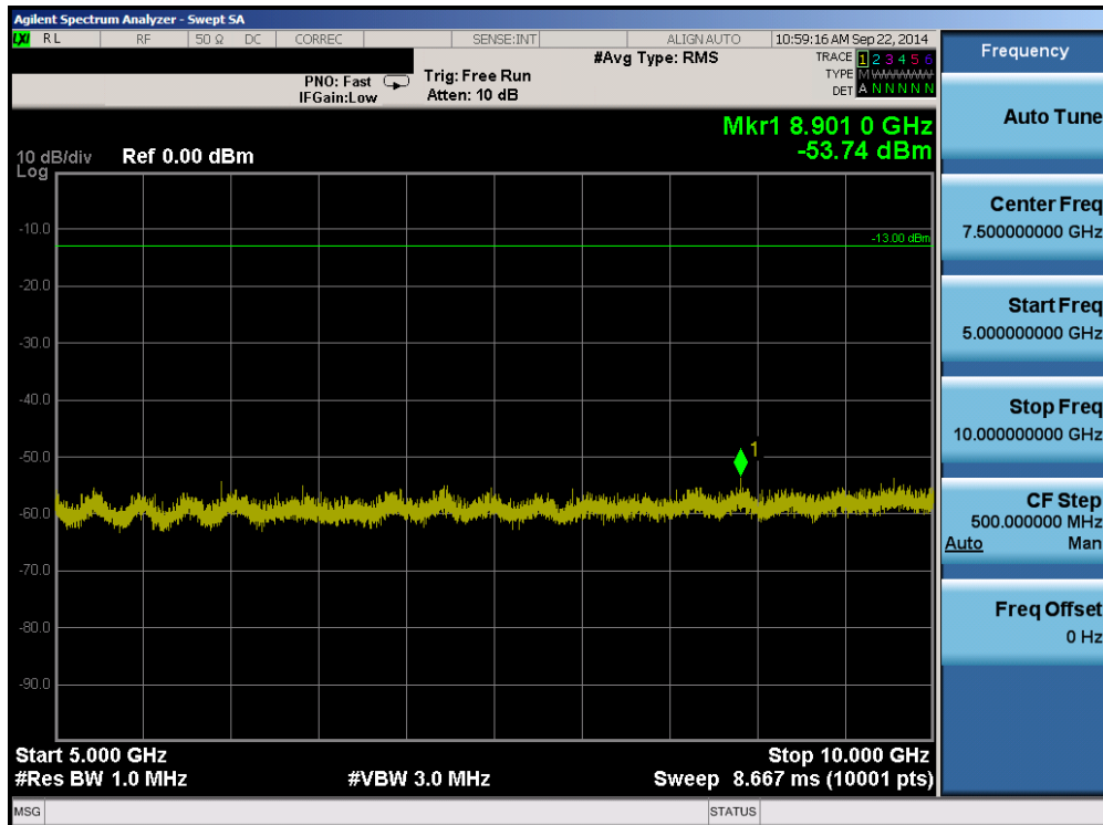
Plot 6-16. Conducted Spurious Plot (Band 17 – 10.0MHz QPSK – RB Size 1, RB Offset 0 – Low Channel)
