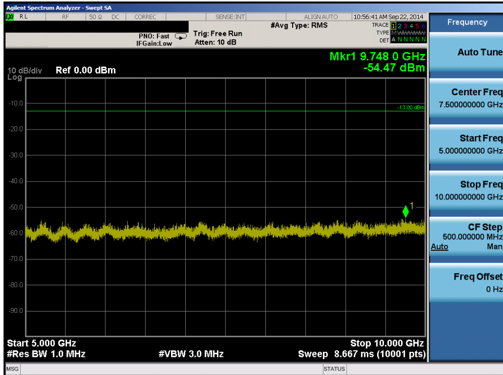
Plot 6-18. Conducted Spurious Plot (Band 17 – 10.0MHz QPSK – RB Size 1, RB Offset 0 – Mid Channel)
