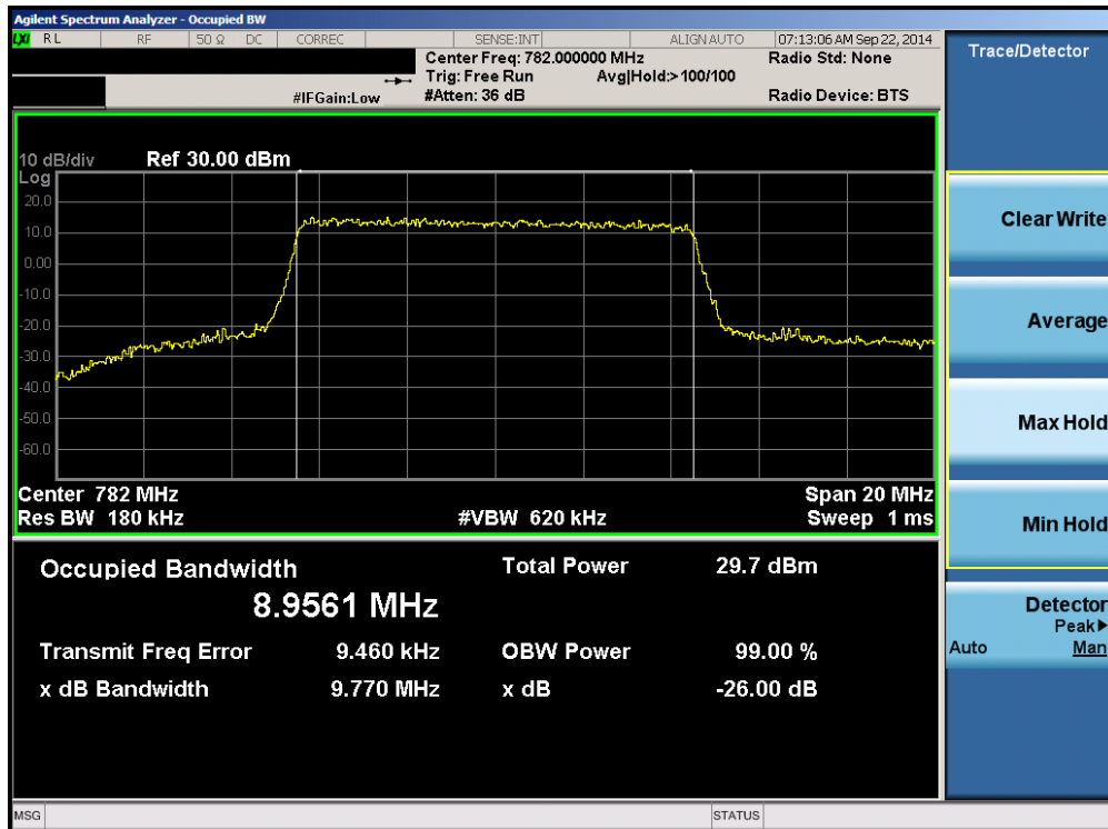
Plot 6-6. Occupied Bandwidth Plot (Band 13 – 10.0MHz 16-QAM – RB Size 50)
