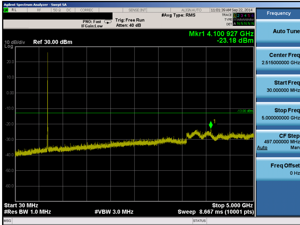
Plot 6-19. Conducted Spurious Plot (Band 17 – 10.0MHz QPSK – RB Size 1, RB Offset 0 – High Channel)
