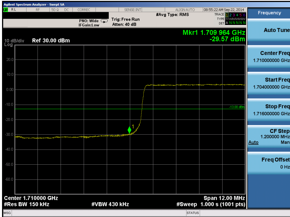
Plot 6-47. Lower Band Edge Plot (Band 4 – 15.0MHz QPSK – RB Size 75)
