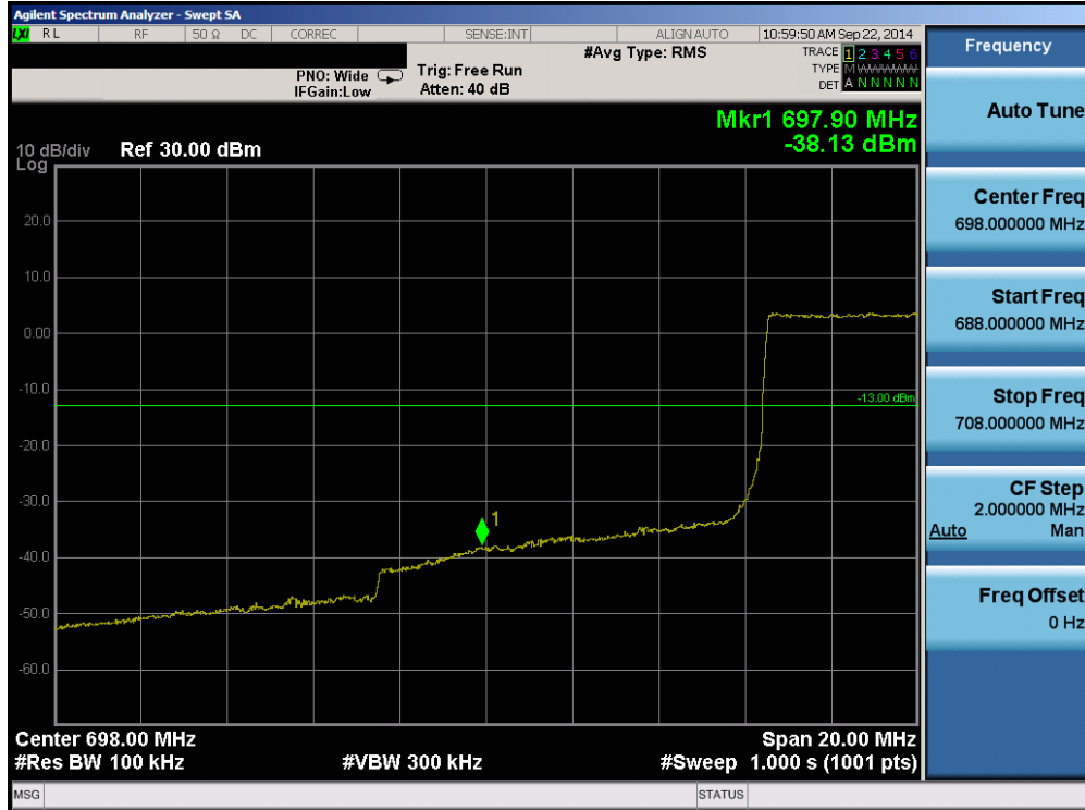
Plot 6-33. Lower Band Edge Plot (Band 17 – 10.0MHz QPSK – RB Size 50)
