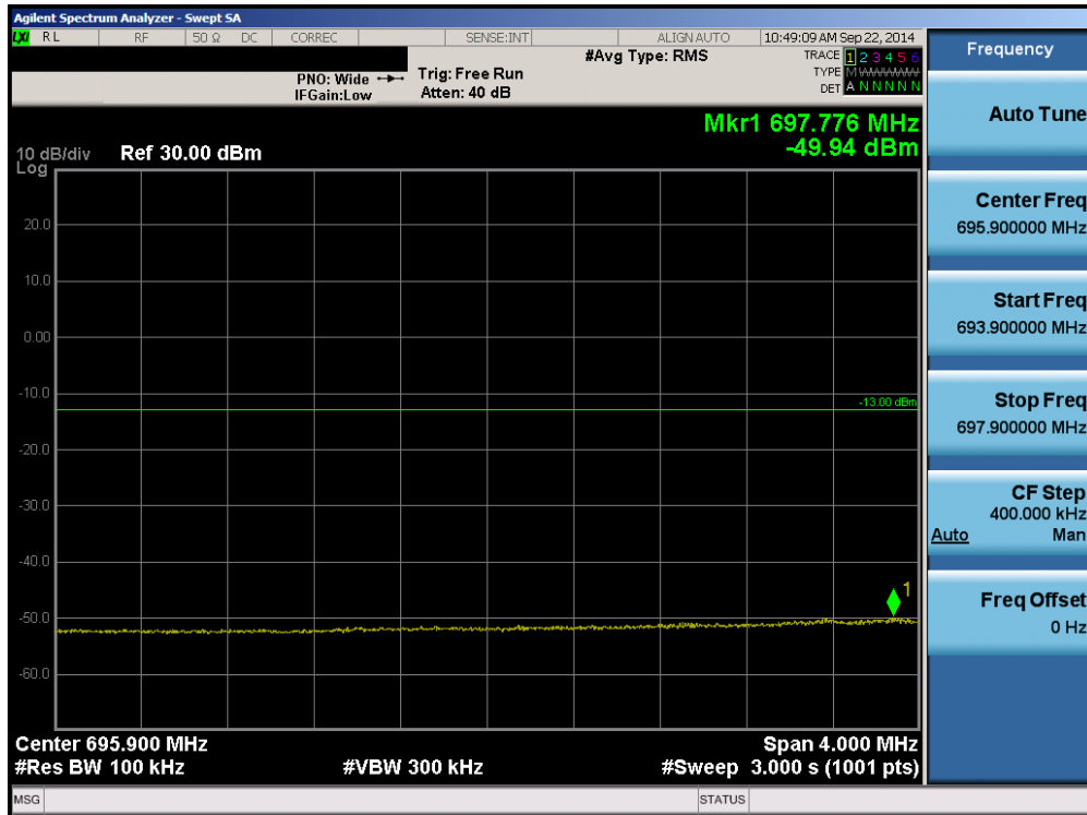
Plot 6-30. Lower Extended Band Edge Plot (Band 17 – 5.0MHz QPSK – RB Size 25)
