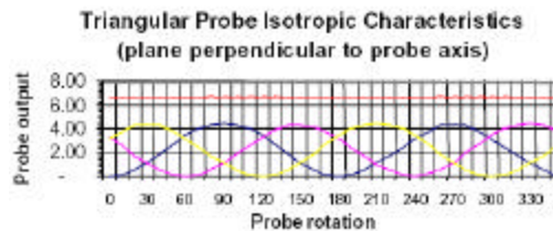
Figure 3.3 Probe Characteristics
