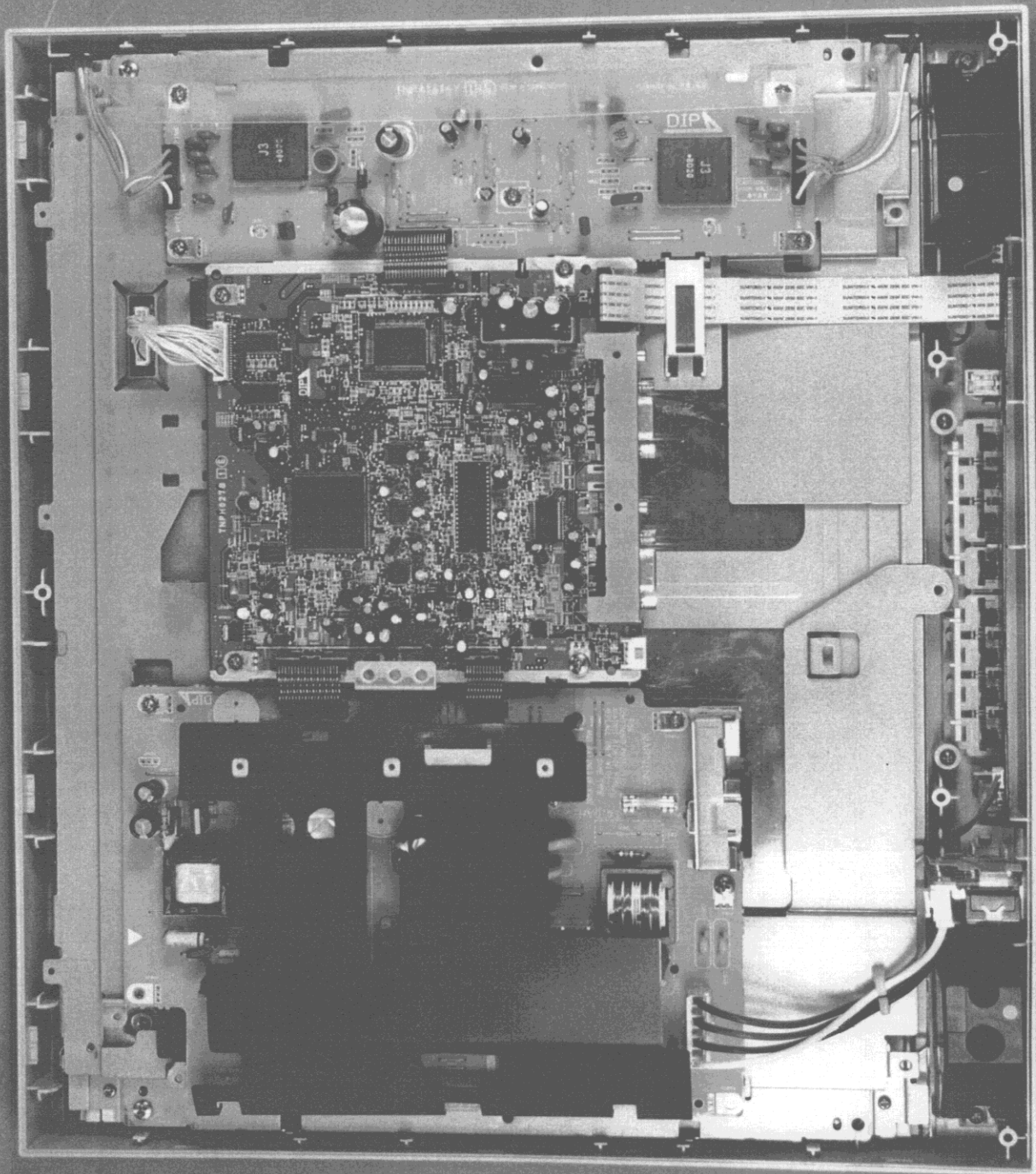
Fig. 5 Inside view of TX-D9L51NMF without shield cover
