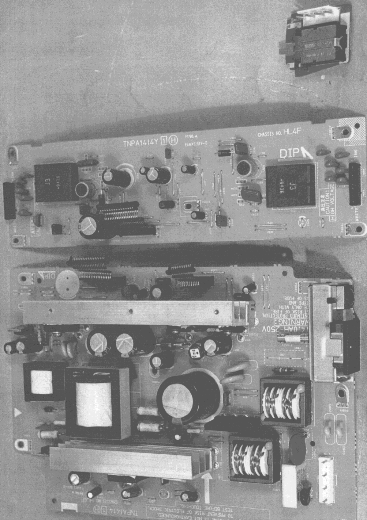
Fig. 6 Power Supply, AC Switch & Inverter PCB of TX-D9L51NMF
