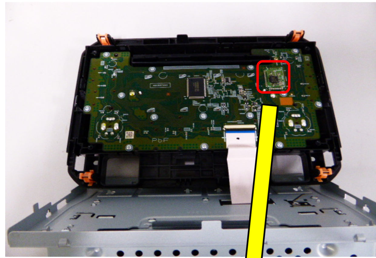
BT PCB
