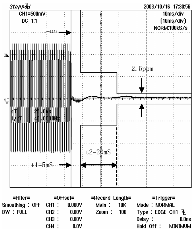
Figure 6I-1: 5 Watts, 12.5 KHz Key-Up Attack Time
