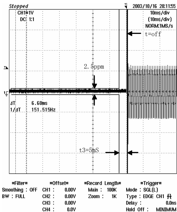
Figure 6I-2: 5 Watts, 12.5 KHz De-Key Decay Time
