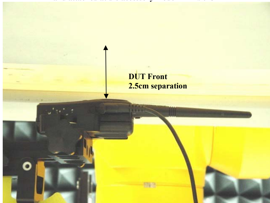
Figure 5: Assessment @ the Body; DUT front towards the phantom separated 2.5cm, with antenna model PMAD4015A and attached audio accessory model HMN9013A
