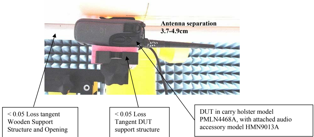
Figure 1: Highest S.A.R. Test Position DUT with carry holster model PMLN4468A against the flat phantom, antenna model PMAD4015A, and attached audio accessory HMN9013A
