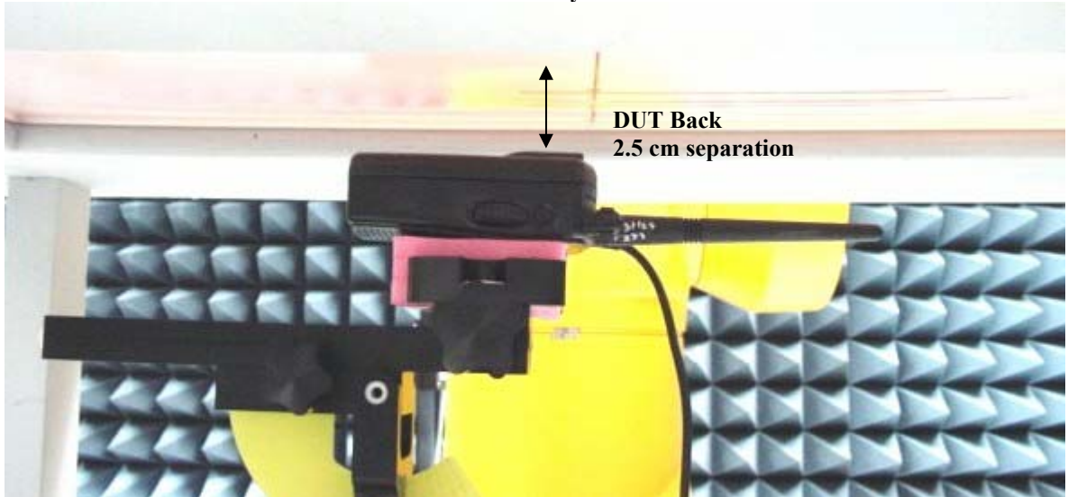
Figure 6: Assessment @ the Body; DUT back towards the phantom and separated 2.5cm, with antenna model PMAD4015A, and attached audio accessory model HMN9013A
