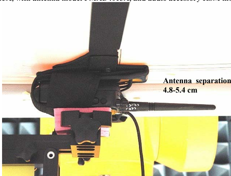
Figure 3. Assessment @ the body; DUT w/ carry case accessory model RLN4815A, with antenna model PMAD4015A, and audio accessory RSM model HMN9030A
