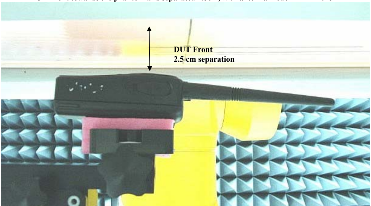
Figure 7: Assessment @ the Face; DUT Front towards the phantom and separated 2.5cm, with antenna model PMAD4015A
