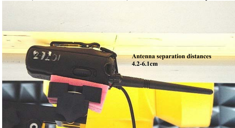
Figure 5: Assessment @ the Body; DUT front towards the phantom separated 2.5cm, with antenna model PMAD4015A and attached audio accessory model HMN9013A
