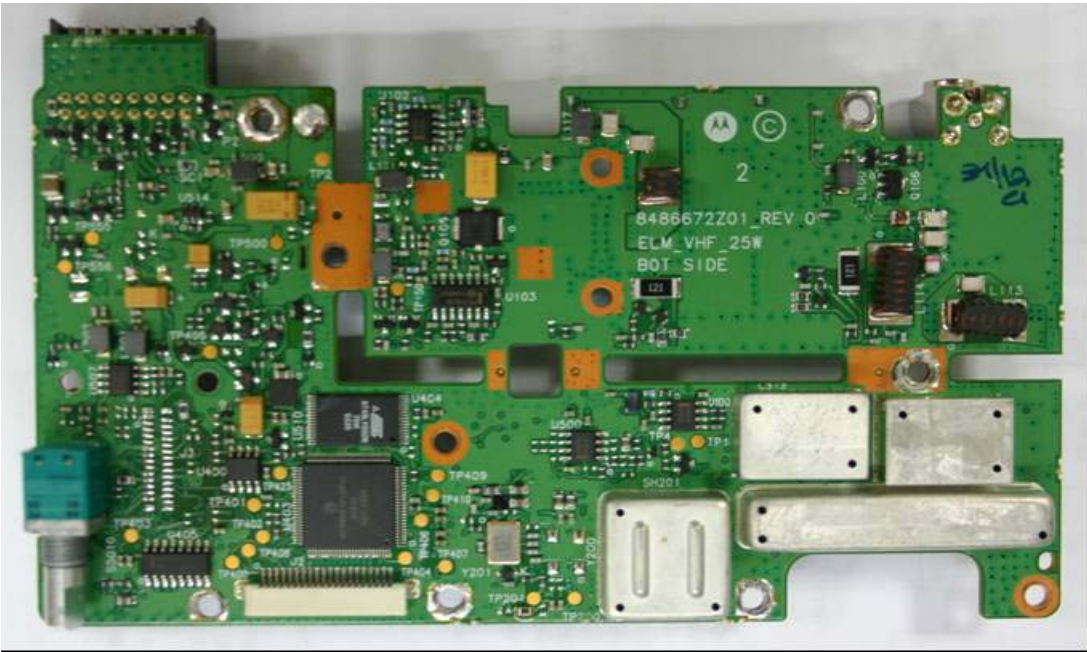
Figure 9-4: Bottom Side of PCB with shields.
