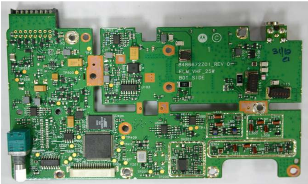
Figure 9-2: Bottom Side of PCB without shields.
