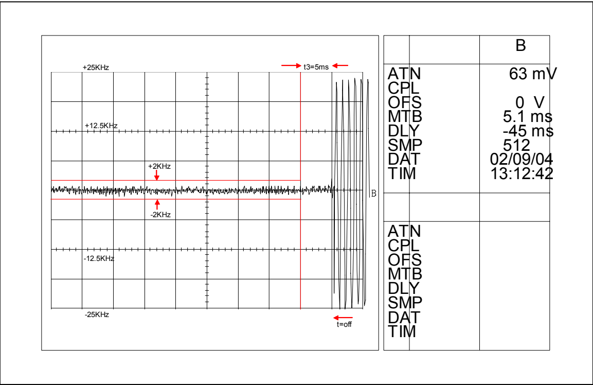
Figure 6I-8: 1 Watts, 25 KHz De-Key Decay Time
