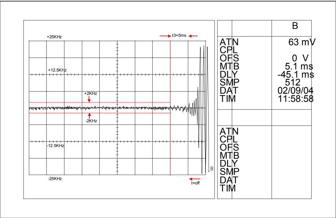
Figure 6I-4: 25 Watts, 25 KHz De-Key Decay Time
