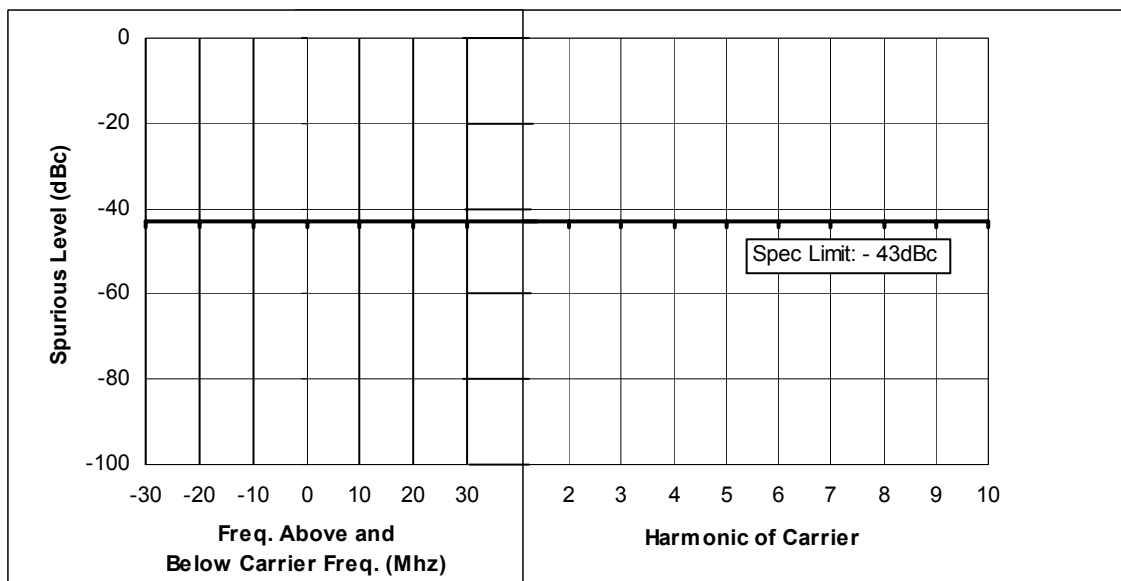
Figure 6F-12: 1 Watts, 161.75 MHz, 25 KHz Channel Spacing
