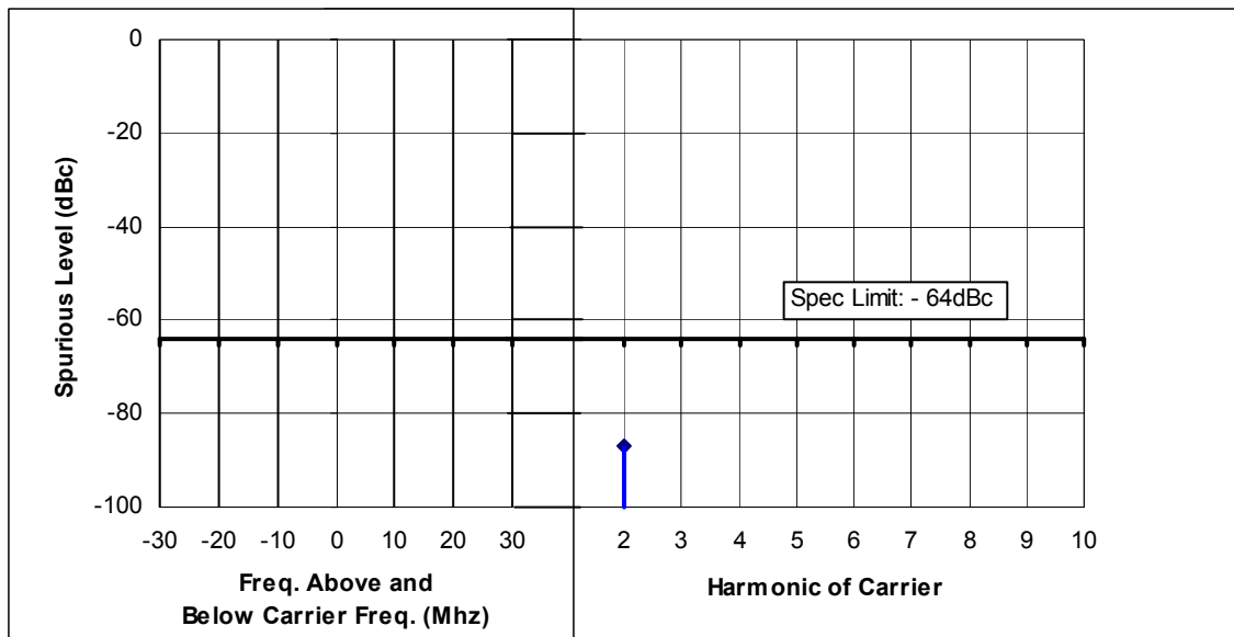
Figure 6F-2: 25 Watts, 149.00 MHz, 12.5 KHz Channel Spacing
