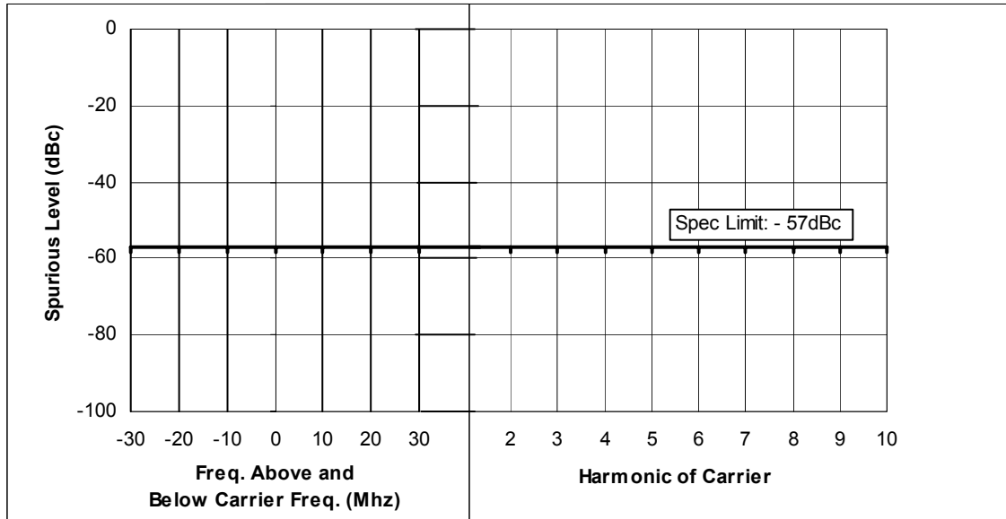
Figure 6F-6: 25 Watts, 161.75 MHz, 25 KHz Channel Spacing
