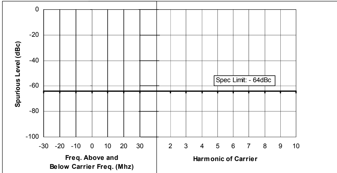
Figure 6F-1: 25 Watts, 136.25 MHz, 12.5 KHz Channel Spacing
