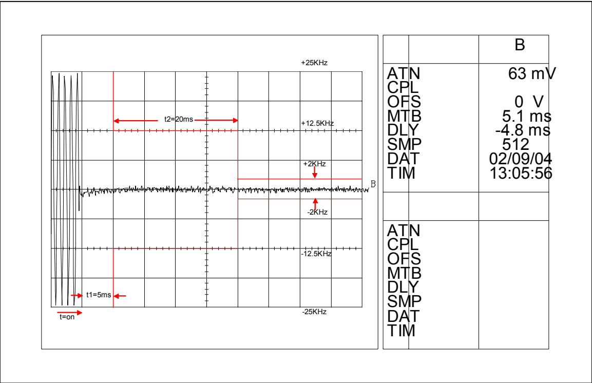
Figure 6I-1: 25 Watts, 12.5 KHz Key-Up Attack Time
