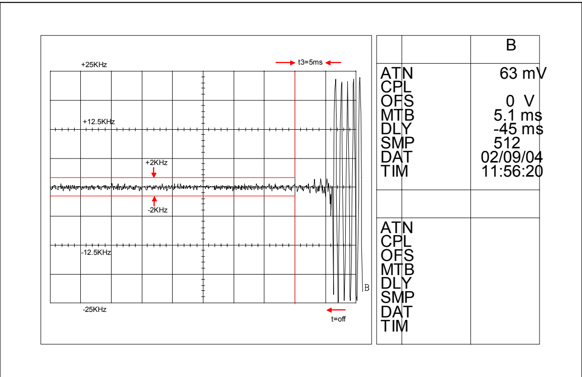
Figure 6I-2: 25 Watts, 12.5 KHz De-Key Decay Time
