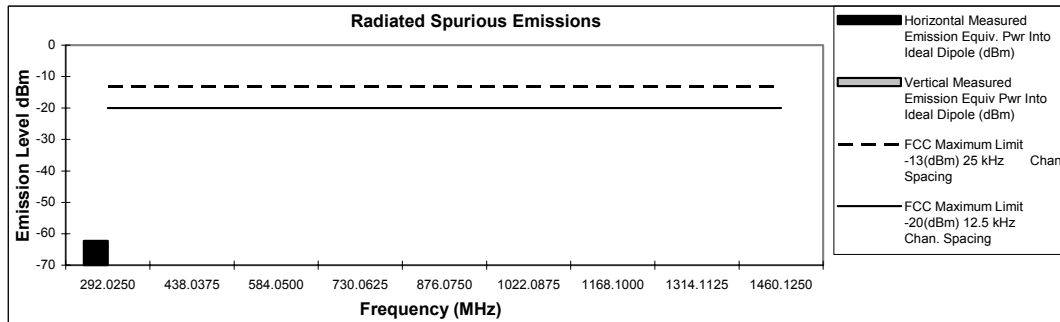
Figure 6G-5 – 1 Watts, 146.0125 MHz
