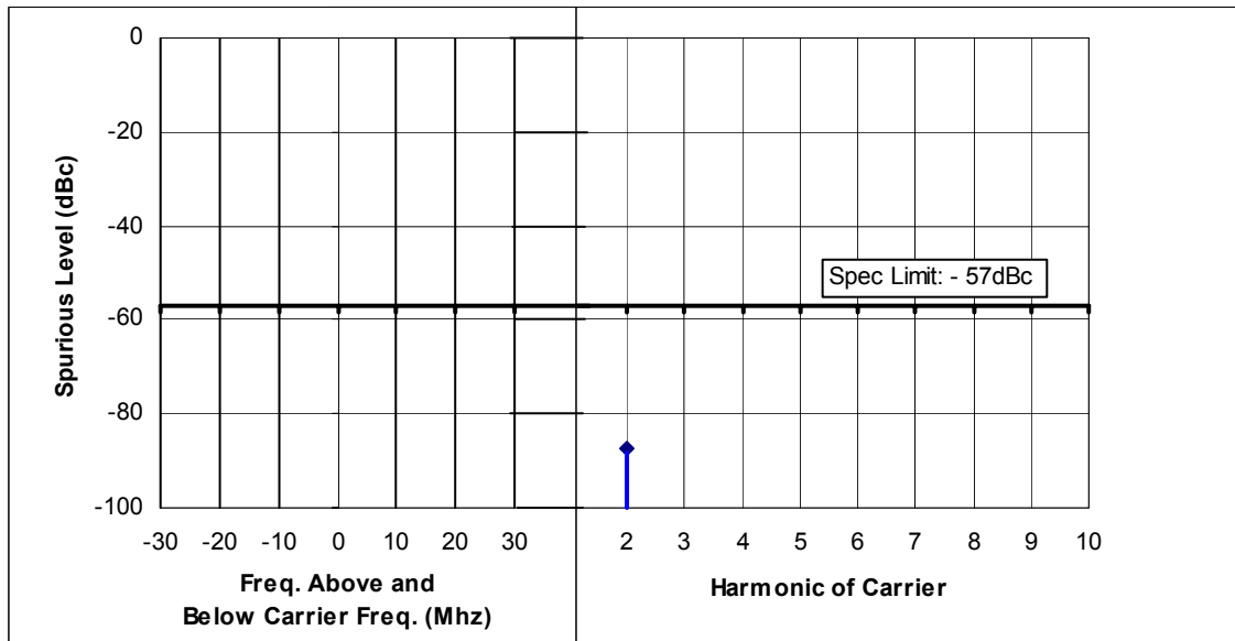
Figure 6F-5: 25 Watts, 149.00 MHz, 25 KHz Channel Spacing
