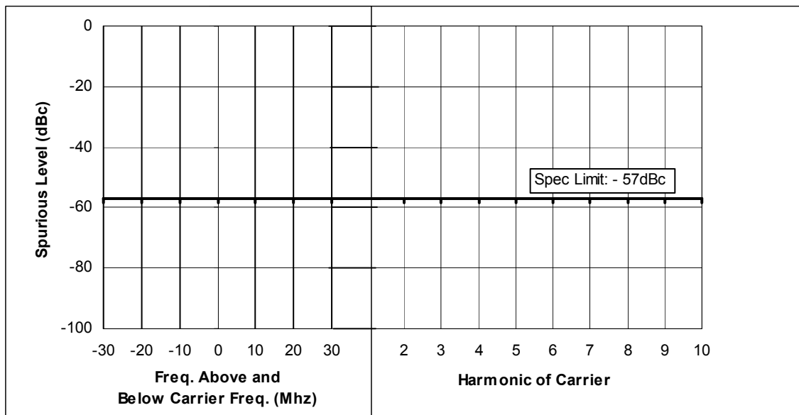
Figure 6F-4: 25 Watts, 136.25 MHz, 25 KHz Channel Spacing
