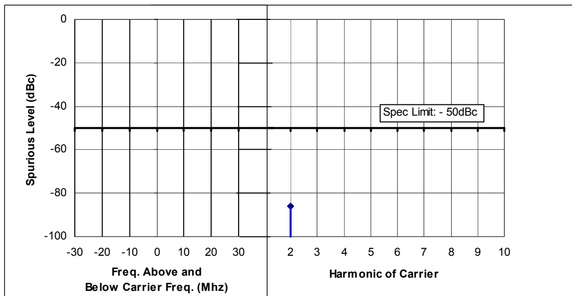
Figure 6F-8: 1 Watts, 149.00 MHz, 12.5 KHz Channel Spacing
