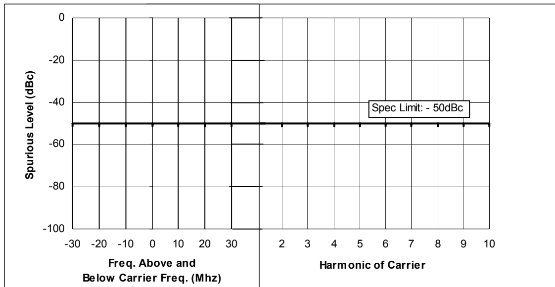
Figure 6F-7: 1 Watts, 136.25 MHz, 12.5 KHz Channel Spacing
