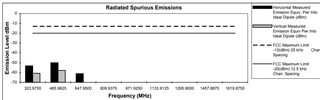
* Figure 6G-3 – 28 Watts, 161.9875 MHz
