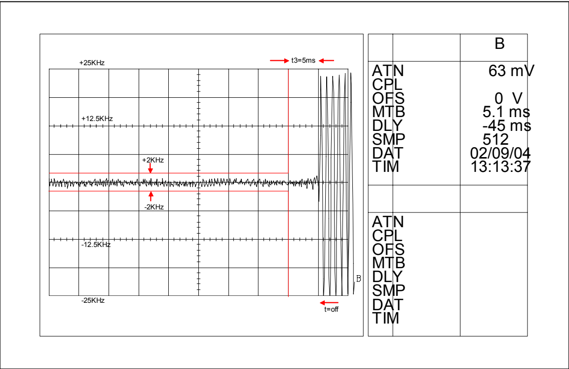
Figure 6I-6: 1 Watts, 12.5 KHz De-Key Decay Time
