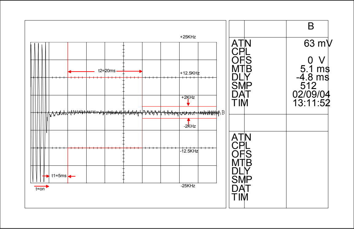
Figure 6I-7: 1 Watts, 25 KHz Key-Up Attack Time
