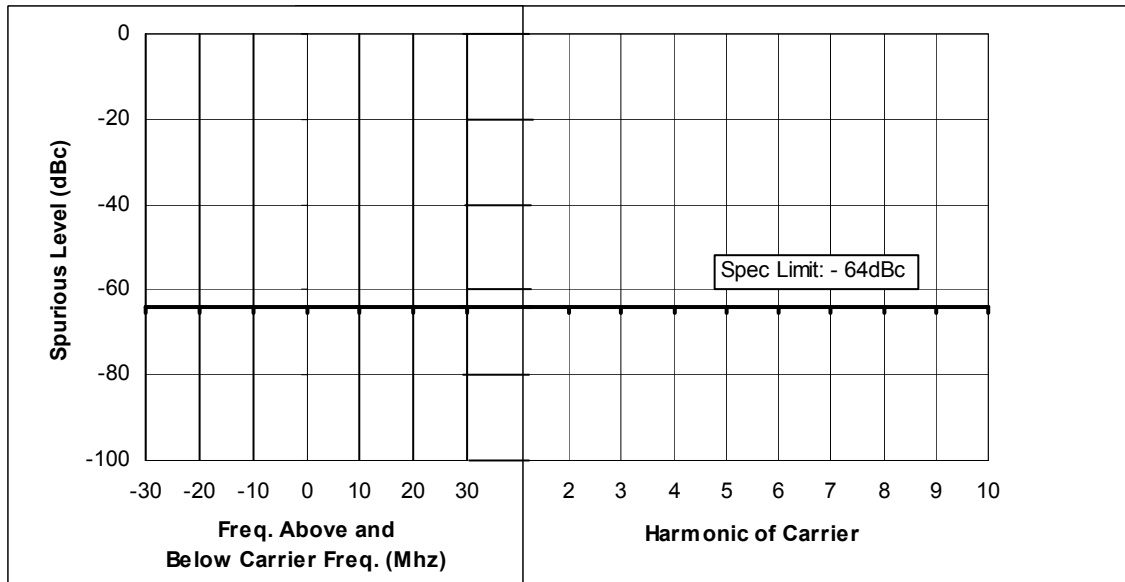
Figure 6F-3: 25 Watts, 161.75 MHz, 12.5 KHz Channel Spacing
