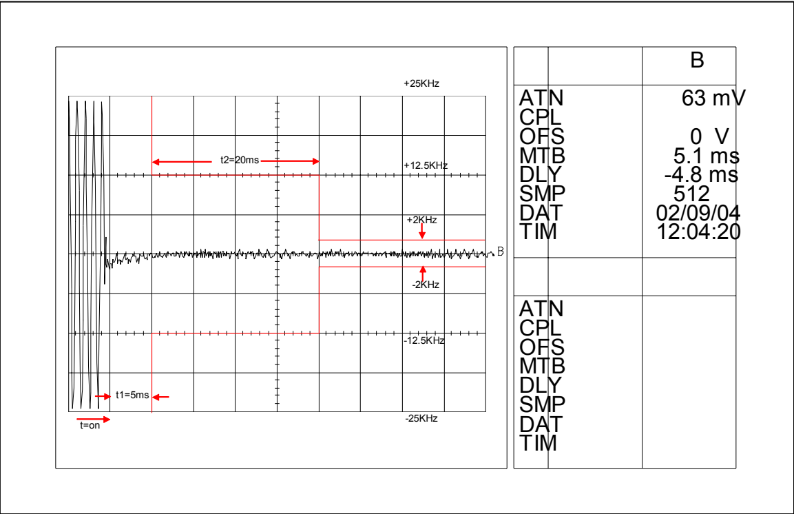
Figure 6I-3: 25 Watts, 25 KHz Key-Up Attack Time
