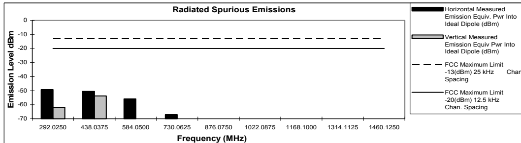
Figure 6G-2 – 28 Watts, 146.0125 MHz
