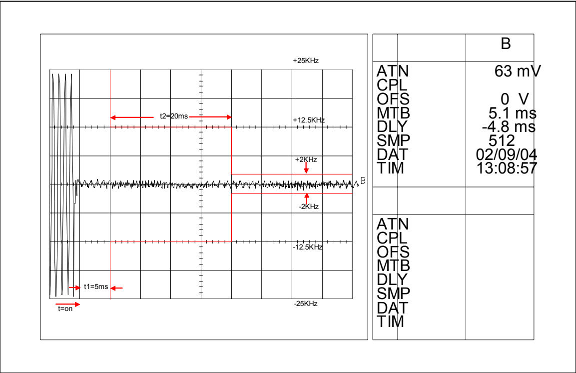
Figure 6I-5: 1 Watts, 12.5 KHz Key-Up Attack Time
