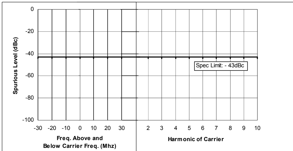
Figure 6F-10: 1 Watts, 136.25 MHz, 25 KHz Channel Spacing
