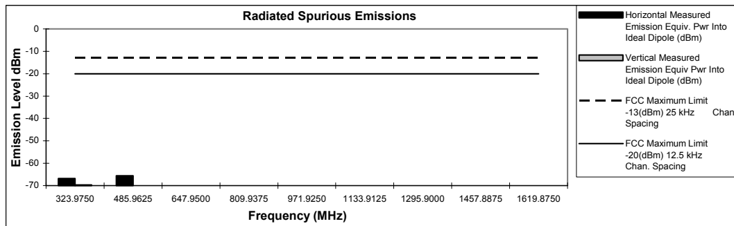
Figure 6G-6 – 1 Watts, 161.9875 MHz
