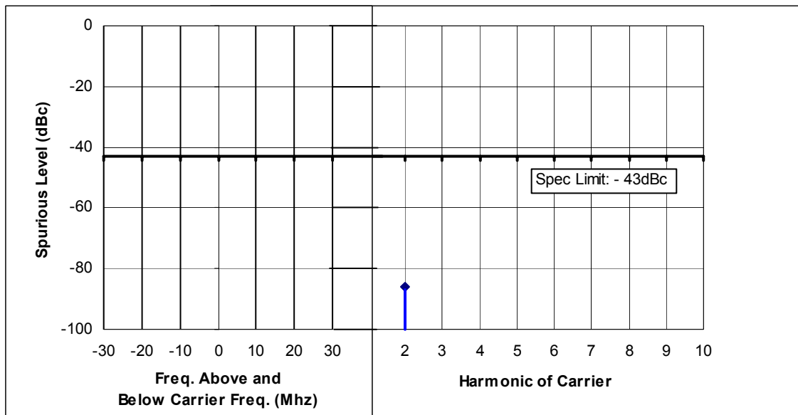
Figure 6F-11: 1 Watts, 149.00 MHz, 25 KHz Channel Spacing
