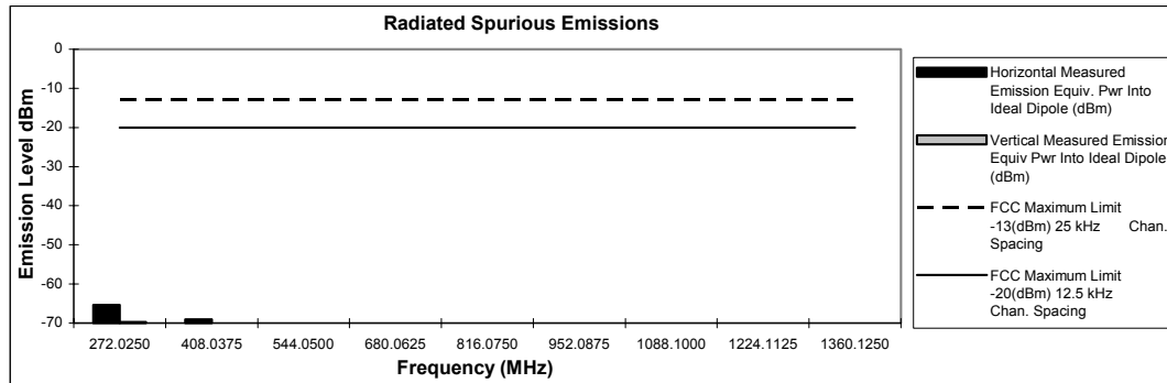
Figure 6G-4 – 1 Watts, 136.0125 MHz
