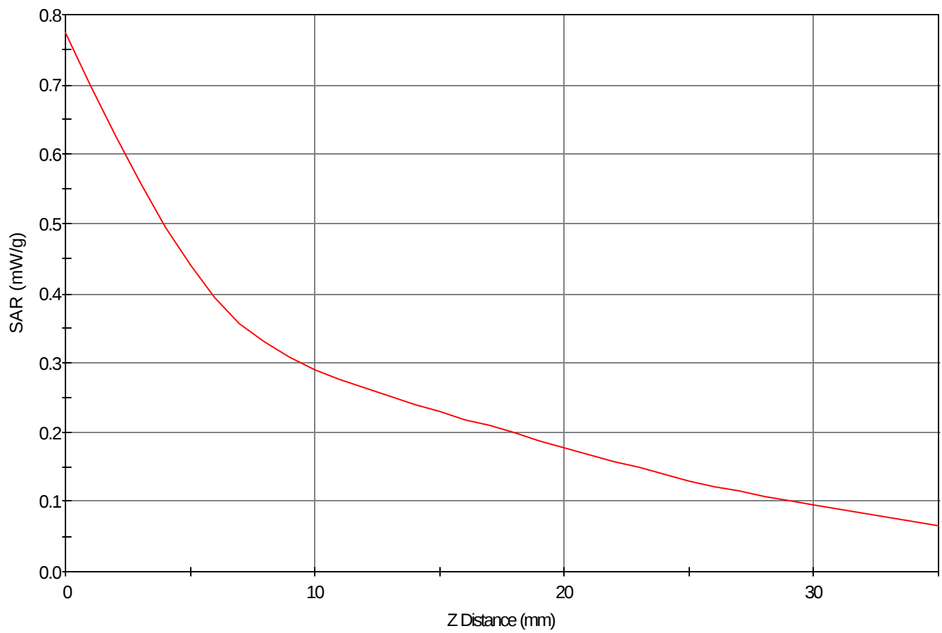
SAR - Z Axis at Hotspot x:109.0 y:-4.0
