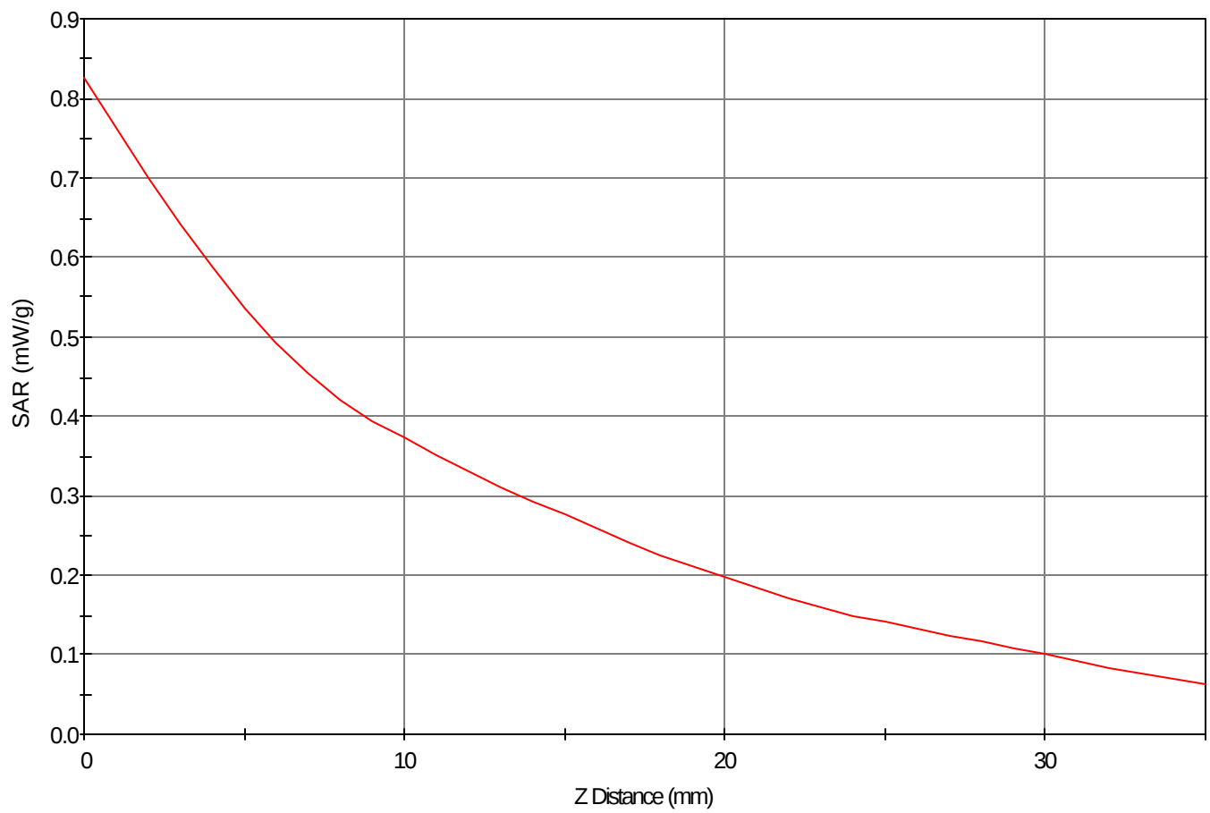
SAR - Z Axis at Hotspot x:104.0 y:-5.0
