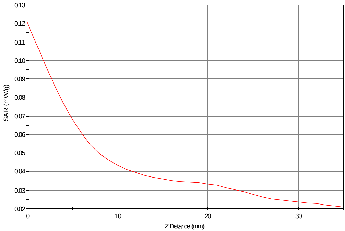
SAR - Z Axis at Hotspot x:115.0 y:-18.0
