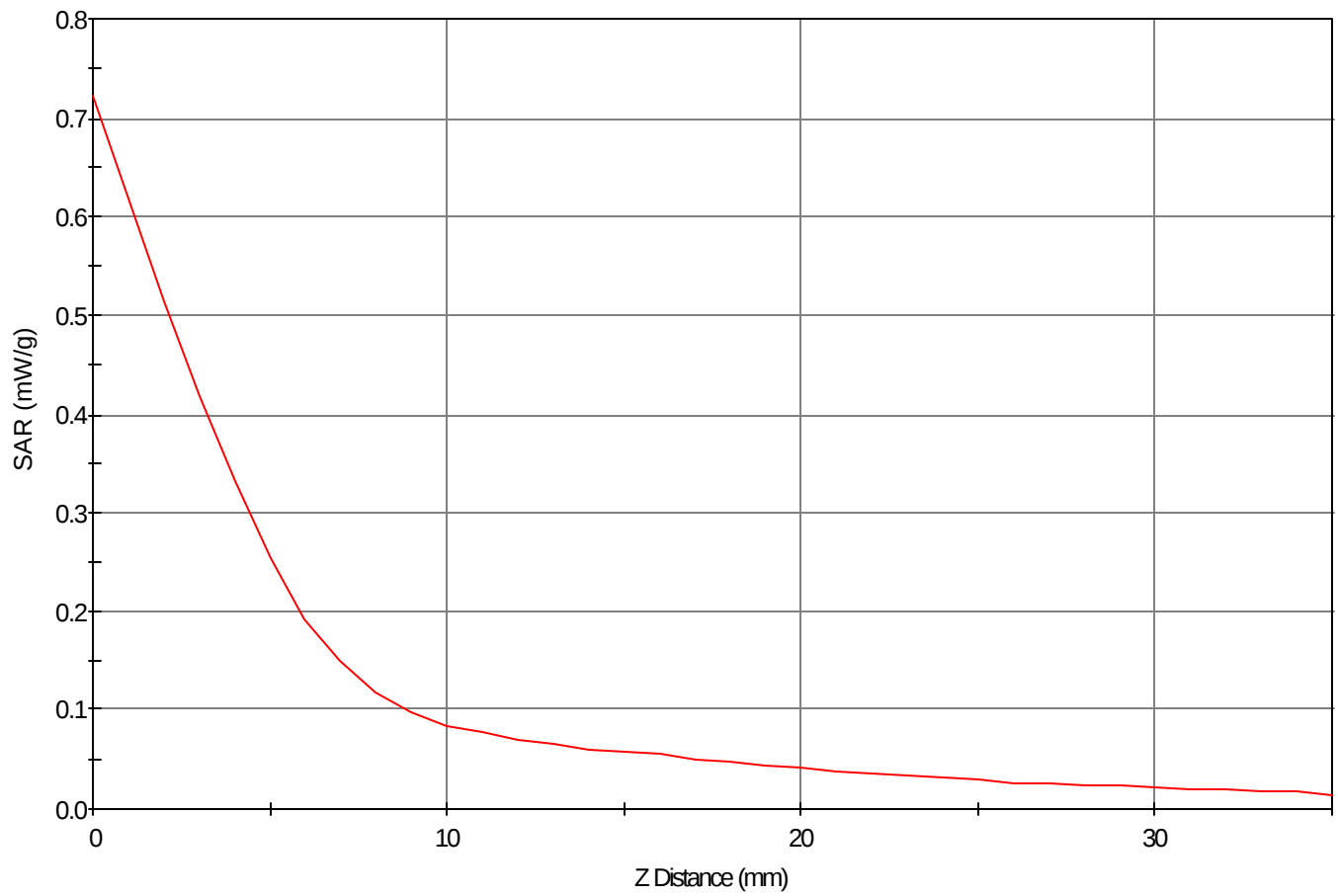
SAR - Z Axis at Hotspot x:10.0 y:-22.0
