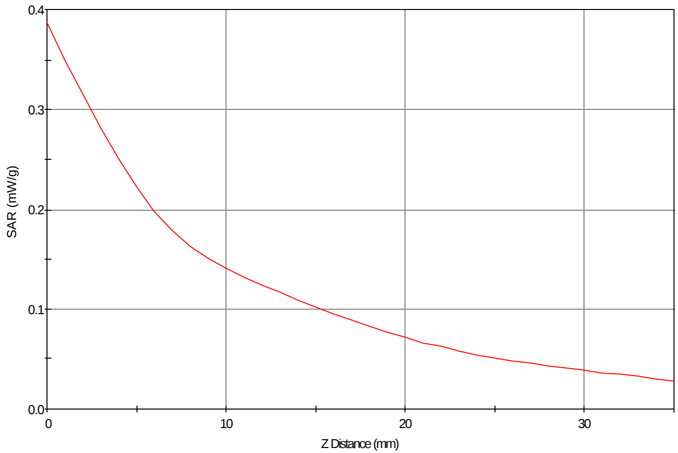
SAR - Z Axis at Hotspot x:108.0 y:17.0
