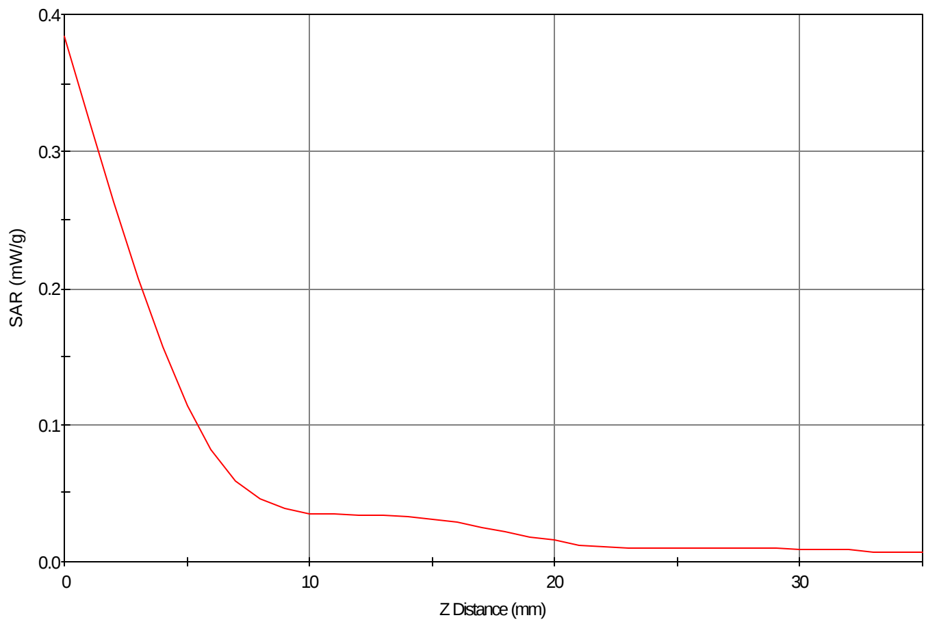
SAR - Z Axis at Hotspot x:11.0 y:17.0
