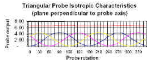
Figure 3.3 Probe Characteristics
