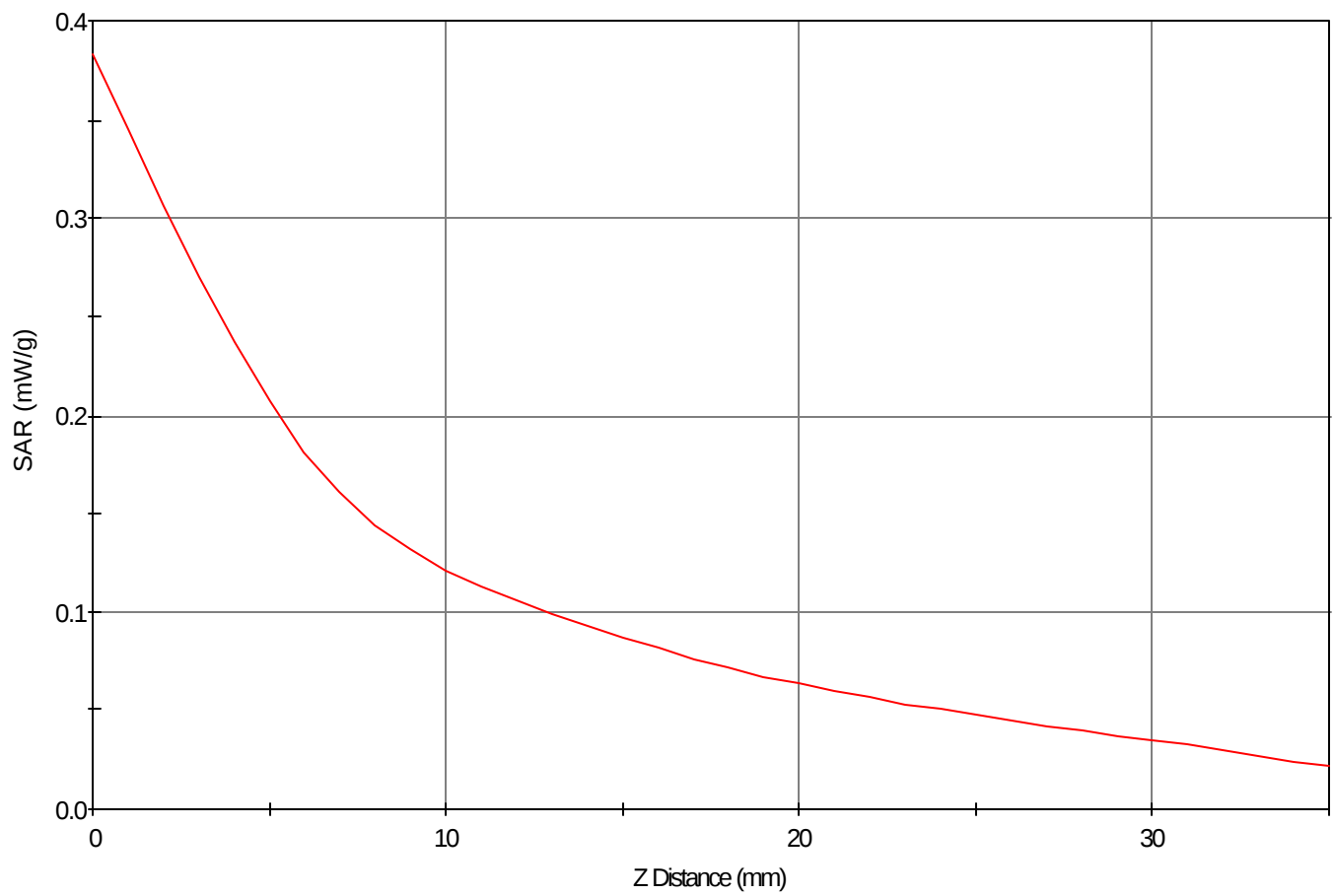
SAR - Z Axis at Hotspot x:107.0 y:-7.0
