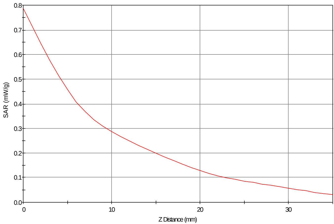
SAR - Z Axis at Hotspot x:20.0 y:-1.0
