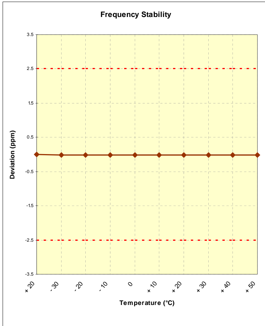
Figure 6-3. Frequency Stability Graph (Cellular WCDMA Mode – Ch. 4183)
