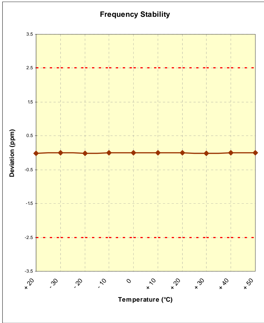
Figure 6-6. Frequency Stability Graph (PCS WCDMA Mode – Ch. 9400)
