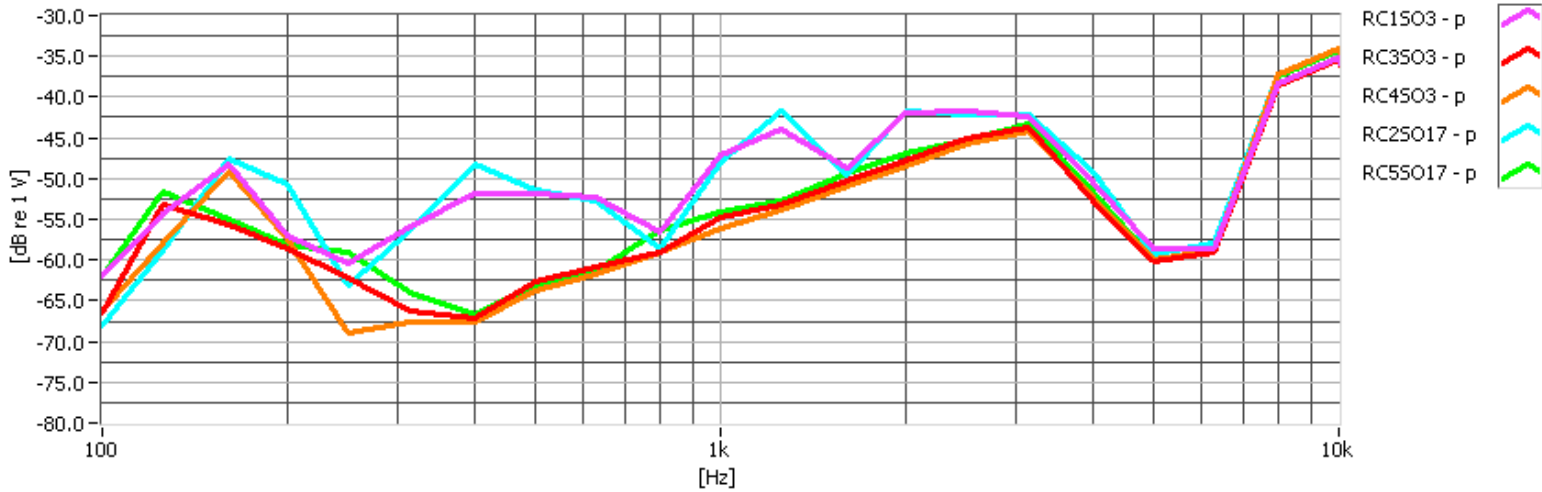
Figure 5-7 Vocoder Analysis for ABM Noise (CDMA)
