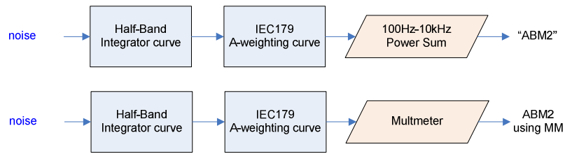
Figure 5-4 ABM2 Validation Block Diagram
