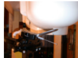
Figure 14.8 Left Head SAR Test Setup -- Ear / Tilt Position --
