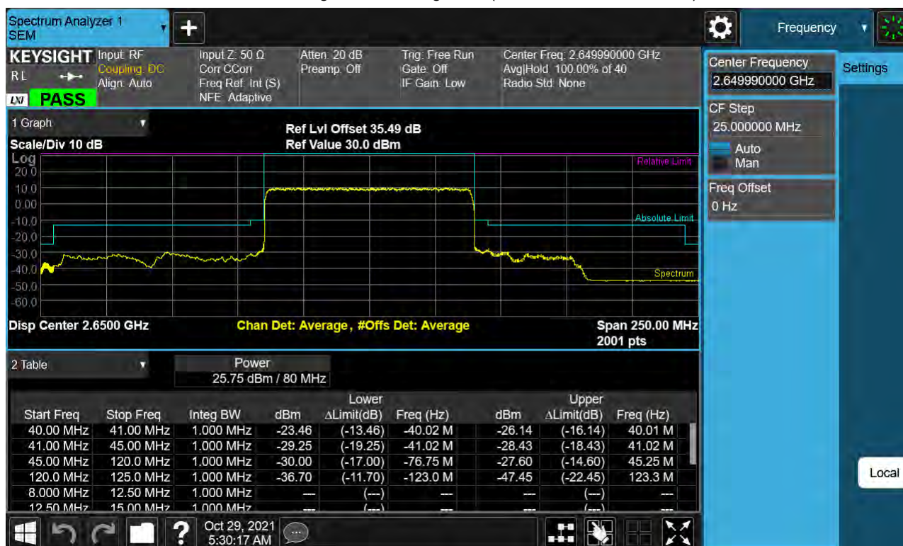
Sub6 n41. High Channel Edge Plot (80 MHz Ch.529998 BPSK)
