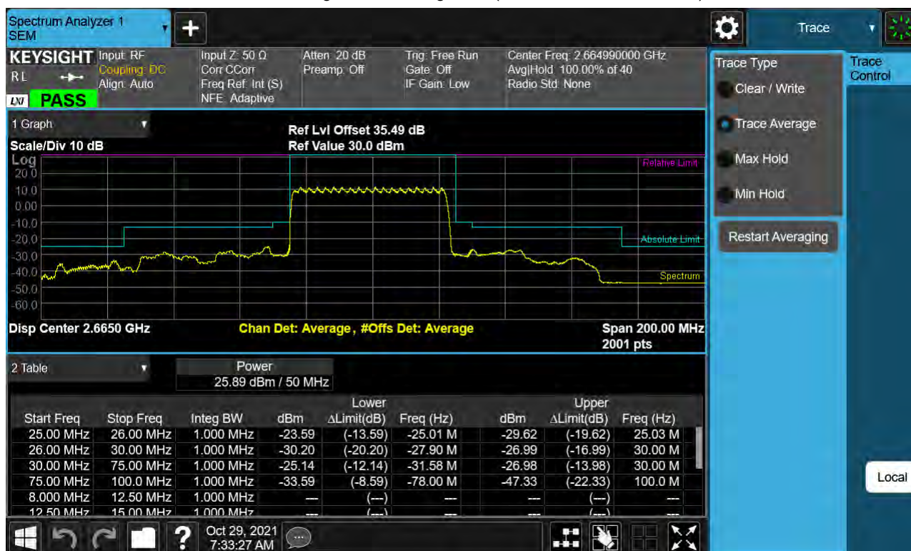
Sub6 n41. High Channel Edge Plot (50 MHz Ch.532998 BPSK)
