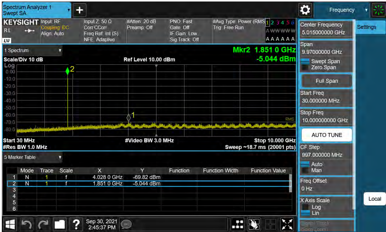
Sub6 n25. Conducted Spurious_1 (374000ch_40 MHz_BPSK_RB 1_1)
