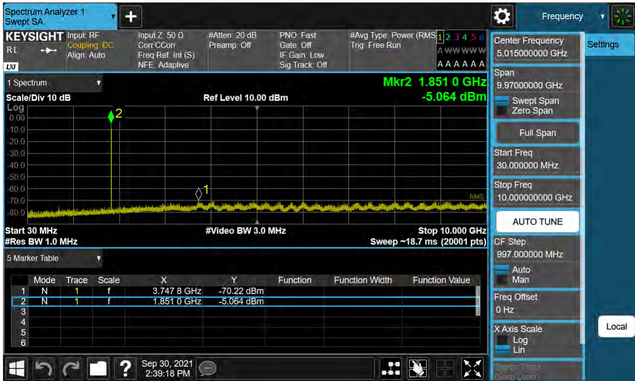
Sub6 n25. Conducted Spurious_1 (373000ch_30 MHz_BPSK_RB 1_1)
