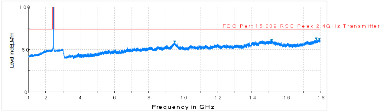
Plot 7-70. Radiated Spurious Plot above 1GHz (802.11b – Ch. 6, Ant. Pol. V)
