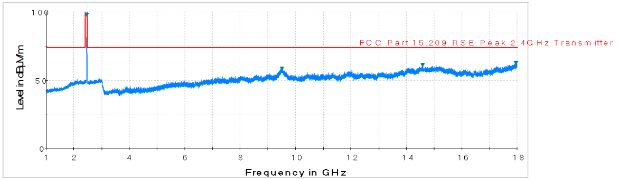
Plot 7-80. Radiated Spurious Plot above 1GHz (802.11b – Ch. 11, Ant. Pol. V)
