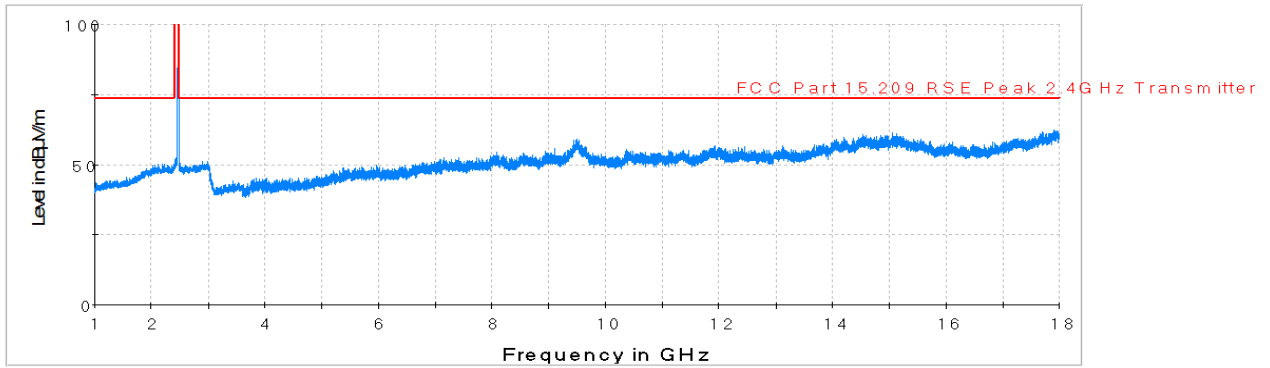
Plot 7-72. Radiated Spurious Plot above 1GHz (802.11b – Ch. 11, Ant. Pol. V)
