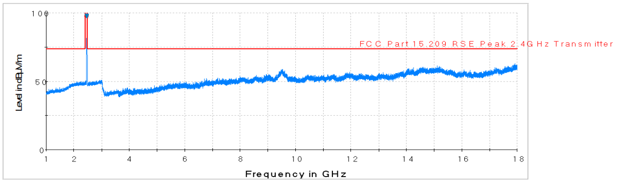
Plot 7-79. Radiated Spurious Plot above 1GHz (802.11b – Ch. 11, Ant. Pol. H)
