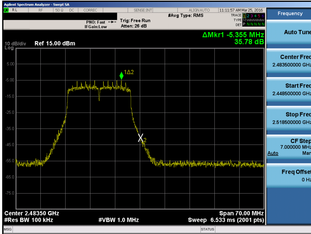
Plot 7-45. Band Edge Plot (802.11n (2.4GHz) – Ch. 13)
