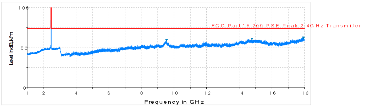
Plot 7-71. Radiated Spurious Plot above 1GHz (802.11b – Ch. 11, Ant. Pol. H)
