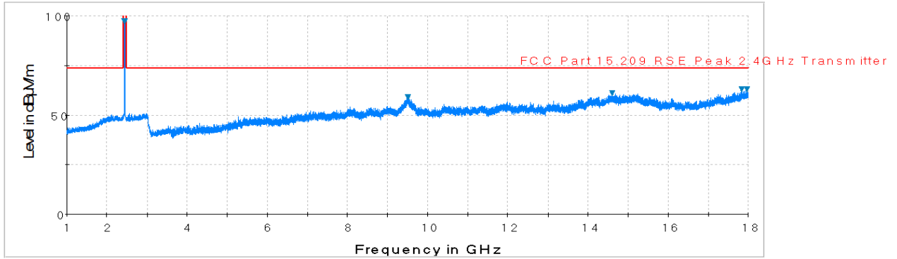
Plot 7-78. Radiated Spurious Plot above 1GHz (802.11b – Ch. 6, Ant. Pol. V)
