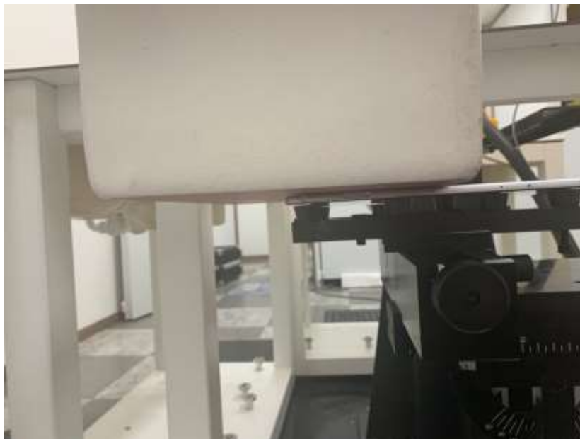
Distance of 0 mm from the EUT (With Holder)
