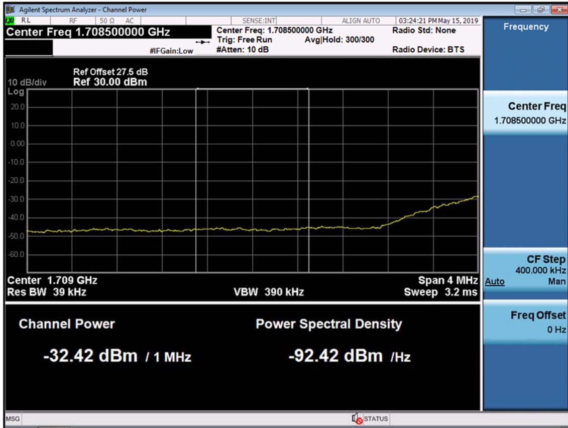
BAND 66/4. Lower Extended Band Edge Plot (15M BW Ch.132047 QPSK_RB75_0) -3
