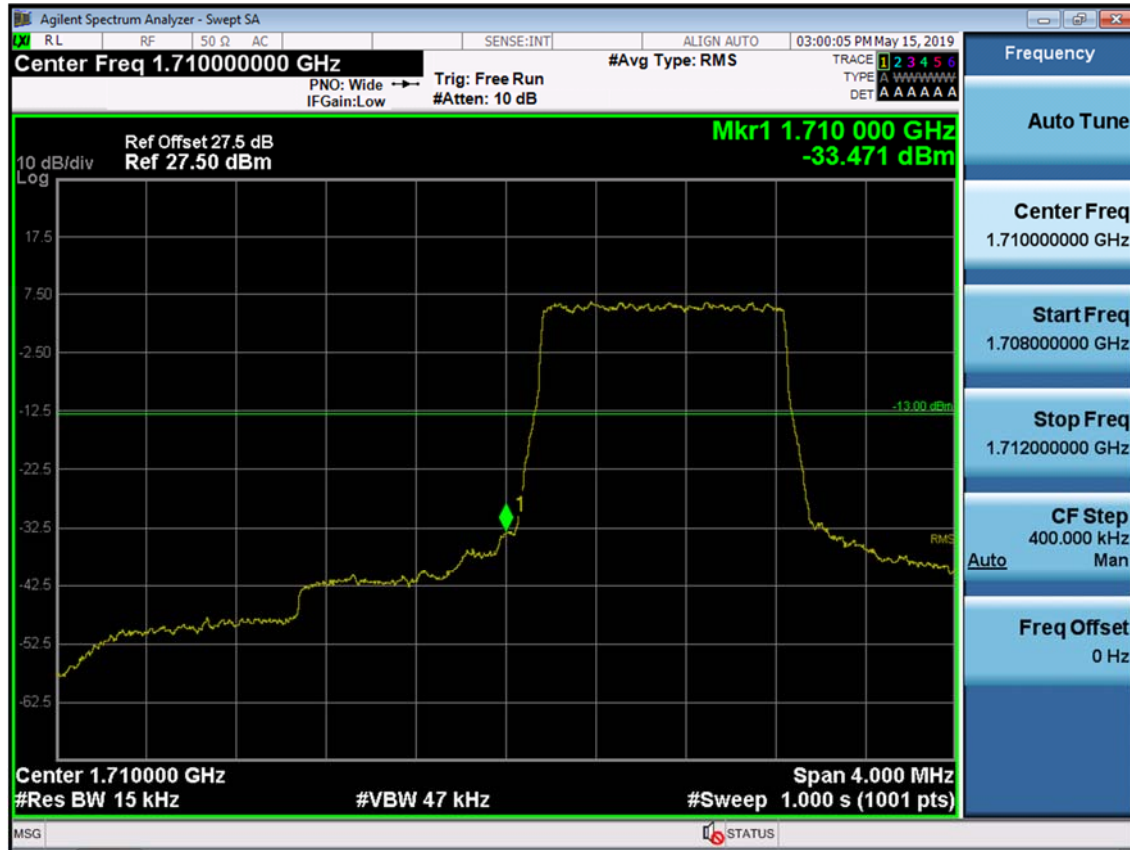
BAND 66/4. Lower Band Edge Plot (1.4M BW Ch.131979 QPSK RB 6) -2
