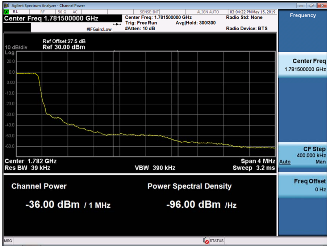
BAND 66/4. Upper Extended Band Edge Plot (1.4M BW Ch. 132665 QPSK_RB6_0) -3
