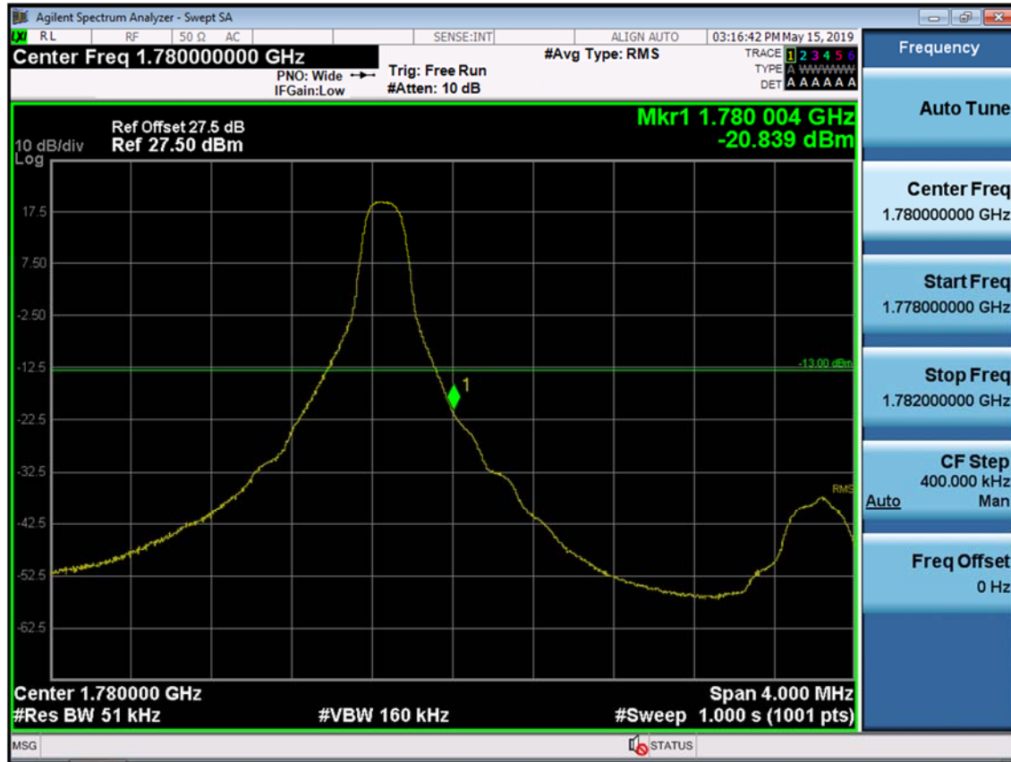
BAND 66/4. Upper Band Edge Plot (5M BW Ch.132647 QPSK_RB1_Offset 24) -1
