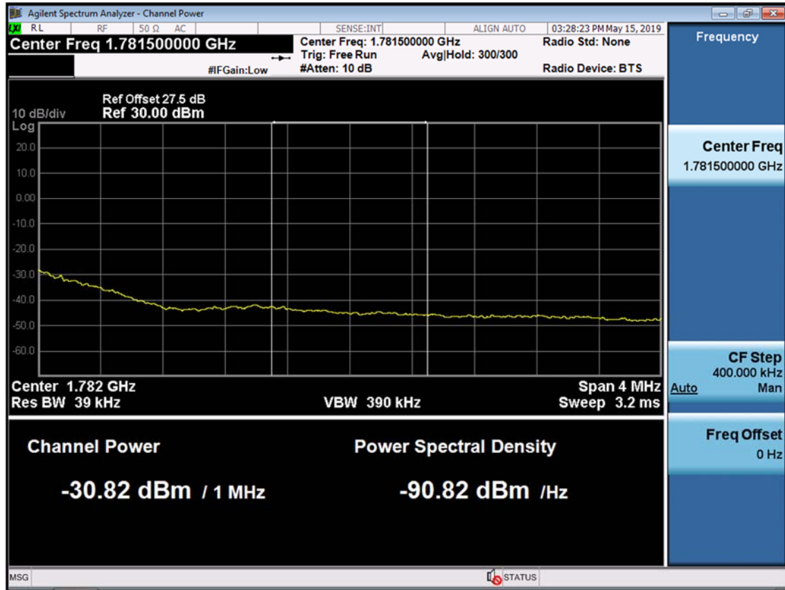
BAND 66/4. Upper Extended Band Edge Plot (15M BW Ch.132597 QPSK_RB75) -3
