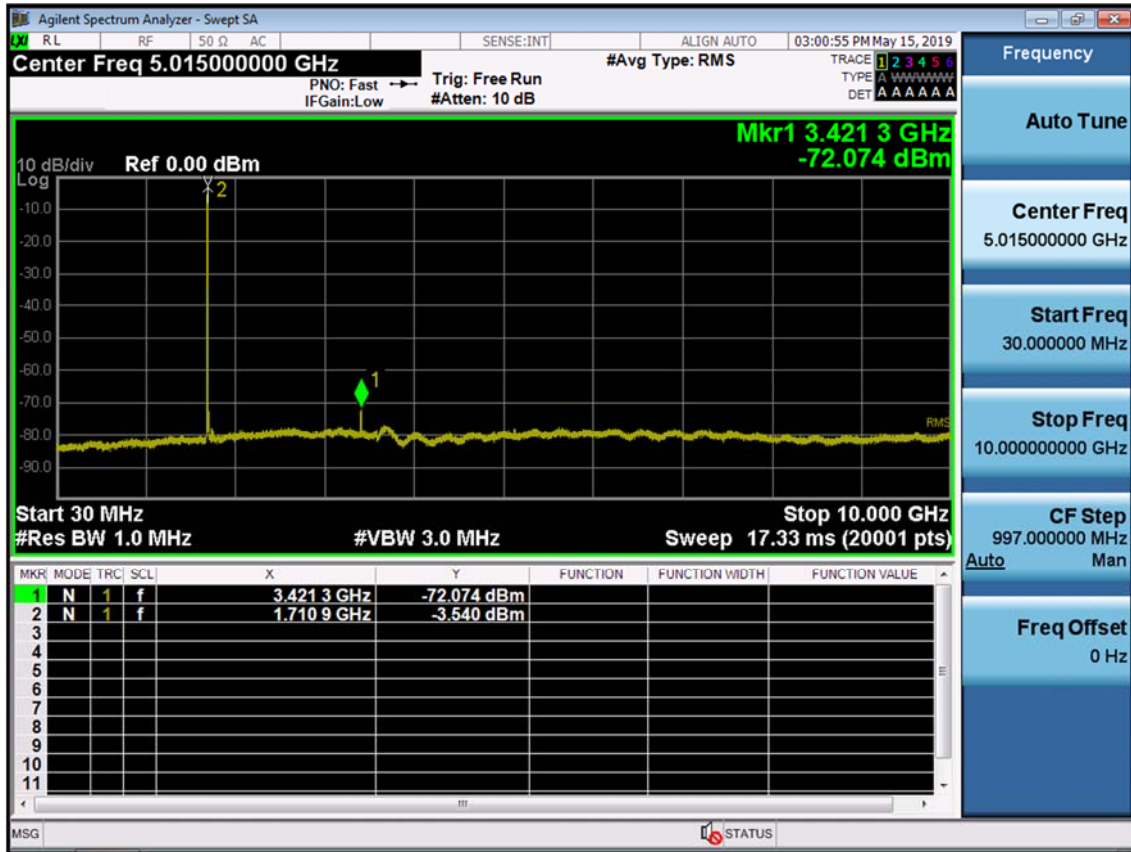
BAND 66/4. Conducted Spurious Plot_1 (131979ch_1.4MHz_QPSK_RB 1_0)
