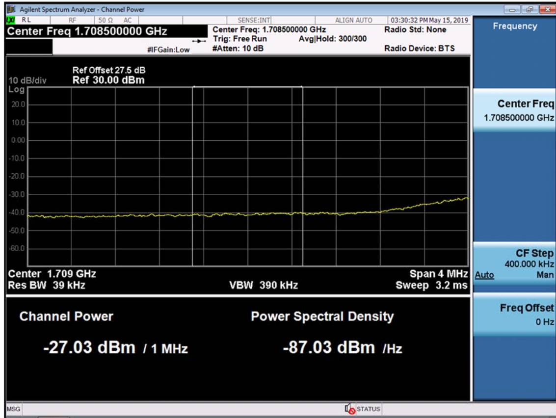
BAND 66/4. Lower Extended Band Edge Plot (20M BW Ch.132072 QPSK_RB100_0) -3
