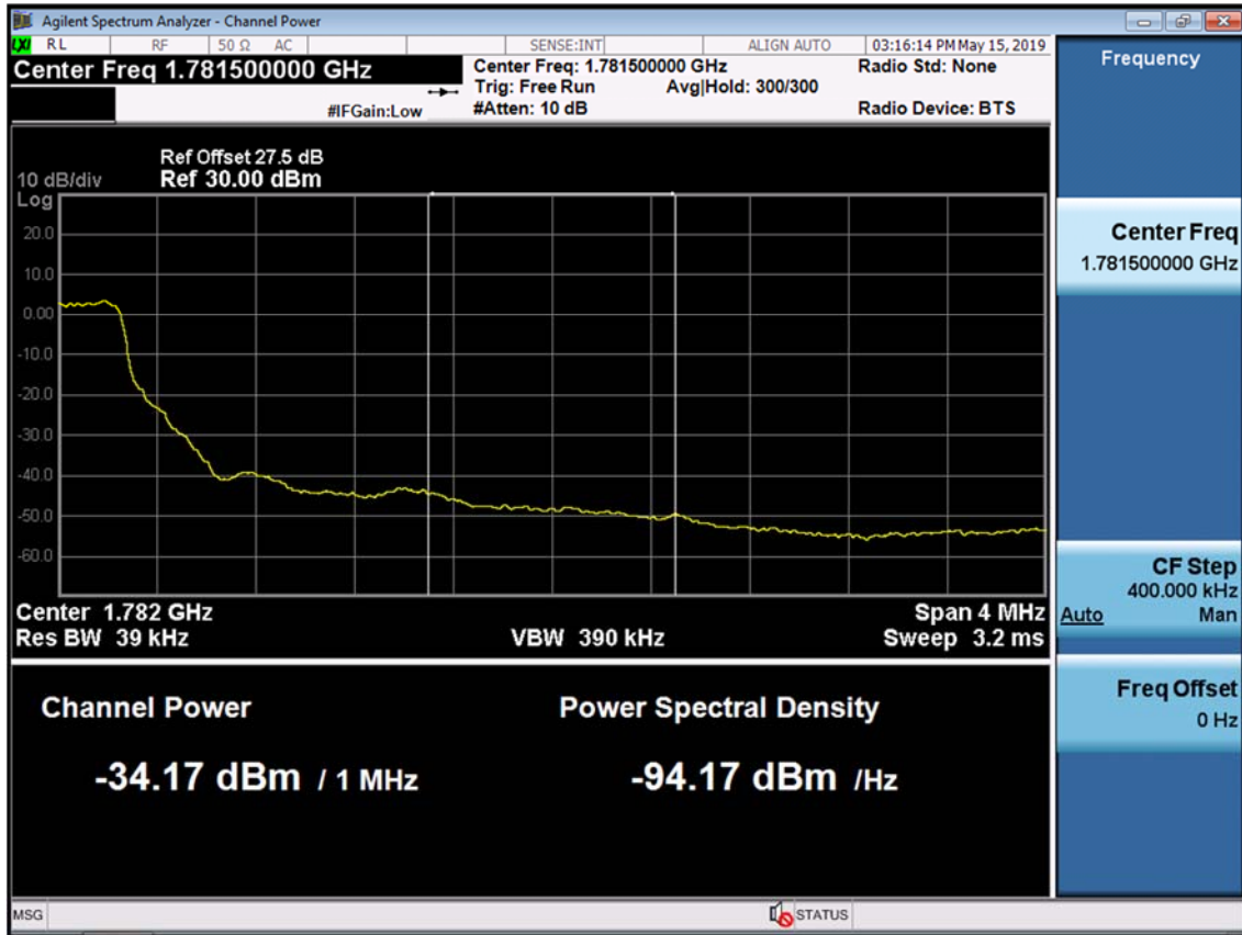
BAND 66/4. Upper Extended Band Edge Plot (5M BW Ch.132647 QPSK_RB25) -3
