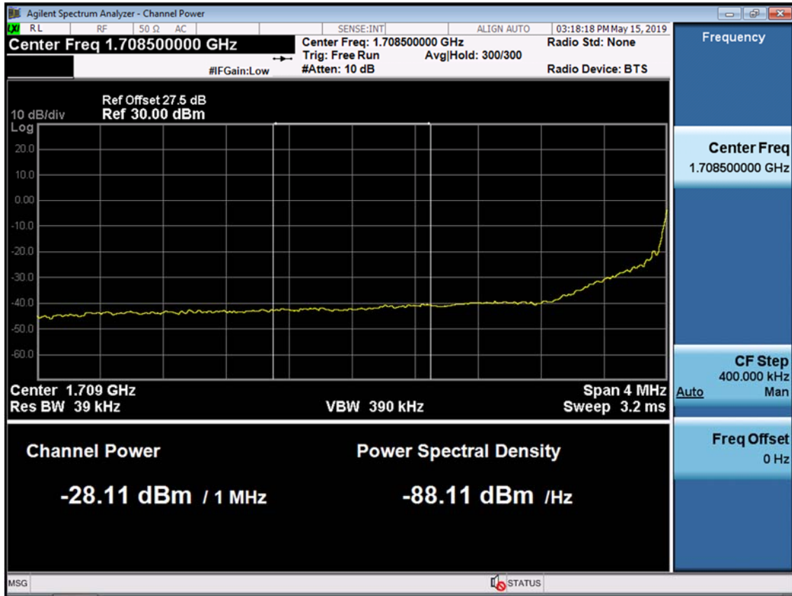
BAND 66/4. Lower Extended Band Edge Plot (10M BW Ch.132022 QPSK_RB50_0) -3
