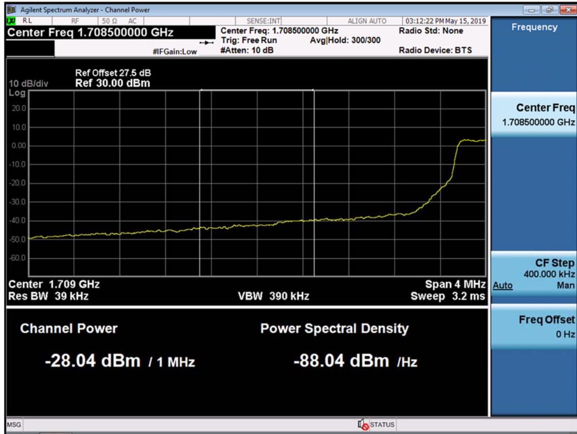
BAND 66/4. Lower Extended Band Edge Plot (5M BW Ch.131997 QPSK_RB25_0) -3
