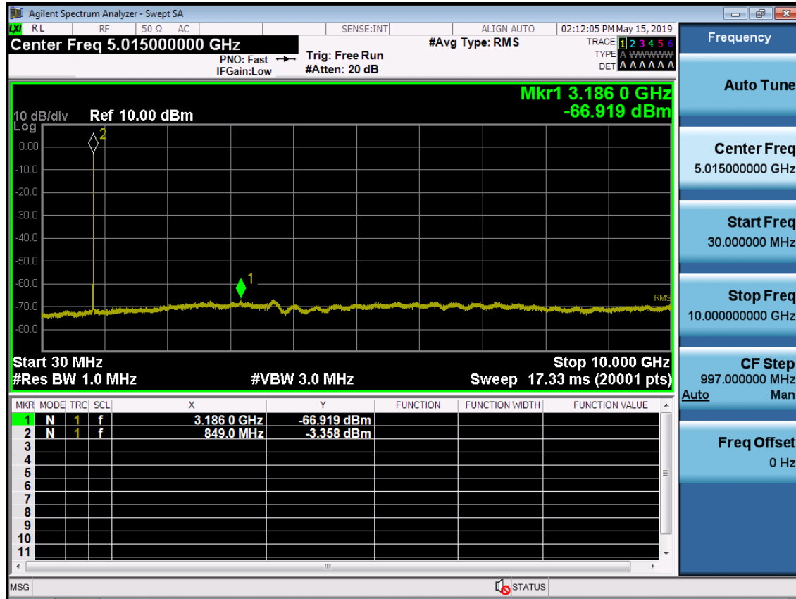
BAND 5. Conducted Spurious Plot (20600ch_10MHz_QPSK_RB 1_0)
