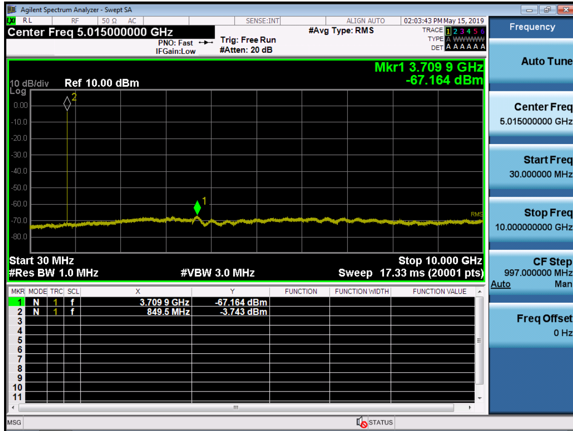
BAND 5. Conducted Spurious Plot (20635ch_3MHz_QPSK_RB 1_0)
