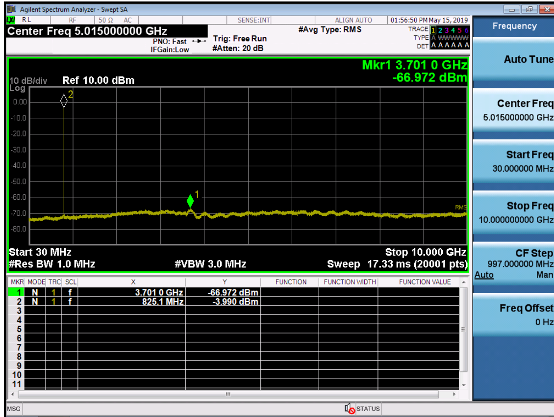
BAND 5. Conducted Spurious Plot (20407ch_1.4MHz_QPSK_RB 1_0)
