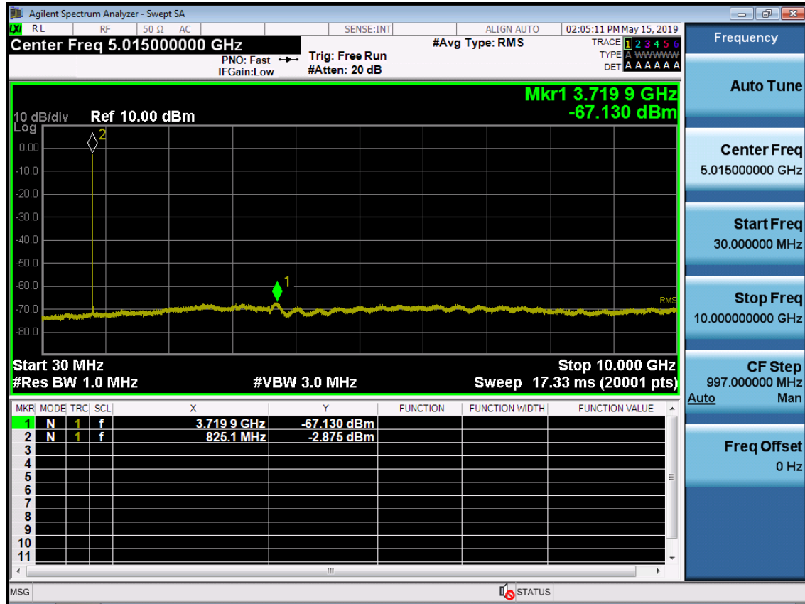
BAND 5. Conducted Spurious Plot (20425ch_5MHz_QPSK_RB 1_0)
