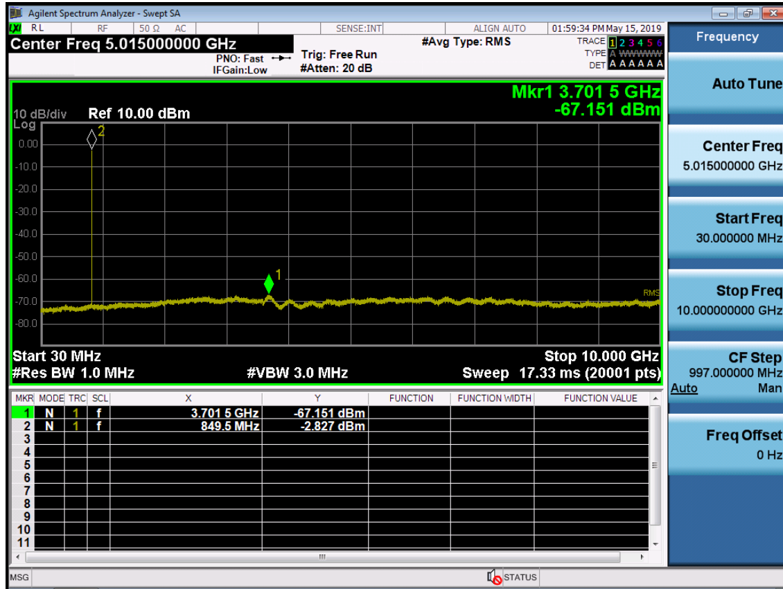
BAND 5. Conducted Spurious Plot (20643ch_1.4MHz_QPSK_RB 1_0)
