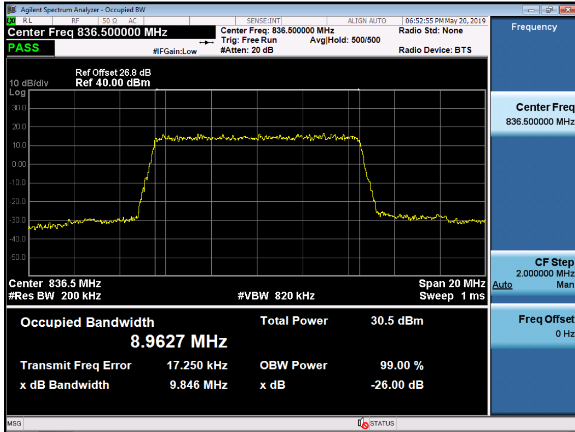
BAND 5. Occupied Bandwidth Plot (10M BW Ch.20525 64QAM_RB50_0)
