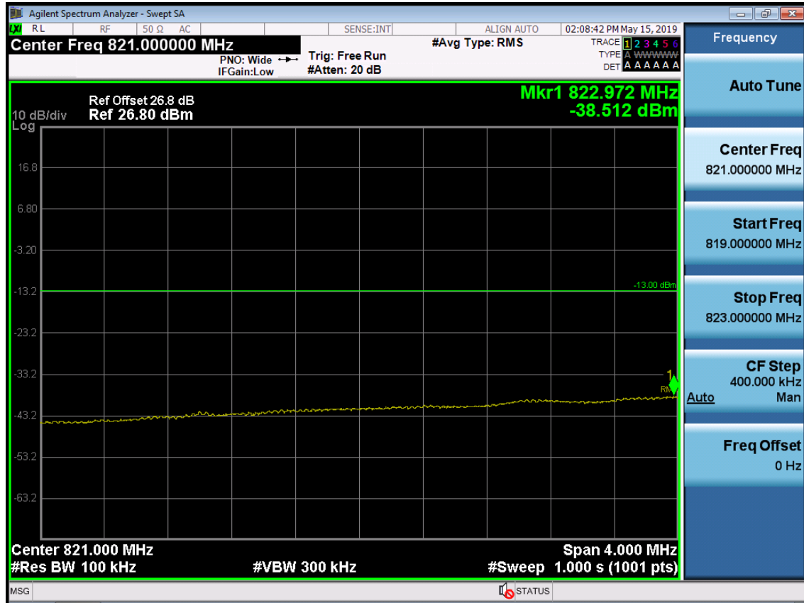
BAND 5. Lower Extended Band Edge Plot (10M BW Ch.20450 QPSK_RB50_0)
