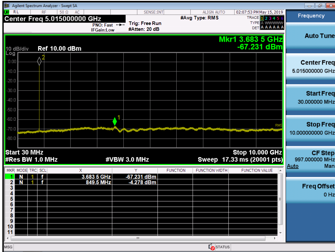
BAND 5. Conducted Spurious Plot (20625ch_5MHz_QPSK_RB 1_0)
