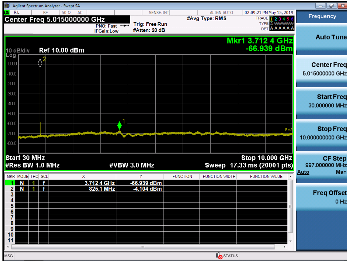
BAND 5. Conducted Spurious Plot (20450ch_10MHz_QPSK_RB 1_0)
