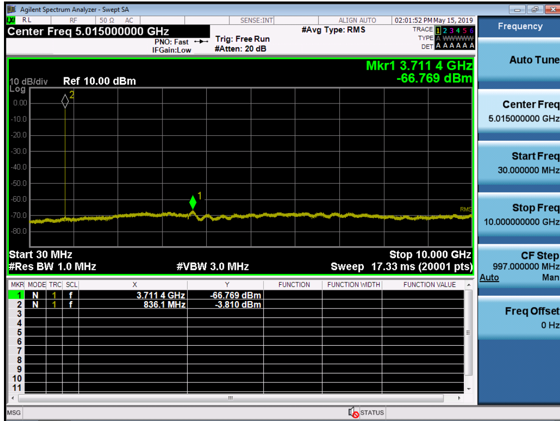
BAND 5. Conducted Spurious Plot (20525ch_3MHz_QPSK_RB 1_0)
