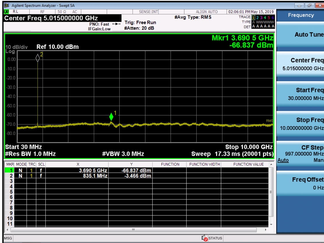
BAND 5. Conducted Spurious Plot (20525ch_5MHz_QPSK_RB 1_0)
