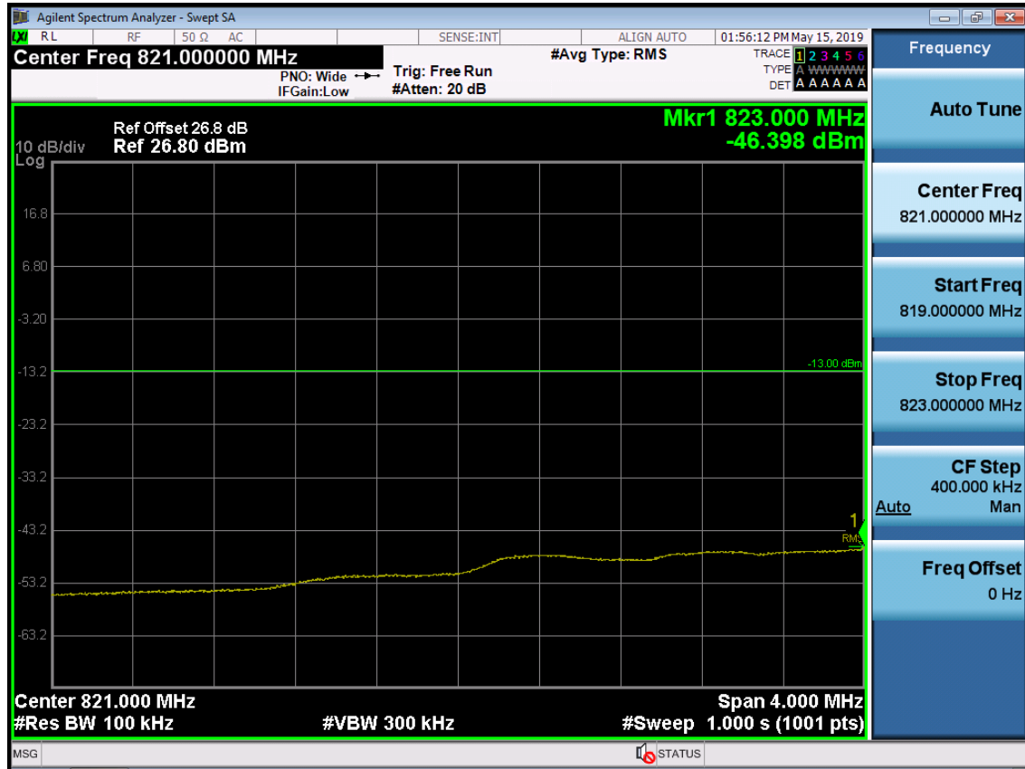
BAND 5. Lower Extended Band Edge Plot (1.4M BW Ch.20407 QPSK_RB6_0)
