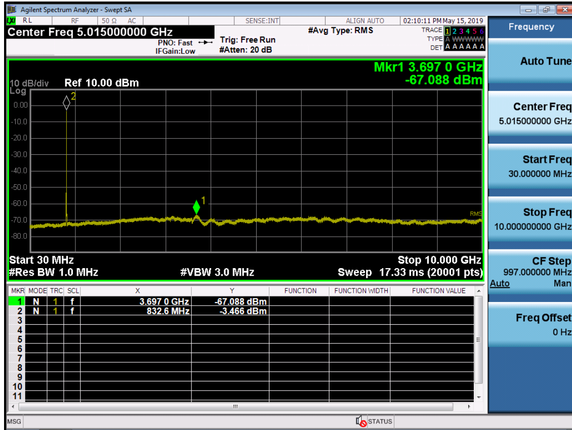
BAND 5. Conducted Spurious Plot (20525ch_10MHz_QPSK_RB 1_0)
