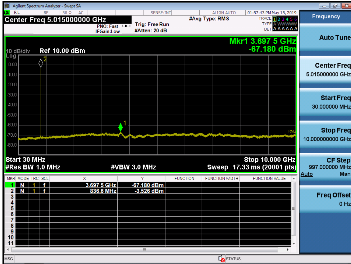
BAND 5. Conducted Spurious Plot (20525ch_1.4MHz_QPSK_RB 1_0)
