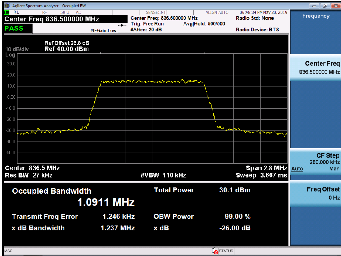
BAND 5. Occupied Bandwidth Plot (1.4M BW Ch.20525 64QAM_RB6_0)
