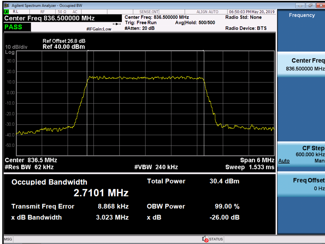
BAND 5. Occupied Bandwidth Plot (3M BW Ch.20525 64QAM_RB15_0)
