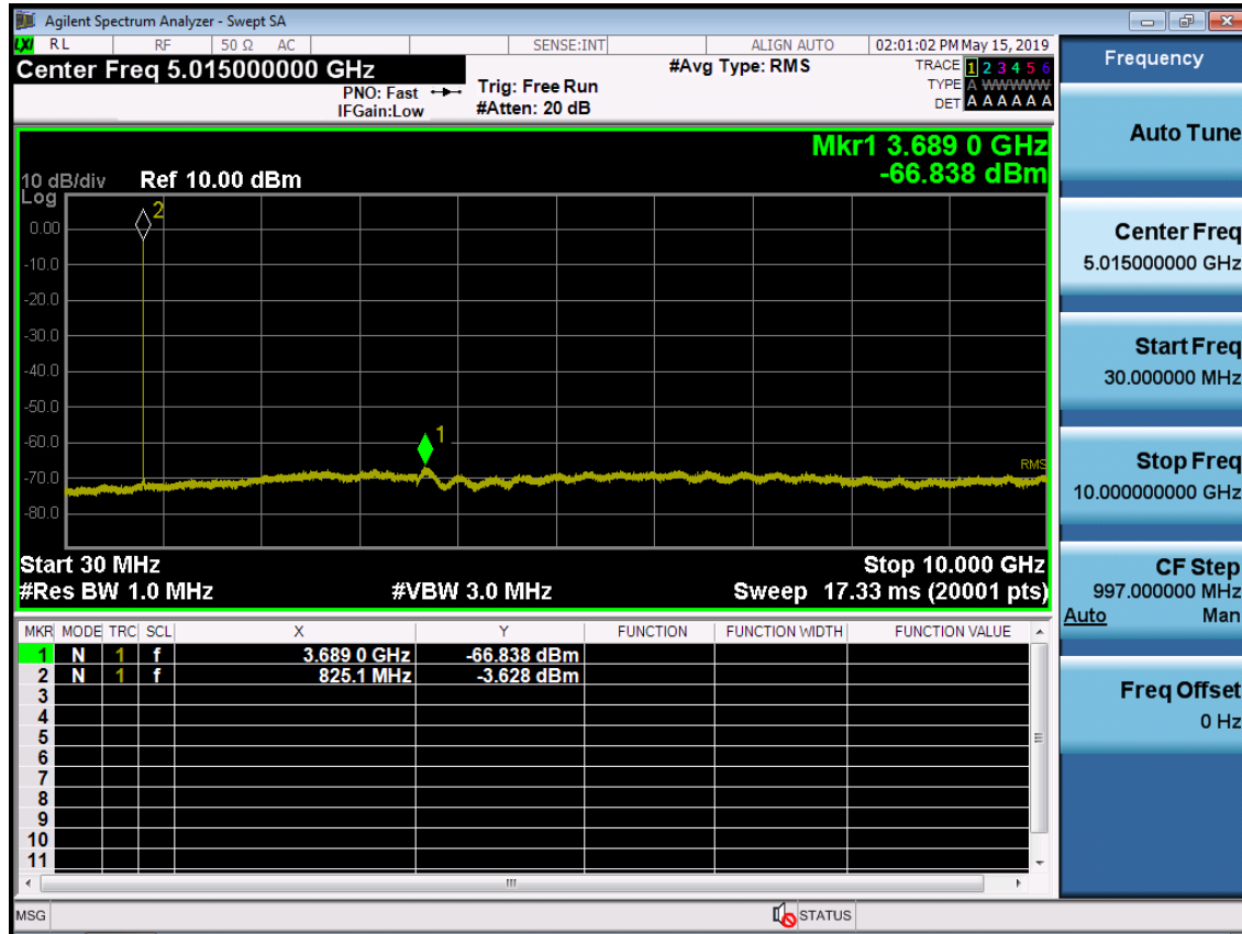
BAND 5. Conducted Spurious Plot (20415ch_3MHz_QPSK_RB 1_0)
