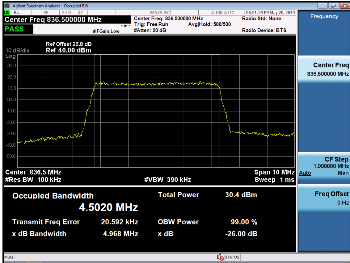
BAND 5. Occupied Bandwidth Plot (5M BW Ch.20525 64QAM_RB25_0)
