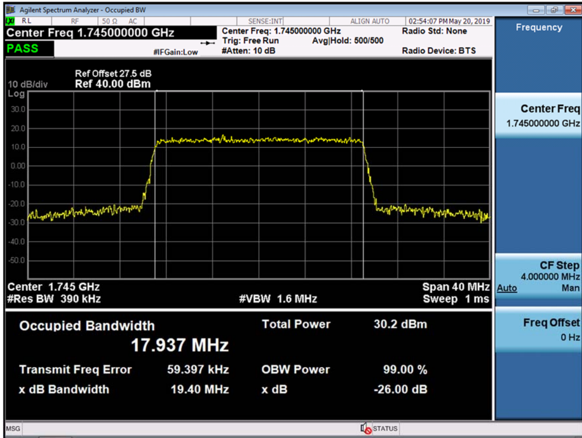
BAND 66/4. Occupied Bandwidth Plot (20M BW Ch.132322 64QAM RB 100)
