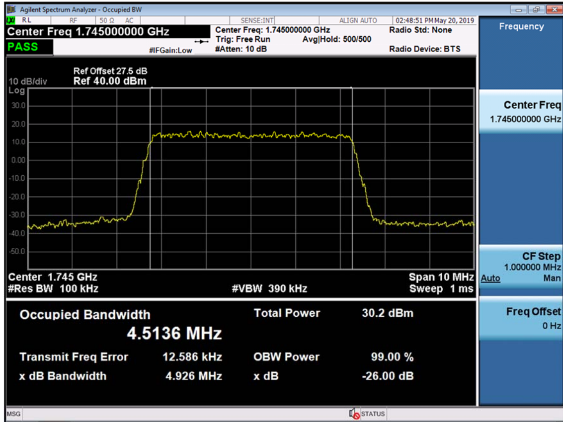
BAND 66/4. Occupied Bandwidth Plot (5M BW Ch.132322 64QAM RB 25)
