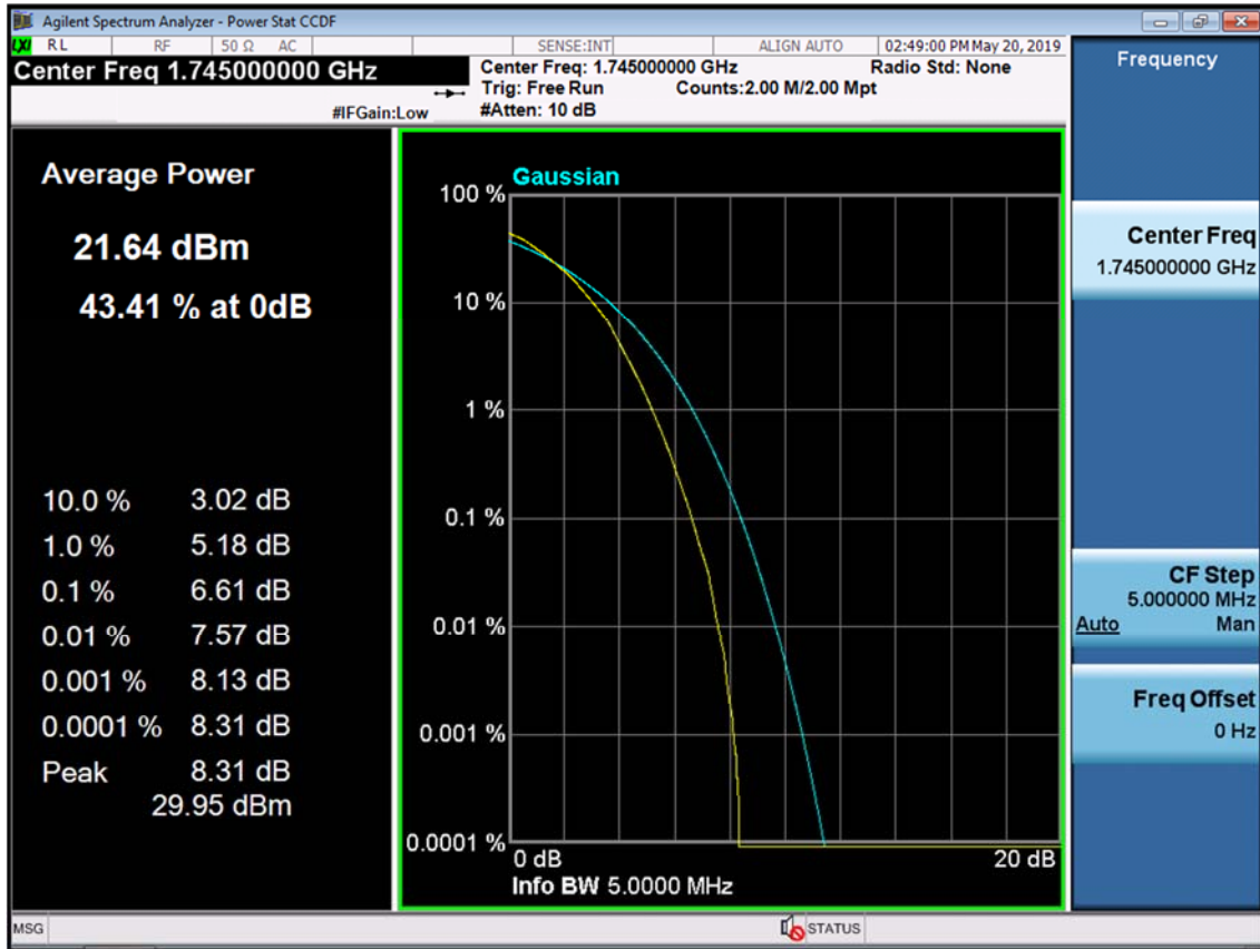
BAND 66/4. PAR Plot (5M BW_Ch.132322_64QAM_RB25_0)
