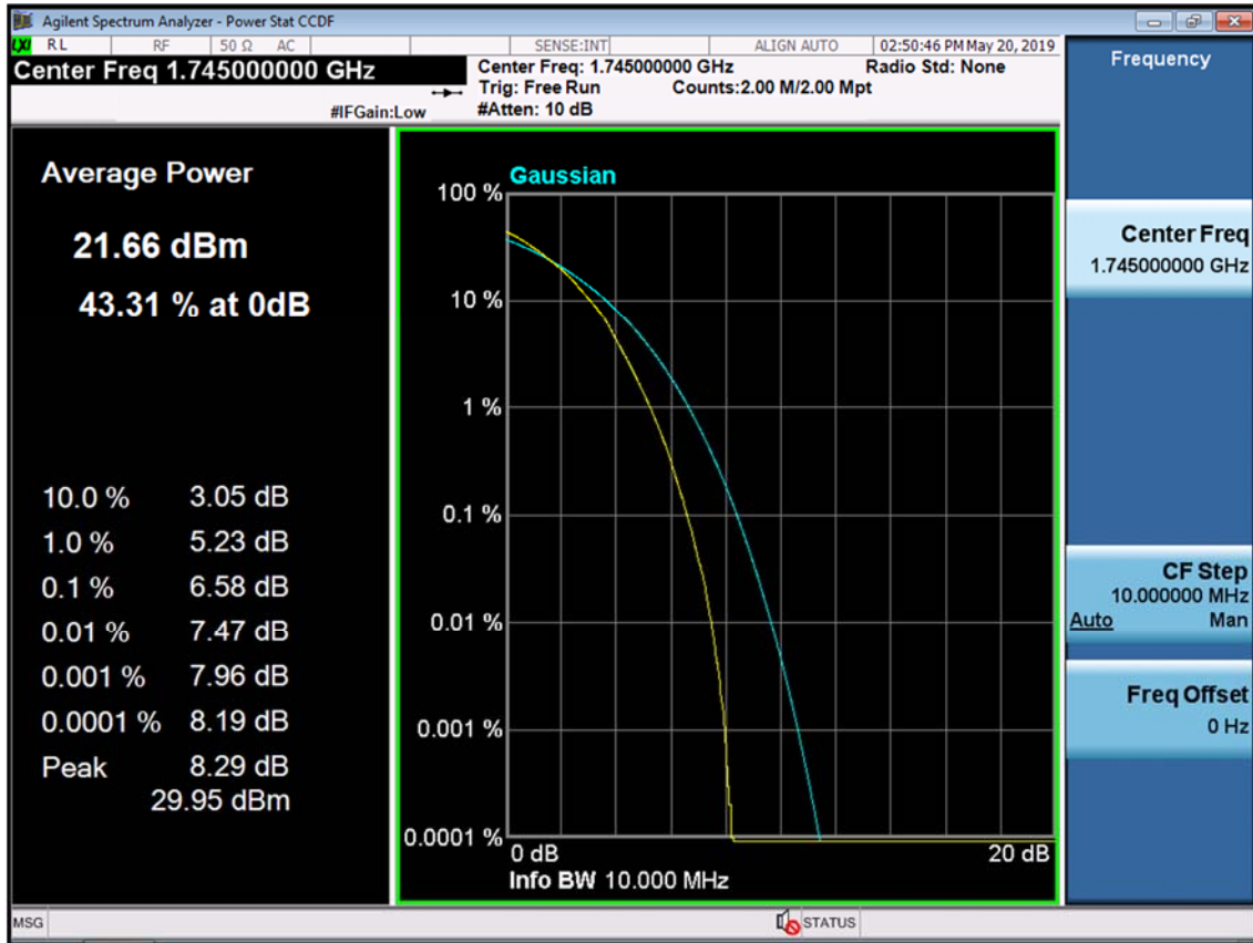
BAND 66/4. PAR Plot (10M BW_Ch.132322_64QAM_RB50_0)
