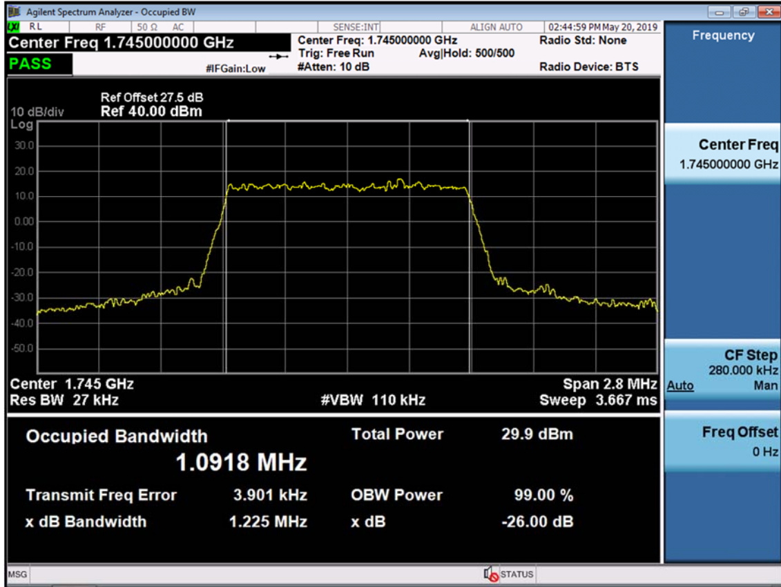
BAND 66/4. Occupied Bandwidth Plot (1.4M BW Ch.132322 64QAM RB 6)
