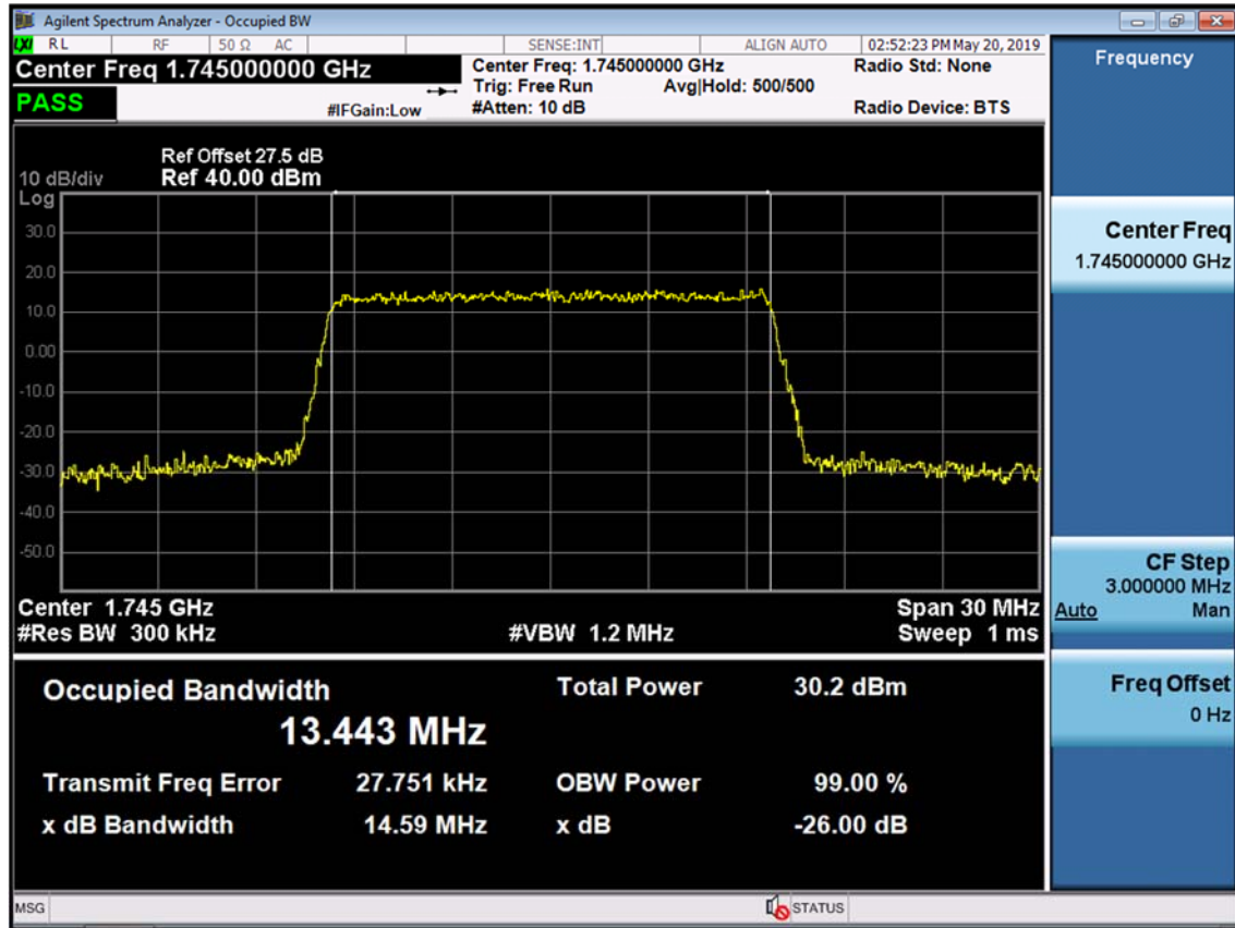
BAND 66/4. Occupied Bandwidth Plot (15M BW Ch.132322 64QAM RB 75)
