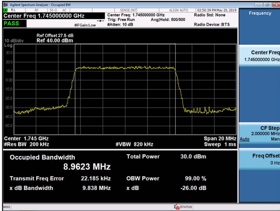
BAND 66/4. Occupied Bandwidth Plot (10M BW Ch.132322 64QAM RB 50)
