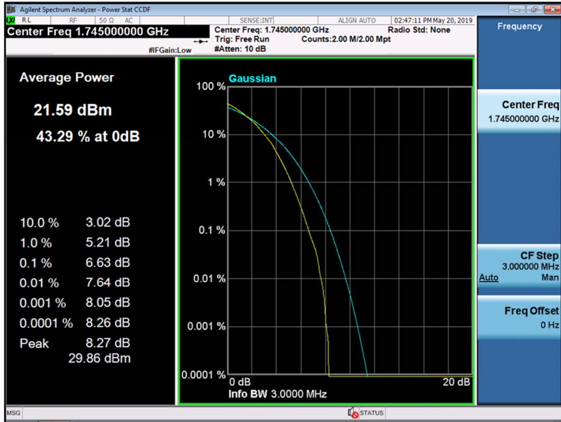
BAND 66/4. PAR Plot (3M BW_Ch.132322_64QAM_RB15_0)
