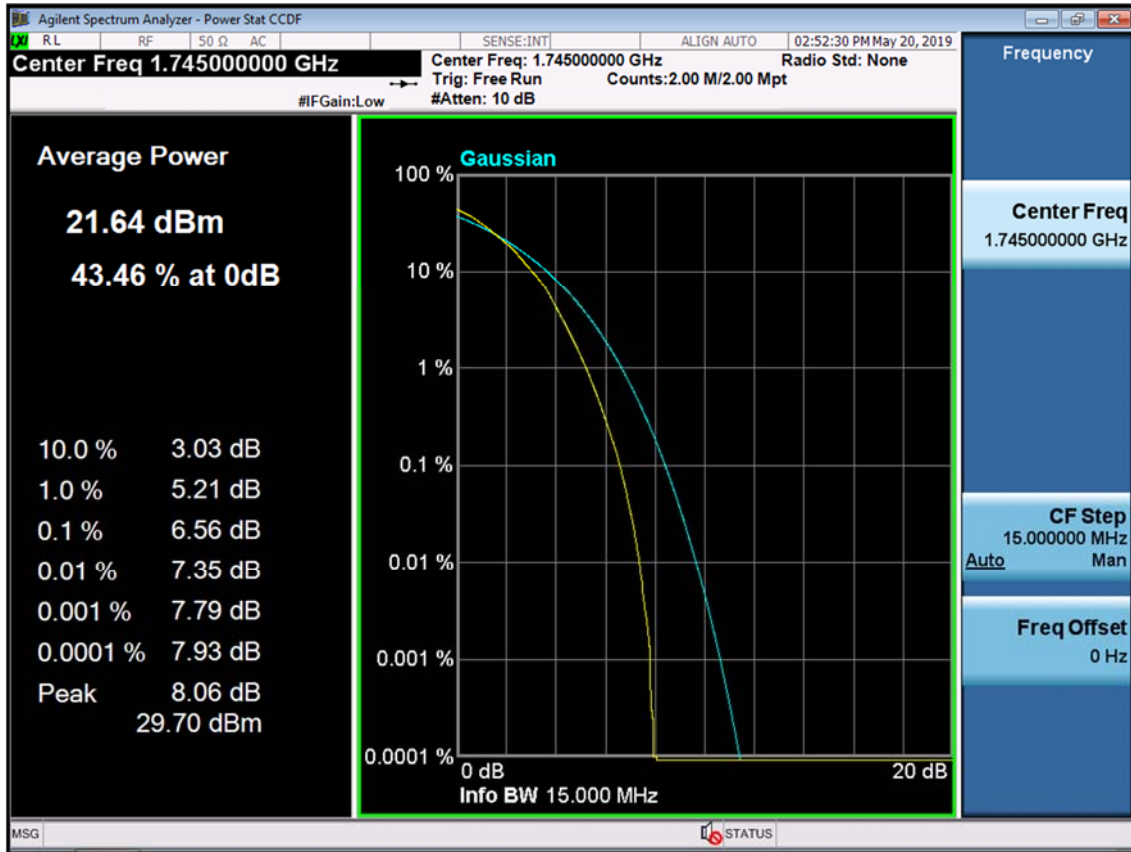
BAND 66/4. PAR Plot (15M BW_Ch.132322_64QAM_RB75_0)
