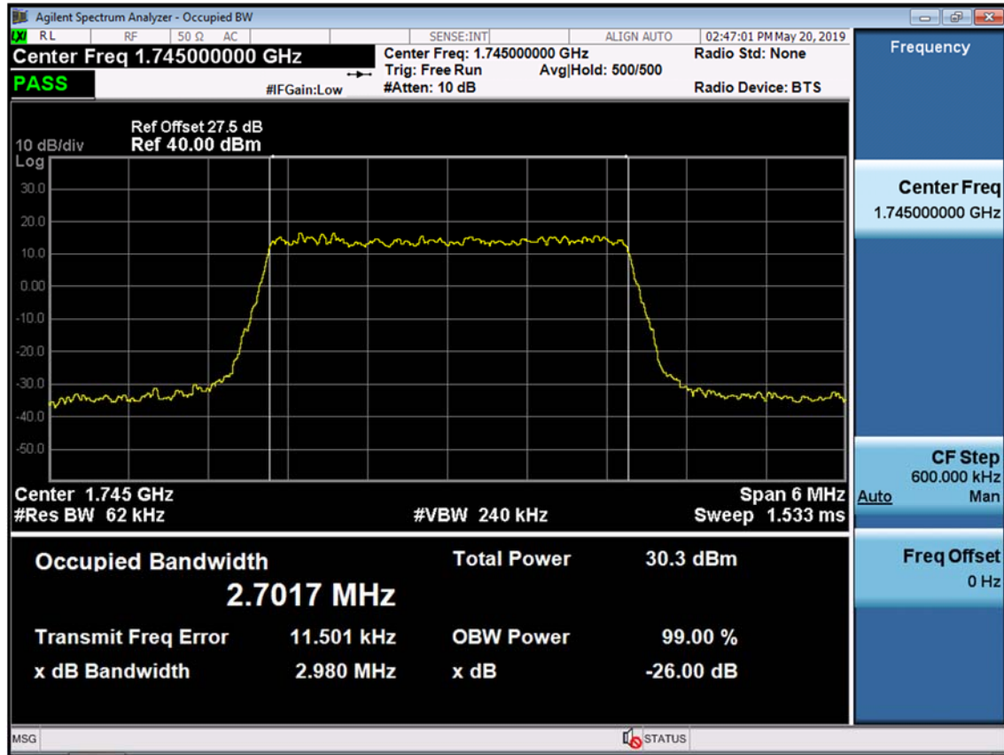
BAND 66/4. Occupied Bandwidth Plot (3M BW Ch.132322 64QAM RB 15)
