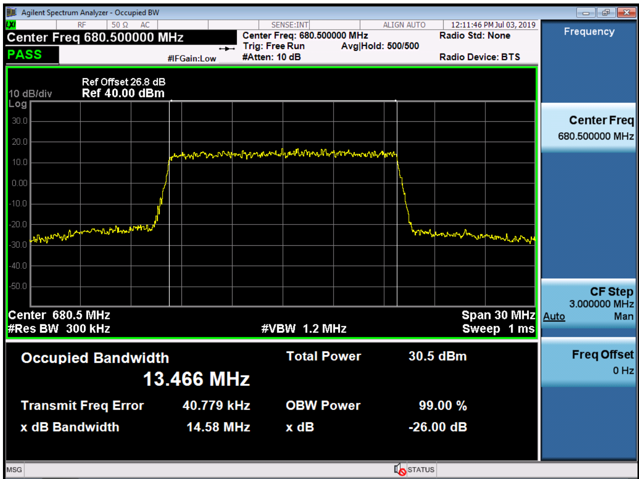
BAND 71. Occupied Bandwidth Plot (15M BW Ch.133297 64QAM_RB25_0)
