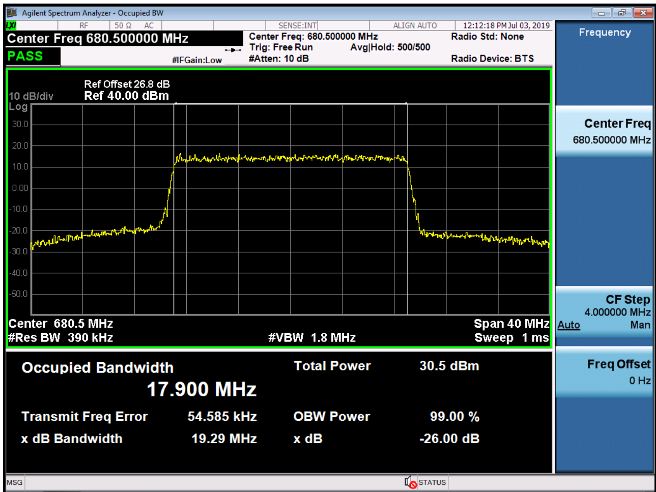
BAND 71. Occupied Bandwidth Plot (20M BW Ch.133297 64QAM_RB50_0)
