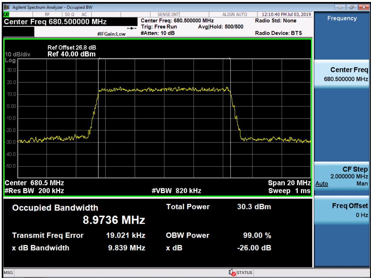
BAND 71. Occupied Bandwidth Plot (10M BW Ch.133297 64QAM_RB15_0)
