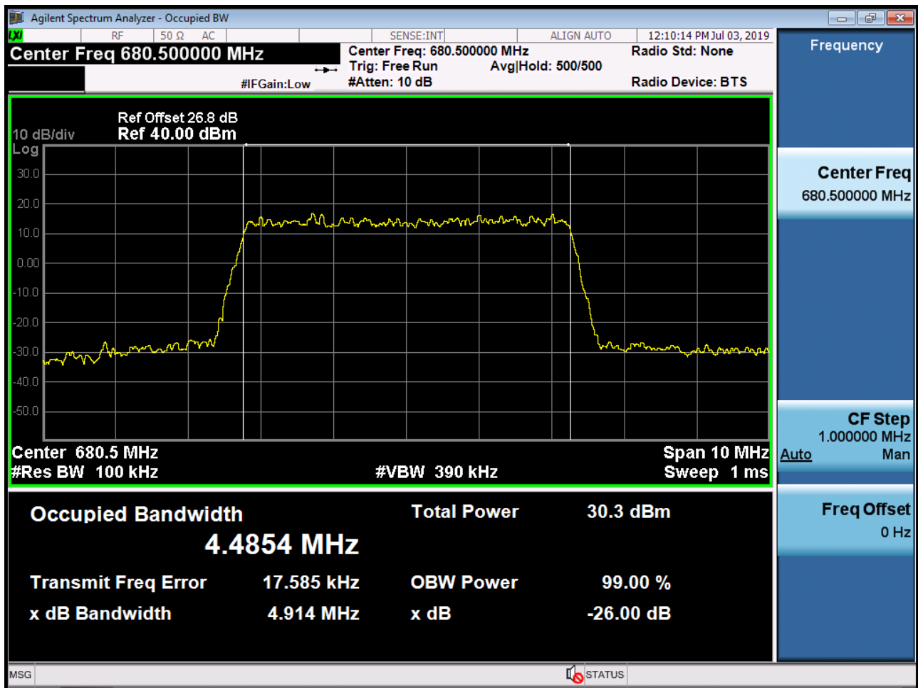
BAND 71. Occupied Bandwidth Plot (5M BW Ch.133297 64QAM_RB6_0)
