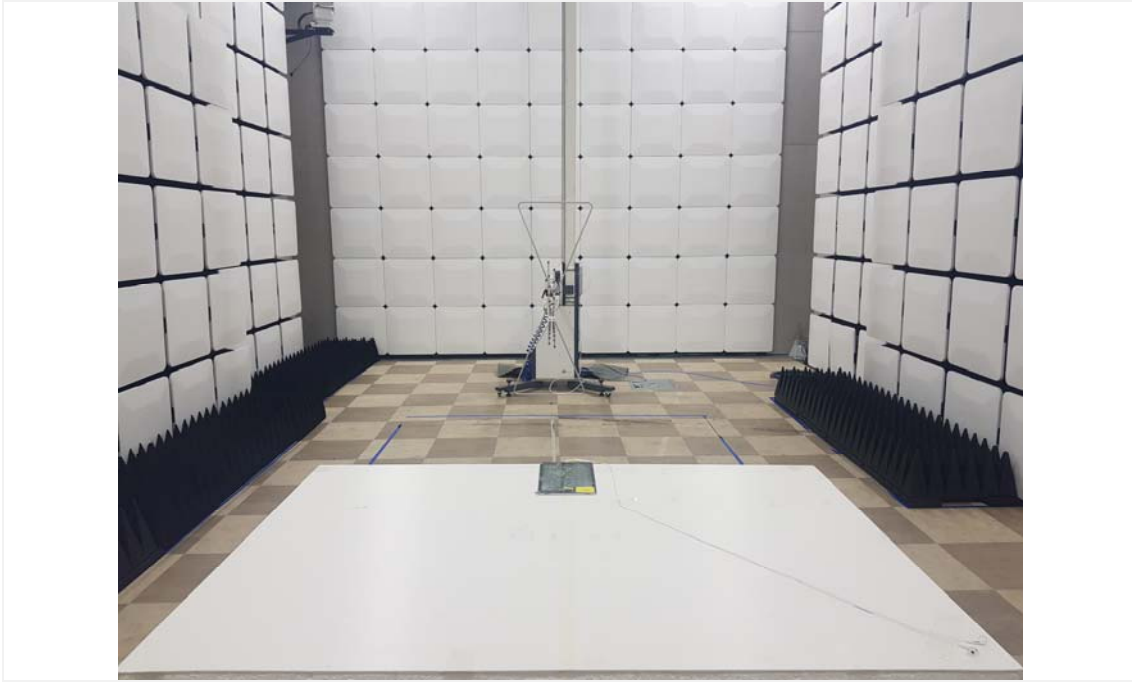
Earphone
