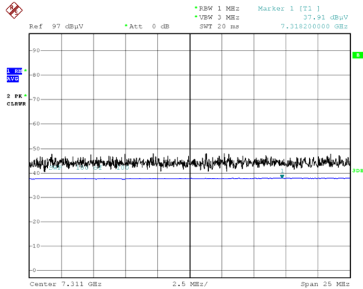
Radiated Spurious Emissions plot – Average Reading (802.11g, Ch.6 3rd Harmonic, H)
