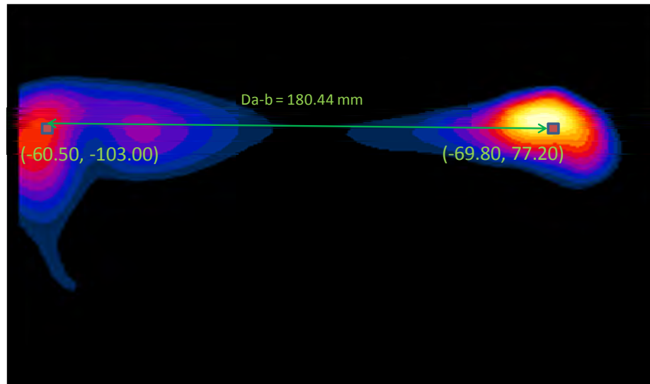
Figure 12-12 Peak SAR Locations of 2.4 GHz WLAN Ant. 2 and UMTS 1900 at 15 mm
