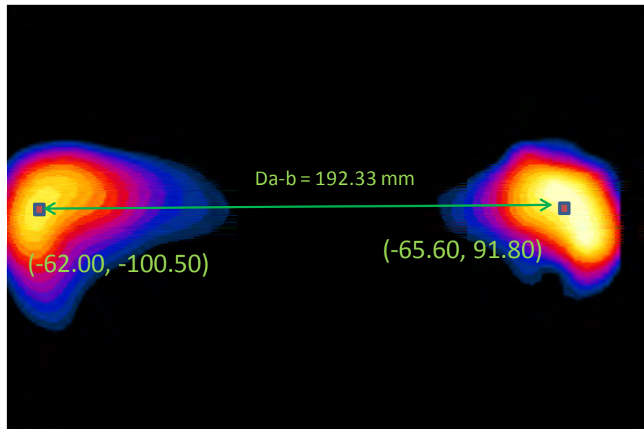
Figure 12-2 Peak SAR Locations of 2.4 GHz WLAN Ant. 1 and GPRS 1900 at 0 mm
