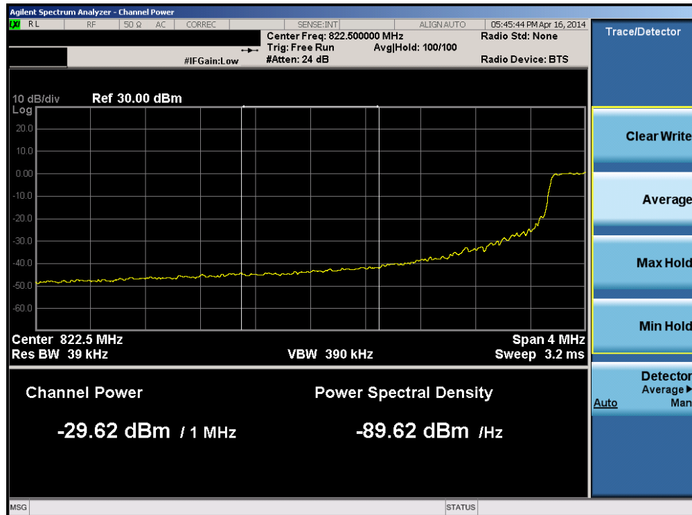
Plot 6-24. Lower Extended Band Edge Plot (Band 5 – 5.0MHz QPSK – RB Size 25)
