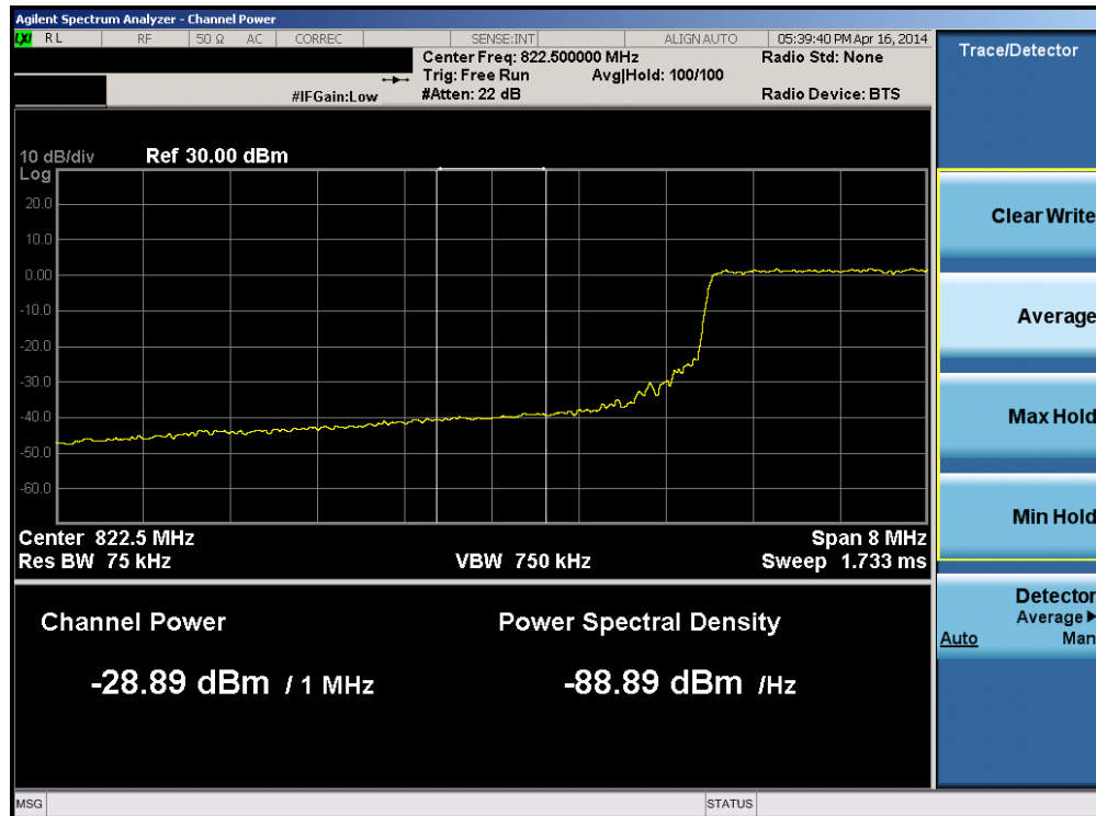
Plot 6-28. Lower Extended Band Edge Plot (Band 5 – 10.0MHz QPSK – RB Size 50)
