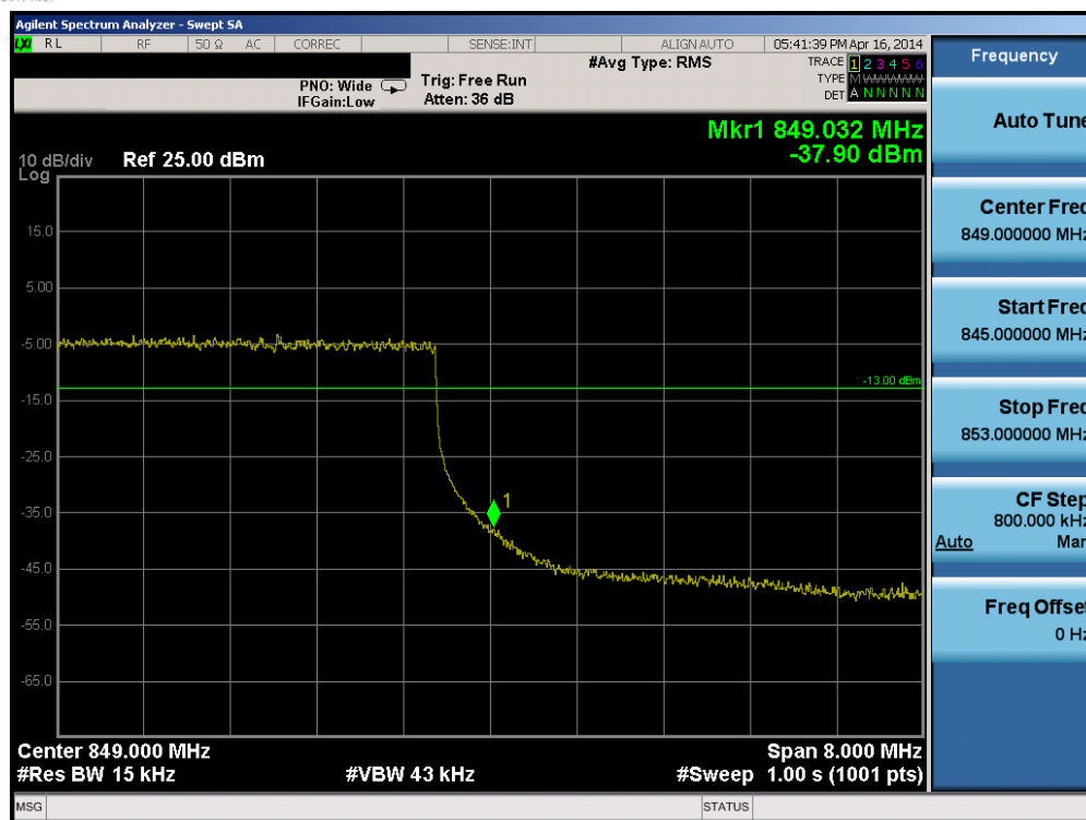
Plot 6-29. Upper Band Edge Plot (Band 5 – 10.0MHz QPSK – RB Size 50)
