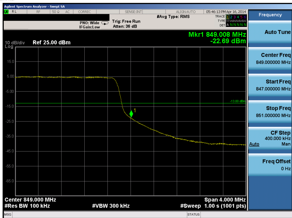
Plot 6-25. Upper Band Edge Plot (Band 5 – 5.0MHz QPSK – RB Size 25)
