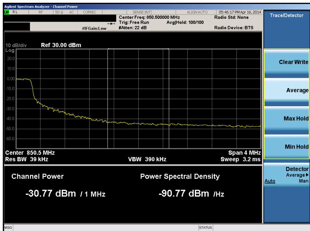
Plot 6-26. Upper Extended Band Edge Plot (Band 5 – 5.0MHz QPSK – RB Size 25)
