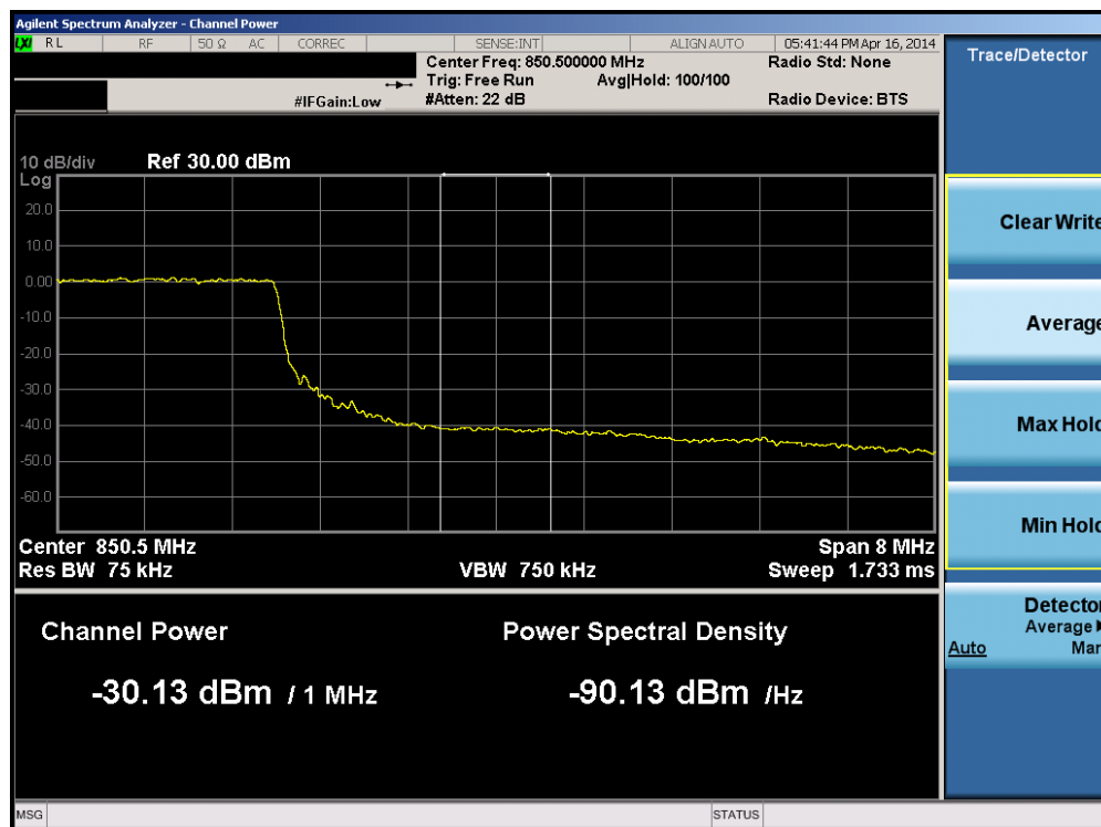
Plot 6-30. Upper Extended Band Edge Plot (Band 5 – 10.0MHz QPSK – RB Size 50)
