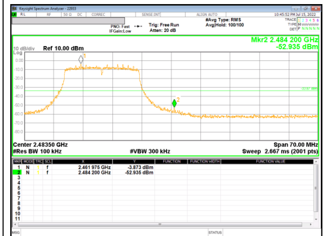
12 Channel Band-edge_SISO
