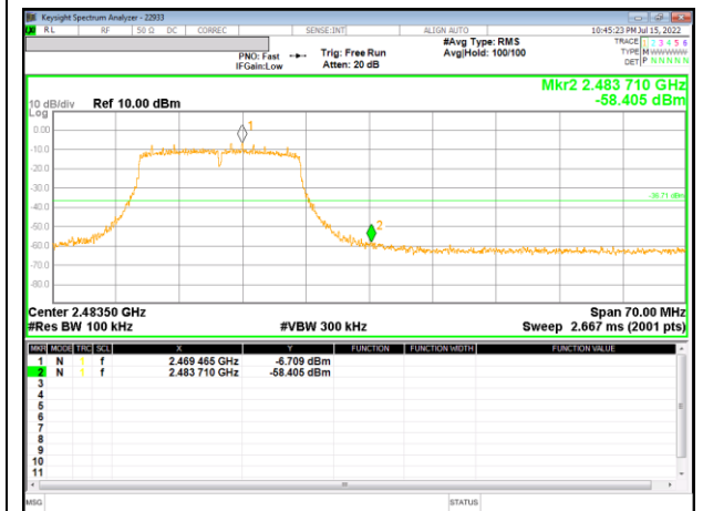
12 Channel Band-edge
