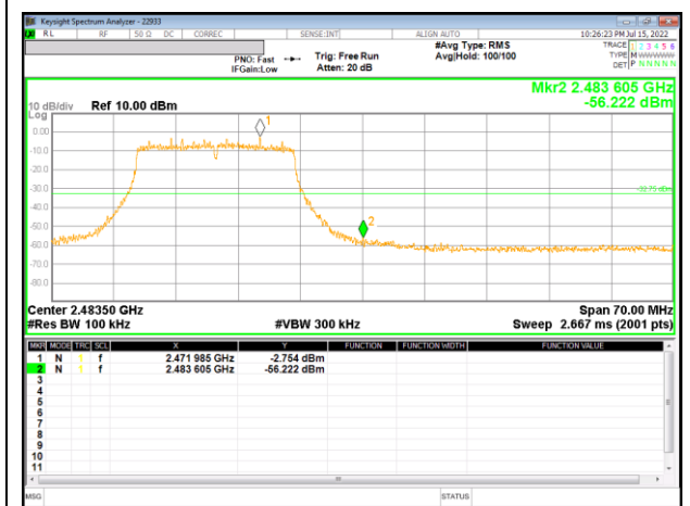
12 Channel Band-edge_SISO
