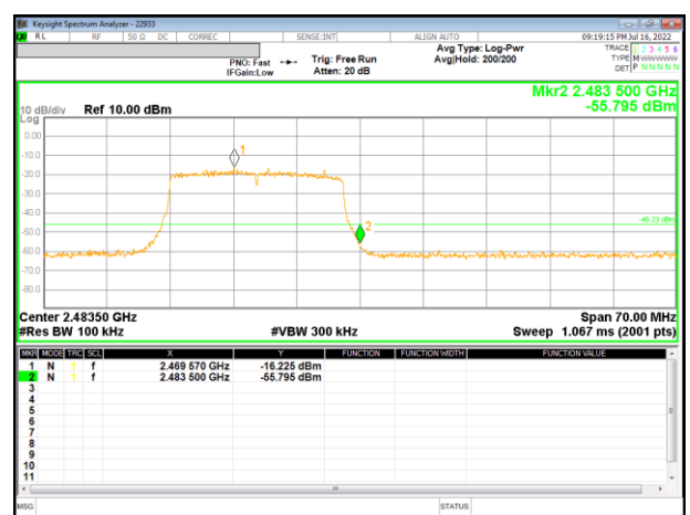
13 Channel Band-edge_SISO
