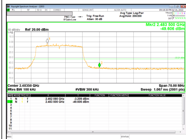
12 Channel Band-edge_SISO
