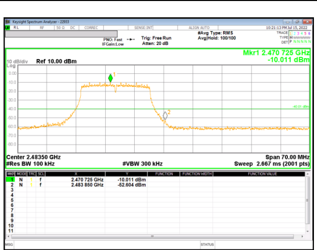
13 Channel Band-edge_SISO
