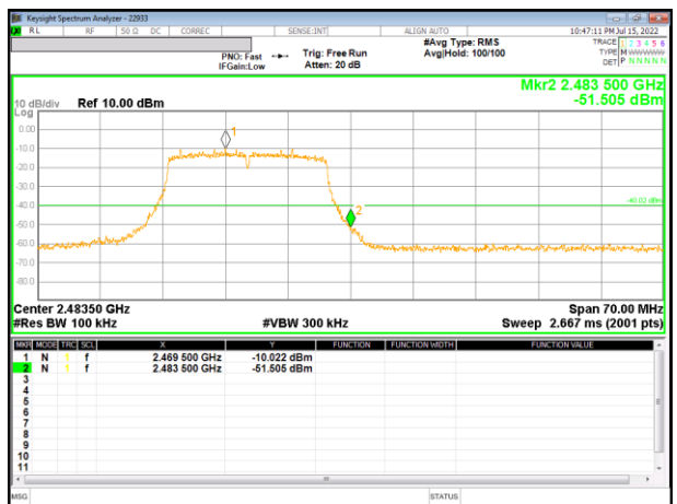
13 Channel Band-edge_SISO
