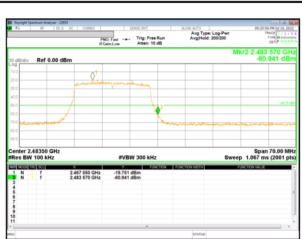
13 Channel Band-edge
