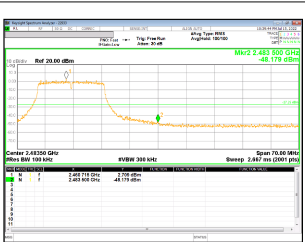
11 Channel Band-edge
