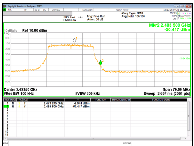
13 Channel Band-edge_SISO
