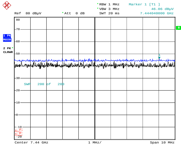
Radiated Spurious Emissions plot – Peak Reading (Ch.39 3rd Harmonic_H)
