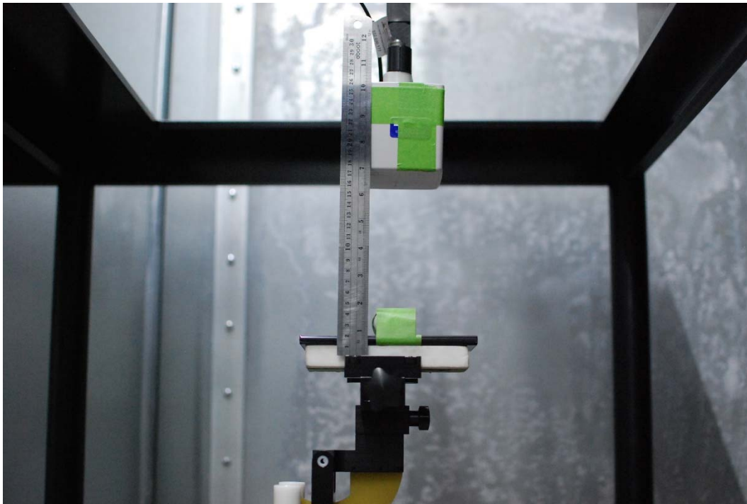
Test Setup Photo 16 H-field, Right edge, 15cm
