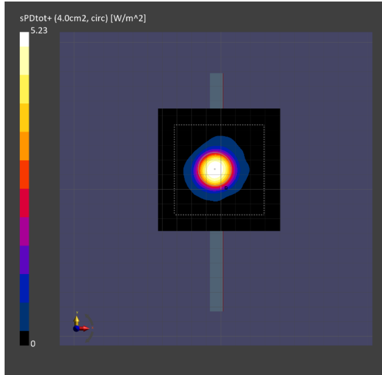
Figure 10-1 4cm 2 psPD distribution measured at input.power.limit of 11.2 dBm on the right edge for n261 beam 1
