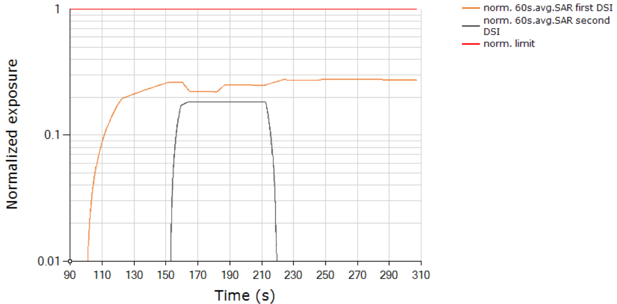
Total Normalized Time-averaged RF Exposure Tech: LTE, Band 48
