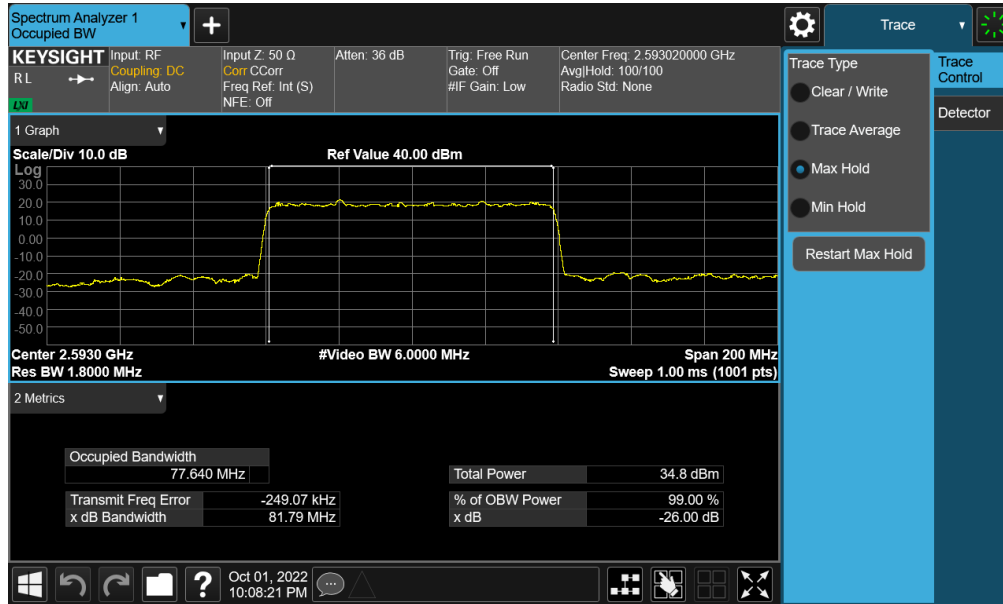
Plot 7-121. Occupied Bandwidth Plot (NR Band n41 - 80MHz \pi/2 BPSK - Full RB - Ant F)
