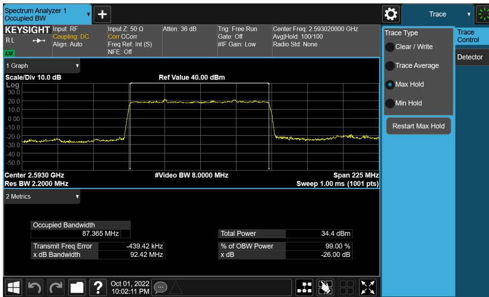
Plot 7-118. Occupied Bandwidth Plot (NR Band n41 - 90MHz \pi/2 BPSK - Full RB - Ant F)
