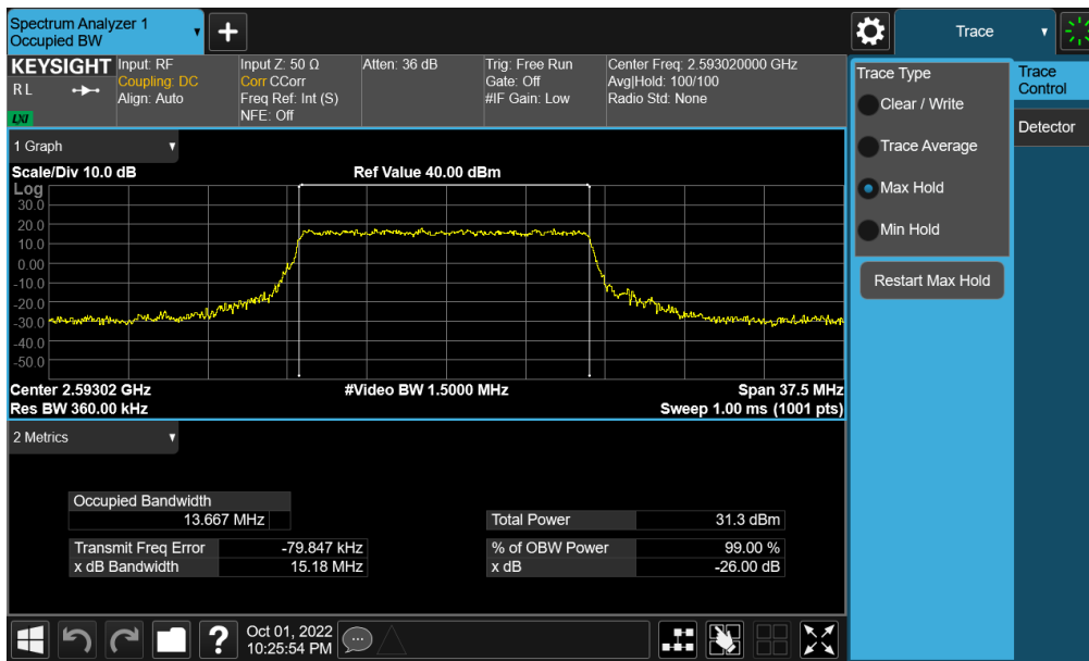
Plot 7-144. Occupied Bandwidth Plot (NR Band n41 - 15MHz 16-QAM - Full RB - Ant F)
