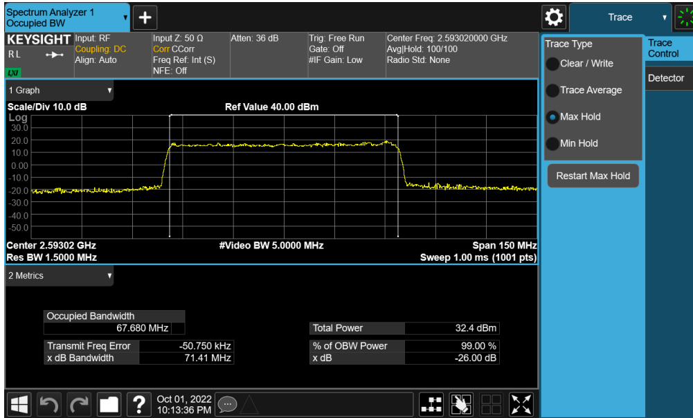
Plot 7-125. Occupied Bandwidth Plot (NR Band n41 - 70MHz QPSK - Full RB - Ant F)
