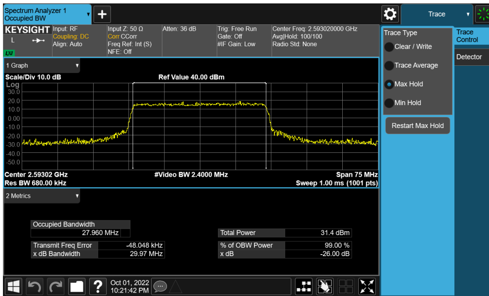
Plot 7-138. Occupied Bandwidth Plot (NR Band n41 - 30MHz 16-QAM - Full RB - Ant F)
