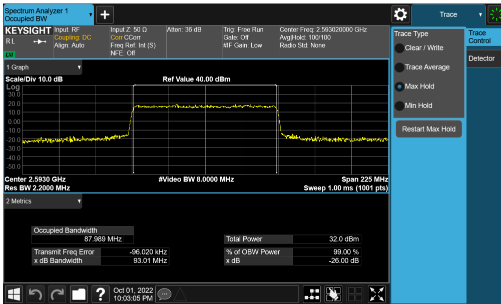
Plot 7-120. Occupied Bandwidth Plot (NR Band n41 - 90MHz 16-QAM - Full RB - Ant F)
