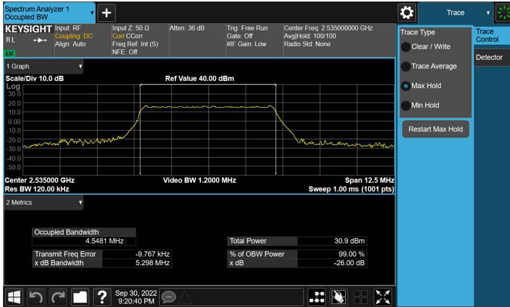
Plot 7-112. Occupied Bandwidth Plot (NR Band n7 - 5MHz \pi/2 BPSK - Full RB - Ant F)
