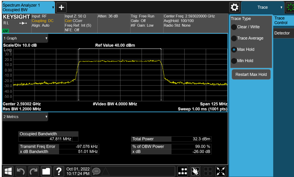
Plot 7-131. Occupied Bandwidth Plot (NR Band n41 - 50MHz QPSK - Full RB - Ant F)
