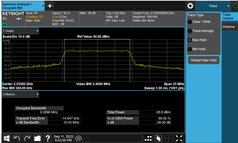
Plot 7-89. Occupied Bandwidth Plot (NR Band n7 - 10MHz QPSK - Full RB - Ant B)
