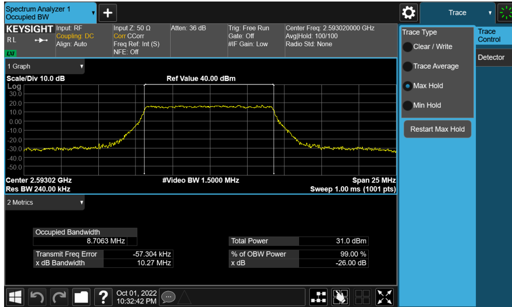
Plot 7-147. Occupied Bandwidth Plot (NR Band n41 - 10MHz 16-QAM - Full RB - Ant F)
