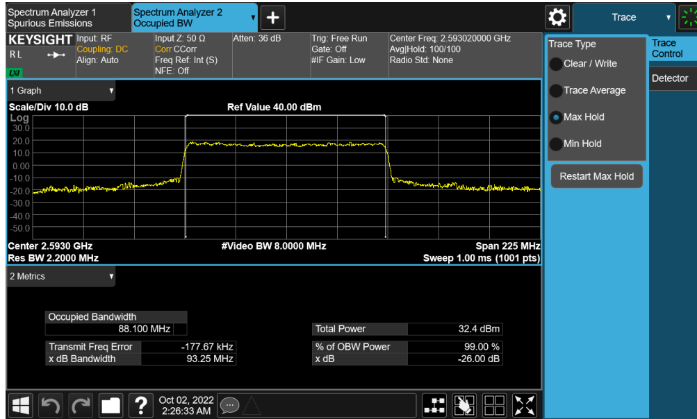
Plot 7-152. Occupied Bandwidth Plot (NR Band n41 - 90MHz QPSK - Full RB - Switching - Ant B)
