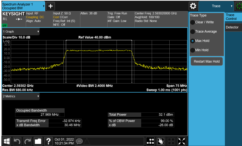
Plot 7-137. Occupied Bandwidth Plot (NR Band n41 - 30MHz QPSK - Full RB - Ant F)
