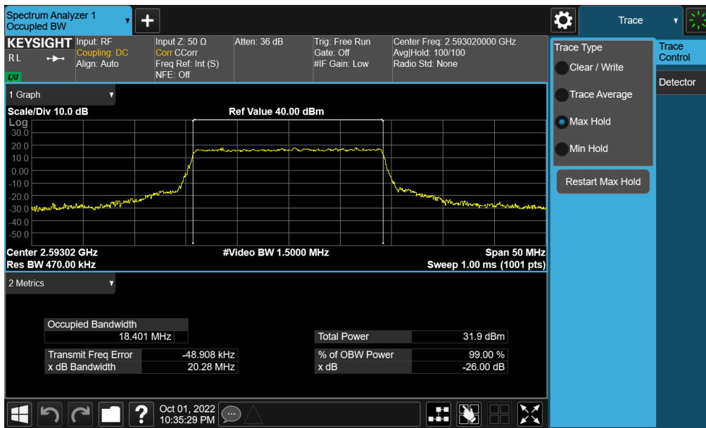
Plot 7-140. Occupied Bandwidth Plot (NR Band n41 - 20MHz QPSK - Full RB - Ant F)
