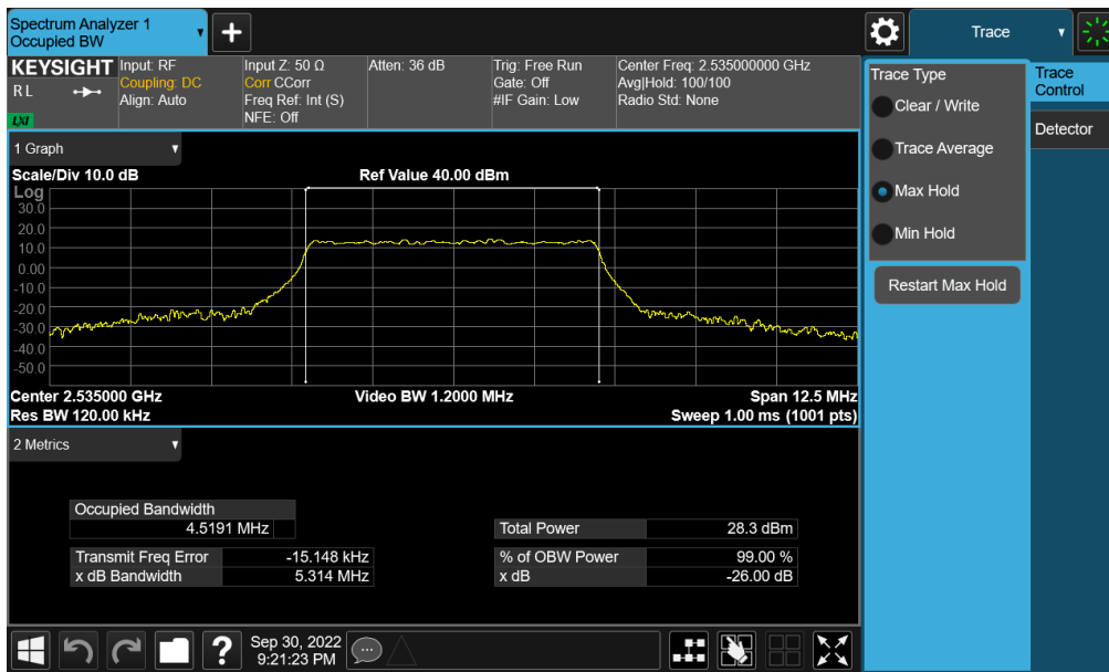
Plot 7-113. Occupied Bandwidth Plot (NR Band n7 - 5MHz QPSK - Full RB - Ant F)
