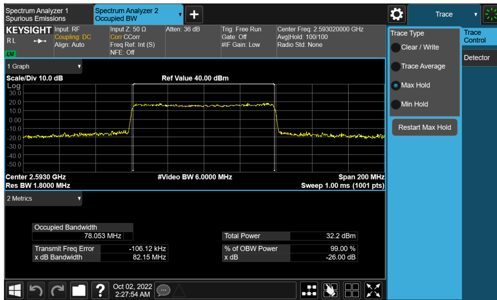
Plot 7-155. Occupied Bandwidth Plot (NR Band n41 - 80MHz QPSK - Full RB - Switching - Ant B)
