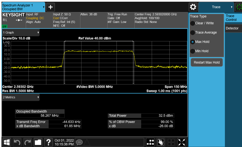
Plot 7-128. Occupied Bandwidth Plot (NR Band n41 - 60MHz QPSK - Full RB - Ant F)
