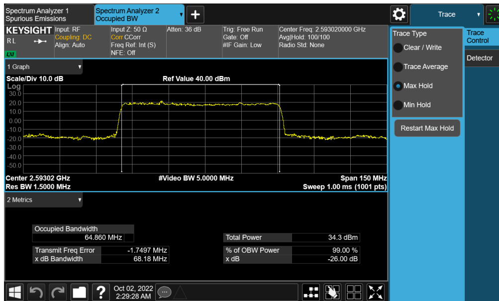
Plot 7-157. Occupied Bandwidth Plot (NR Band n41 - 70MHz \pi/2 BPSK - Full RB - Switching - Ant B)
