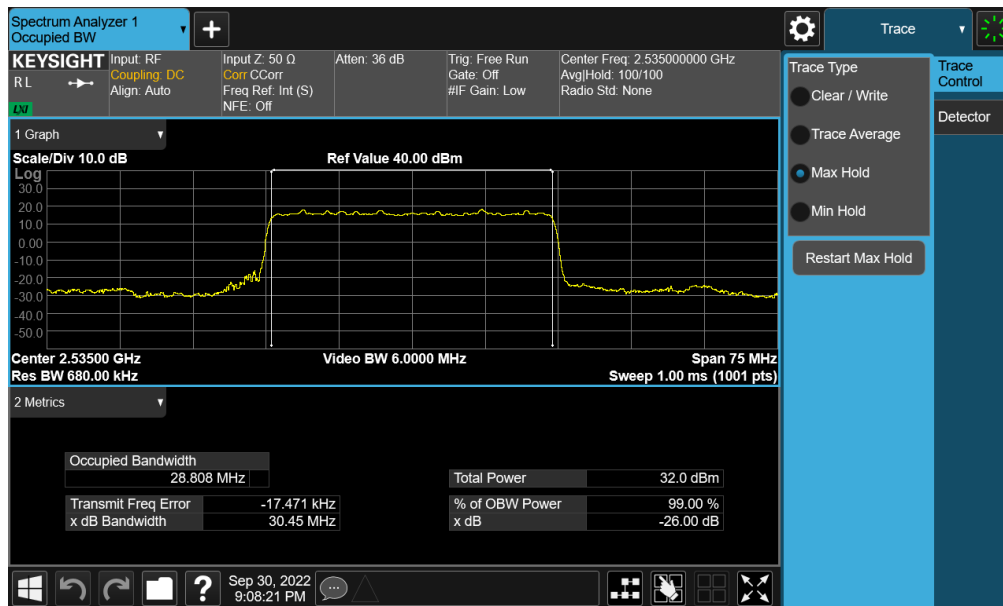
Plot 7-97. Occupied Bandwidth Plot (NR Band n7 - 30MHz \pi/2 BPSK - Full RB - Ant F)
