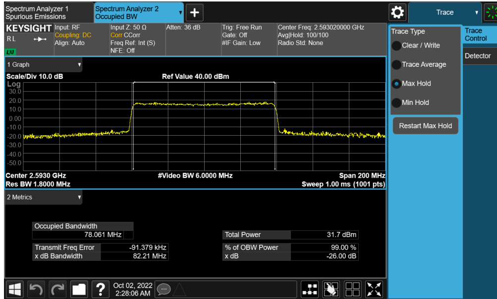
Plot 7-156. Occupied Bandwidth Plot (NR Band n41 - 80MHz 16-QAM - Full RB - Switching - Ant B)
