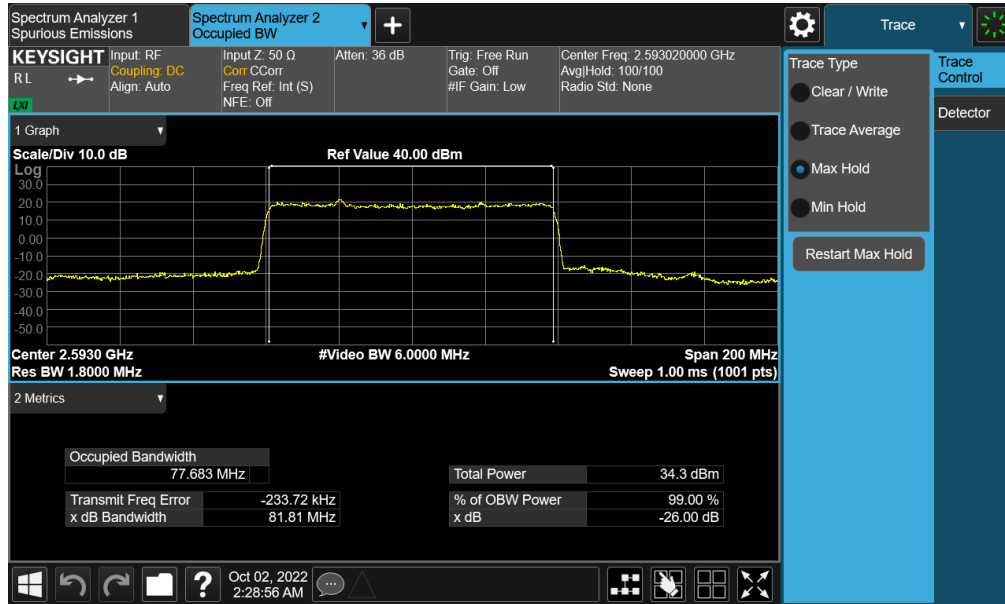
Plot 7-154. Occupied Bandwidth Plot (NR Band n41 - 80MHz \pi/2 BPSK - Full RB - Switching - Ant B)
