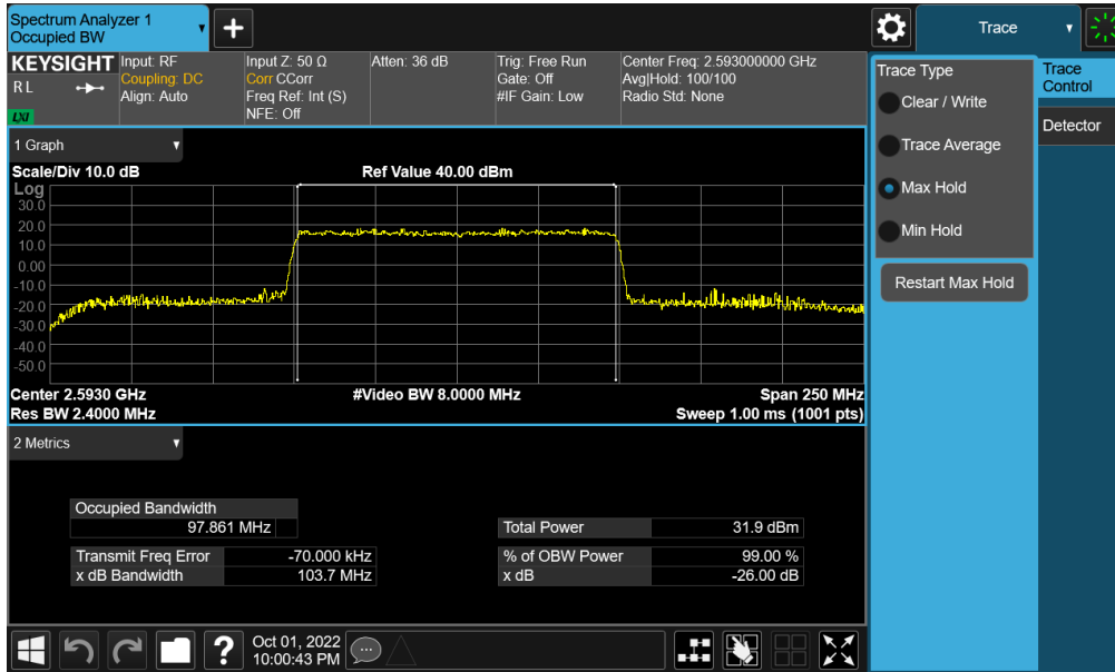
Plot 7-117. Occupied Bandwidth Plot (NR Band n41 - 100MHz 16-QAM - Full RB - Ant F)
