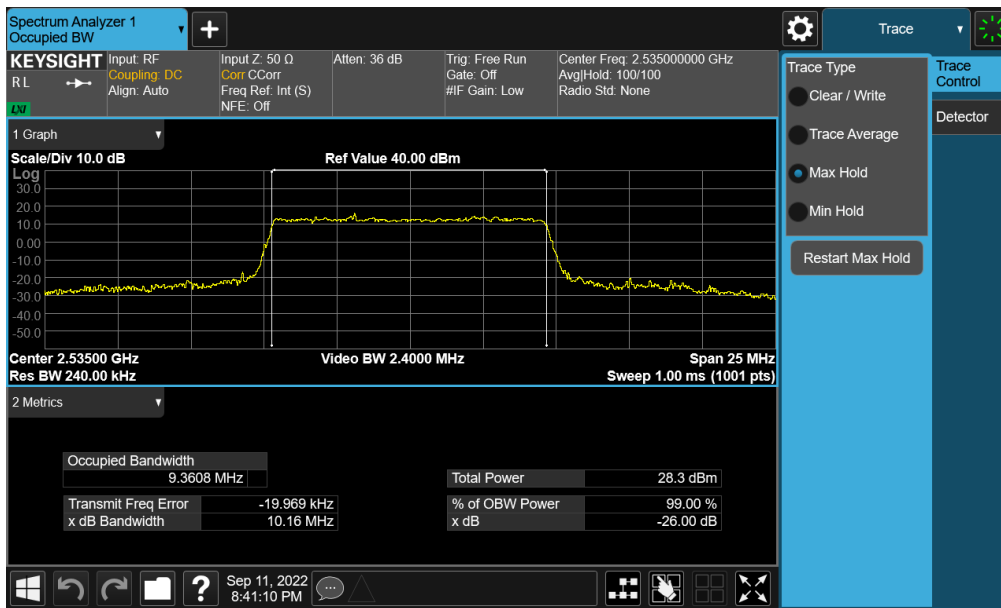
Plot 7-90. Occupied Bandwidth Plot (NR Band n7 - 10MHz 16-QAM - Full RB - Ant B)
