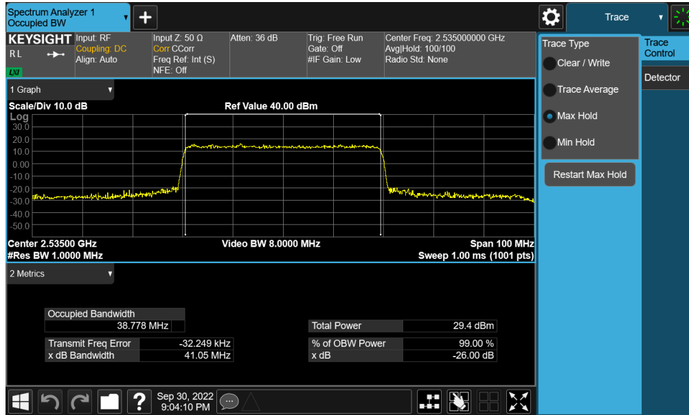
Plot 7-96. Occupied Bandwidth Plot (NR Band n7 - 40MHz 16-QAM - Full RB - Ant F)
