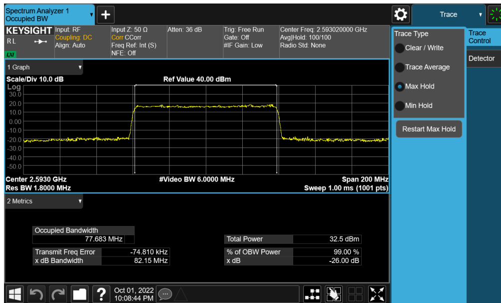
Plot 7-122. Occupied Bandwidth Plot (NR Band n41 - 80MHz QPSK - Full RB - Ant F)
