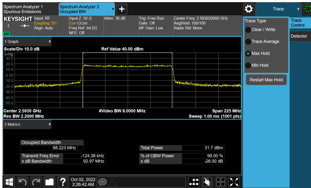
Plot 7-153. Occupied Bandwidth Plot (NR Band n41 - 90MHz 16-QAM - Full RB - Switching - Ant B)
