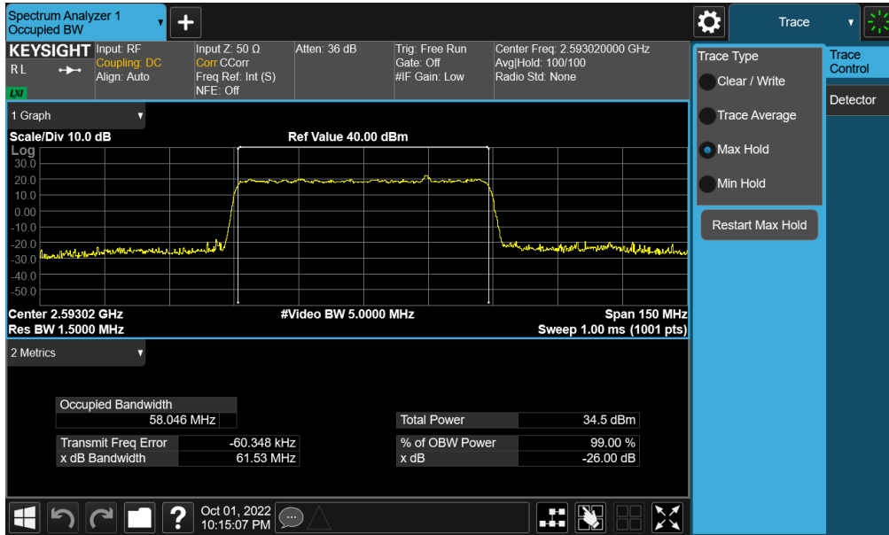
Plot 7-127. Occupied Bandwidth Plot (NR Band n41 - 60MHz \pi/2 BPSK - Full RB - Ant F)
