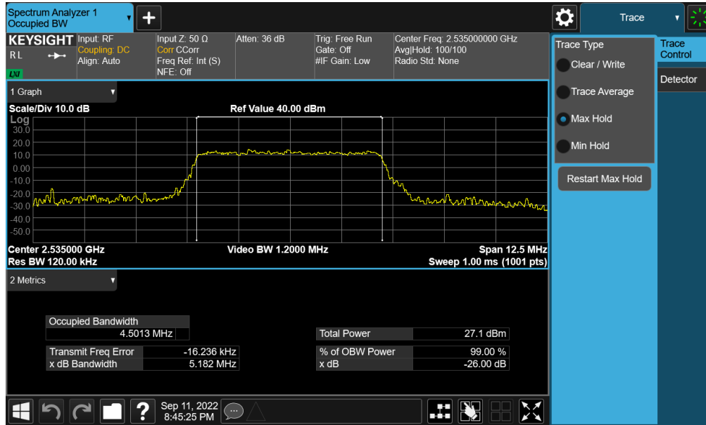
Plot 7-93. Occupied Bandwidth Plot (NR Band n7 - 5MHz 16-QAM - Full RB - Ant B)
