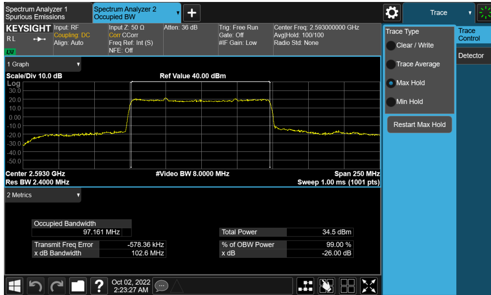
Plot 7-148. Occupied Bandwidth Plot (NR Band n41 - 100MHz \pi/2 BPSK - Full RB - Switching - Ant B)
