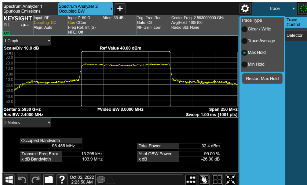
Plot 7-149. Occupied Bandwidth Plot (NR Band n41 - 100MHz QPSK - Full RB - Switching - Ant B)
