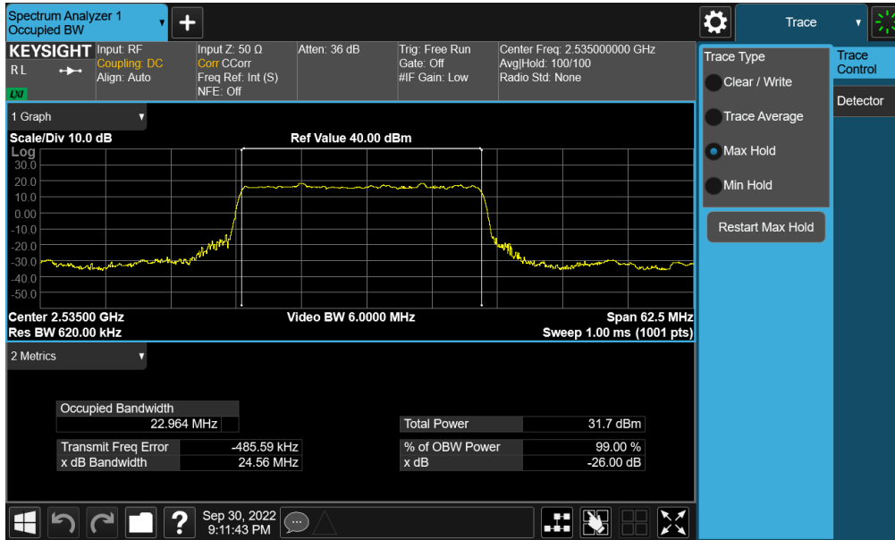
Plot 7-100. Occupied Bandwidth Plot (NR Band n7 - 25MHz \pi/2 BPSK - Full RB - Ant F)
