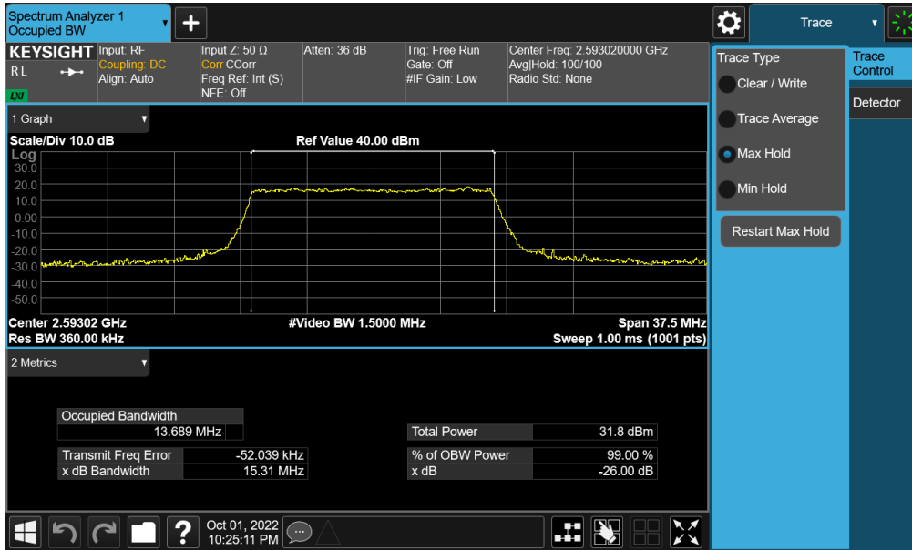
Plot 7-143. Occupied Bandwidth Plot (NR Band n41 - 15MHz QPSK - Full RB - Ant F)
