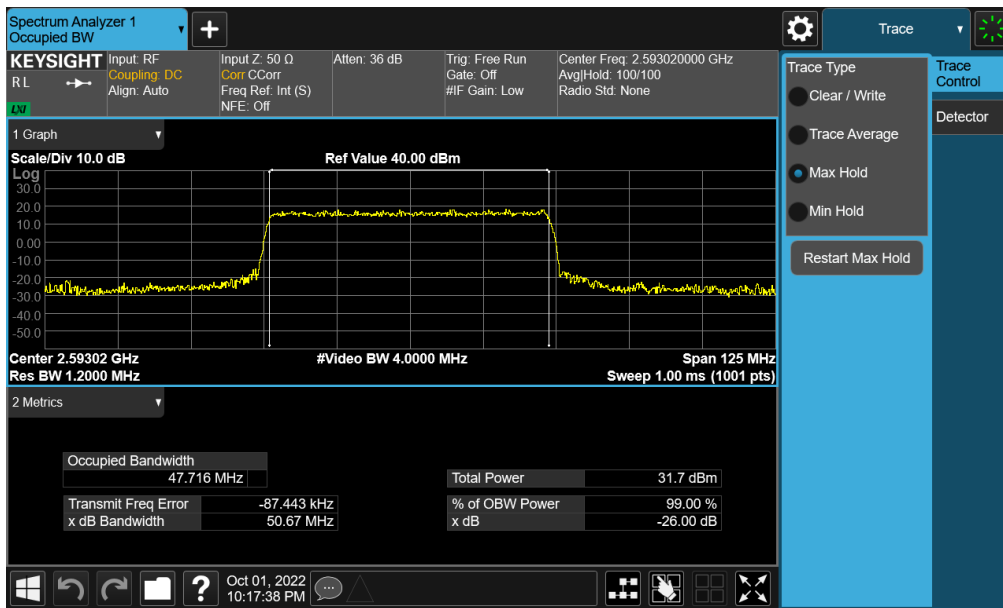
Plot 7-132. Occupied Bandwidth Plot (NR Band n41 - 50MHz 16-QAM - Full RB - Ant F)
