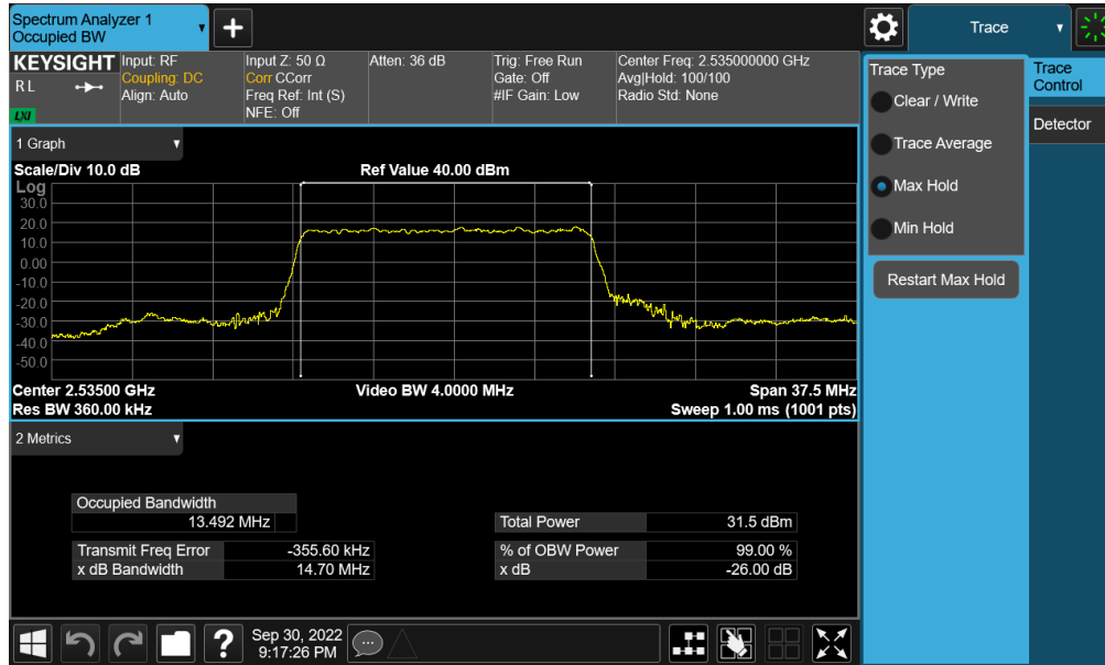
Plot 7-106. Occupied Bandwidth Plot (NR Band n7 - 15MHz \pi/2 BPSK - Full RB - Ant F)
