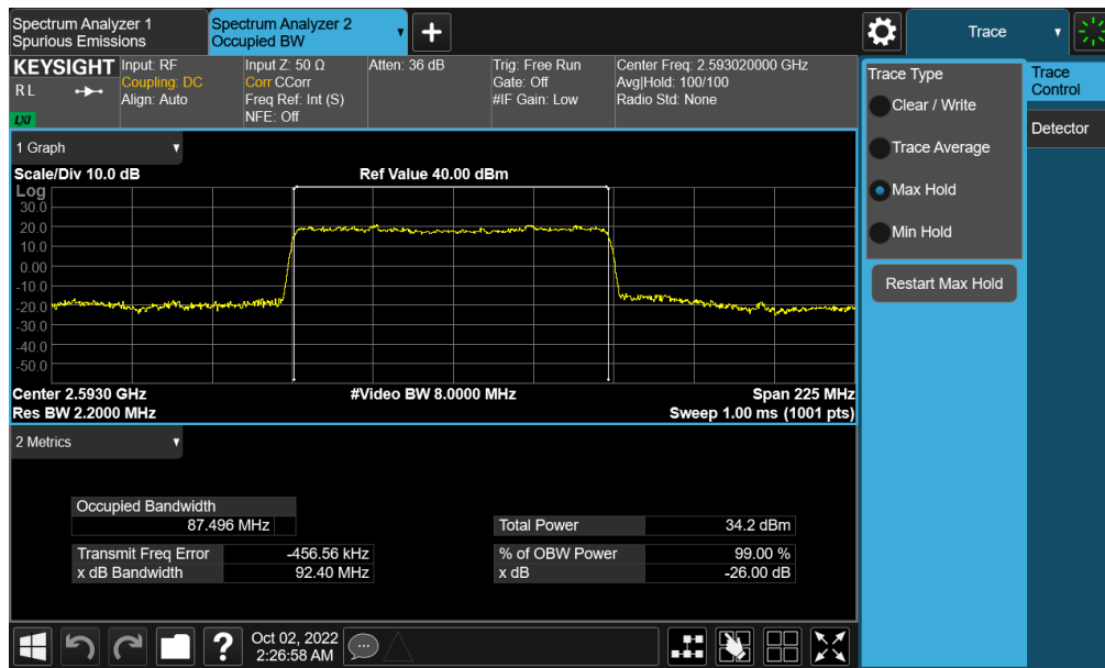
Plot 7-151. Occupied Bandwidth Plot (NR Band n41 - 90MHz \pi/2 BPSK - Full RB - Switching - Ant B)
