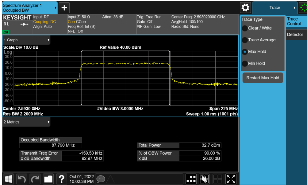
Plot 7-119. Occupied Bandwidth Plot (NR Band n41 - 90MHz QPSK - Full RB - Ant F)
