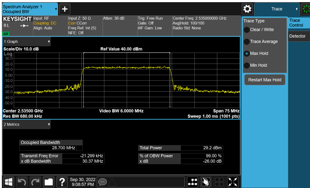
Plot 7-99. Occupied Bandwidth Plot (NR Band n7 - 30MHz 16-QAM - Full RB - Ant F)
