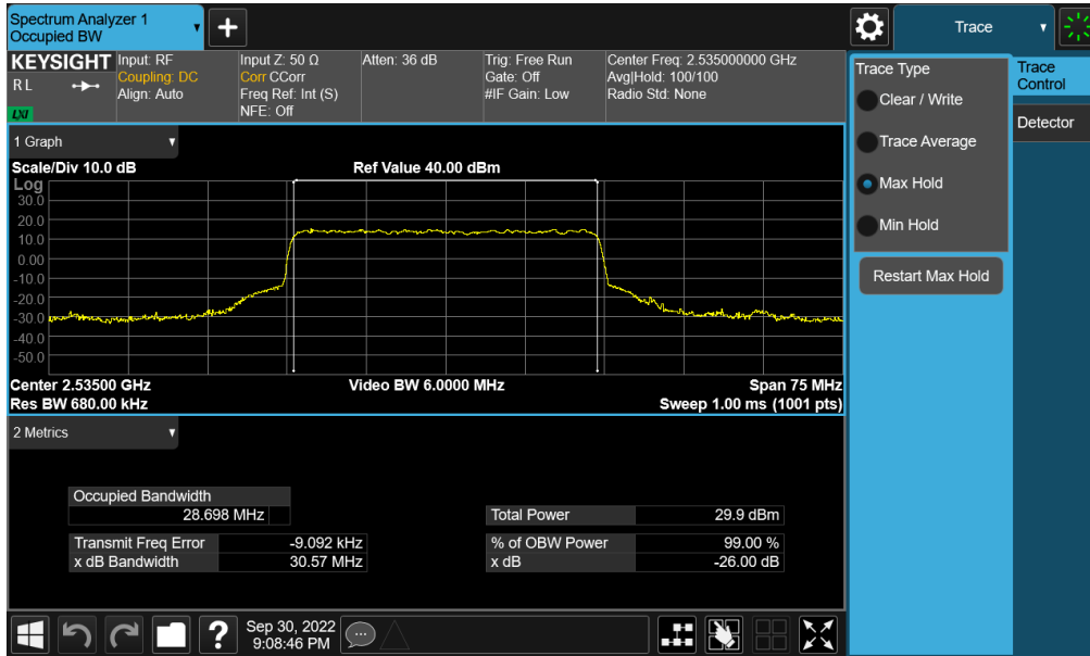
Plot 7-98. Occupied Bandwidth Plot (NR Band n7 - 30MHz QPSK - Full RB - Ant F)
