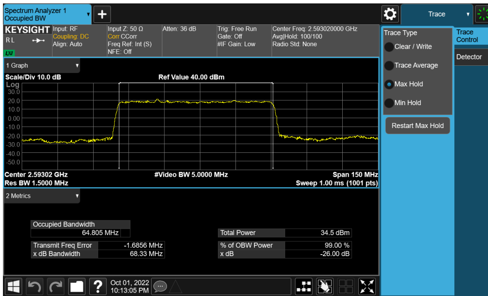
Plot 7-124. Occupied Bandwidth Plot (NR Band n41 - 70MHz \pi/2 BPSK - Full RB - Ant F)
