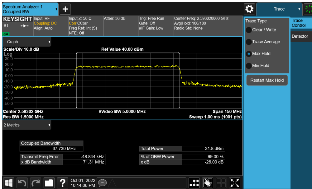
Plot 7-126. Occupied Bandwidth Plot (NR Band n41 - 70MHz 16-QAM - Full RB - Ant F)
