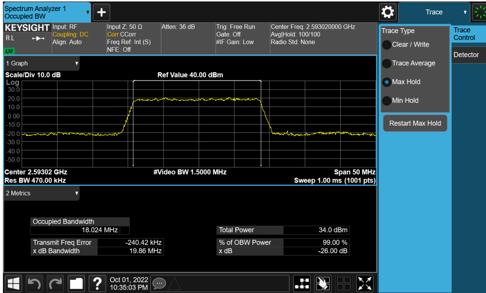
Plot 7-139. Occupied Bandwidth Plot (NR Band n41 - 20MHz \pi/2 BPSK - Full RB - Ant F)
