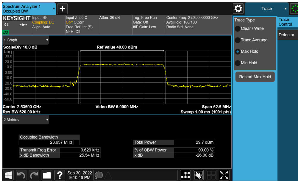
Plot 7-101. Occupied Bandwidth Plot (NR Band n7 - 25MHz QPSK - Full RB - Ant F)
