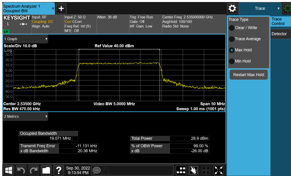
Plot 7-105. Occupied Bandwidth Plot (NR Band n7 - 20MHz 16-QAM - Full RB - Ant F)
