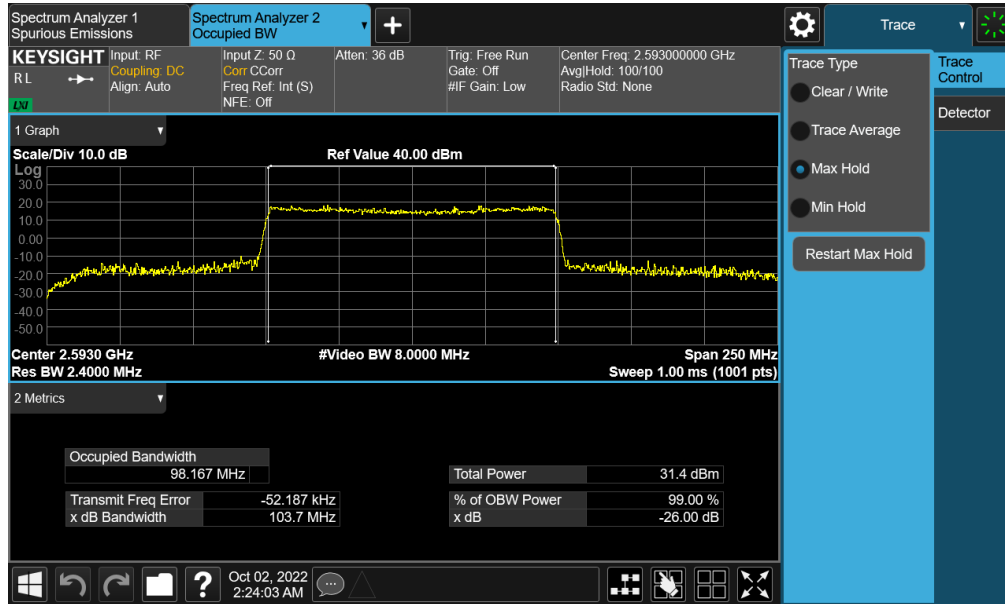
Plot 7-150. Occupied Bandwidth Plot (NR Band n41 - 100MHz 16-QAM - Full RB - Switching - Ant B)
