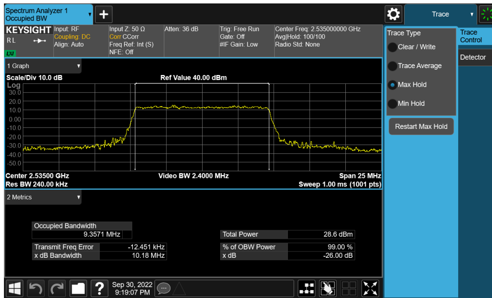
Plot 7-111. Occupied Bandwidth Plot (NR Band n7 - 10MHz 16-QAM - Full RB - Ant F)
