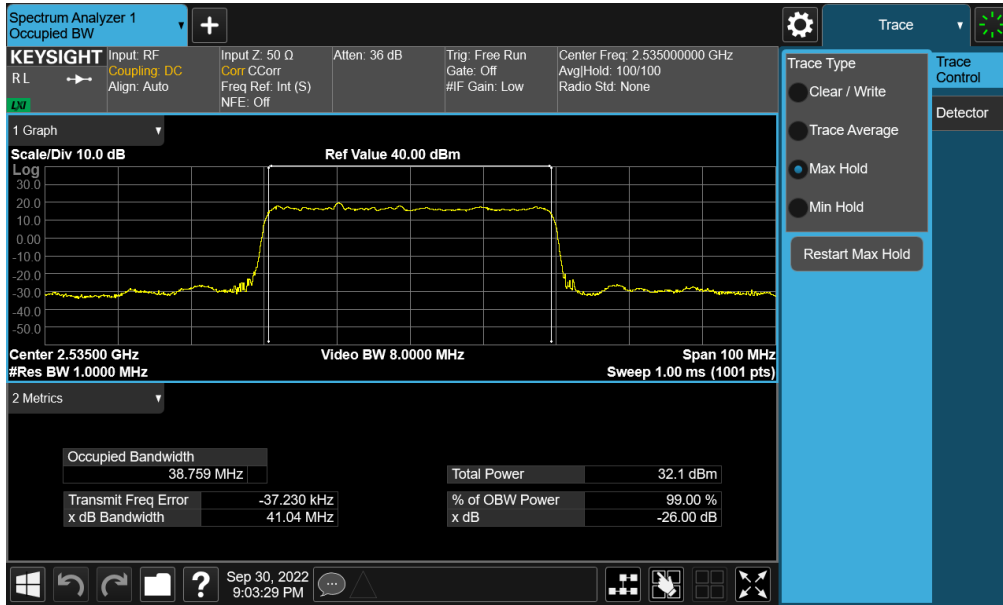
Plot 7-94. Occupied Bandwidth Plot (NR Band n7 - 40MHz \pi/2 BPSK - Full RB - Ant F)
