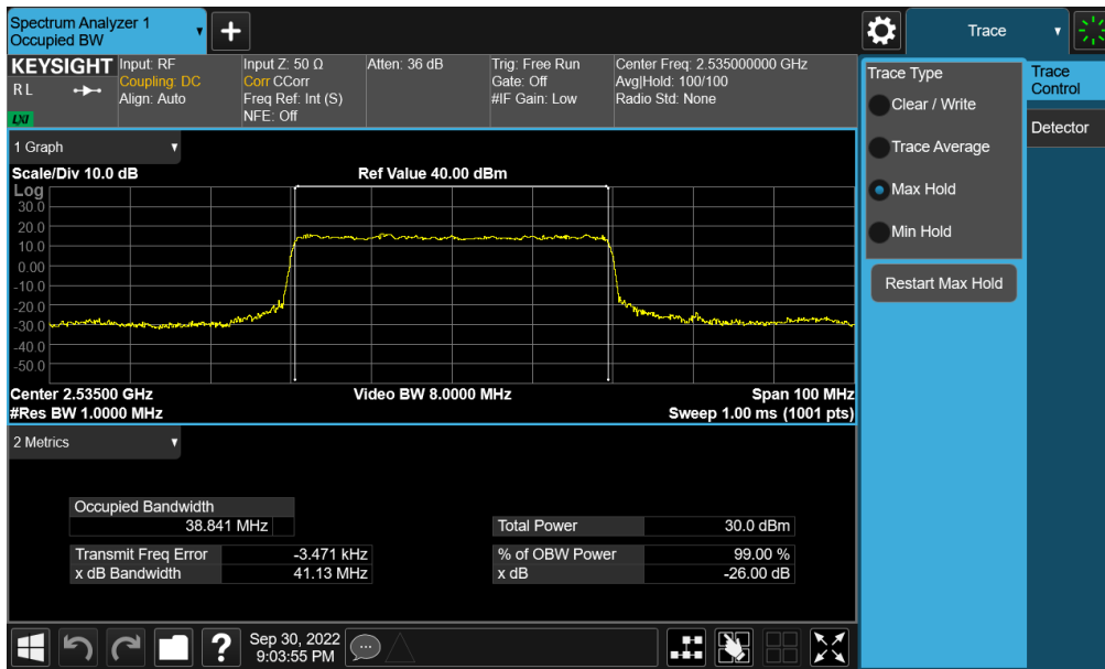
Plot 7-95. Occupied Bandwidth Plot (NR Band n7 - 40MHz QPSK - Full RB - Ant F)
