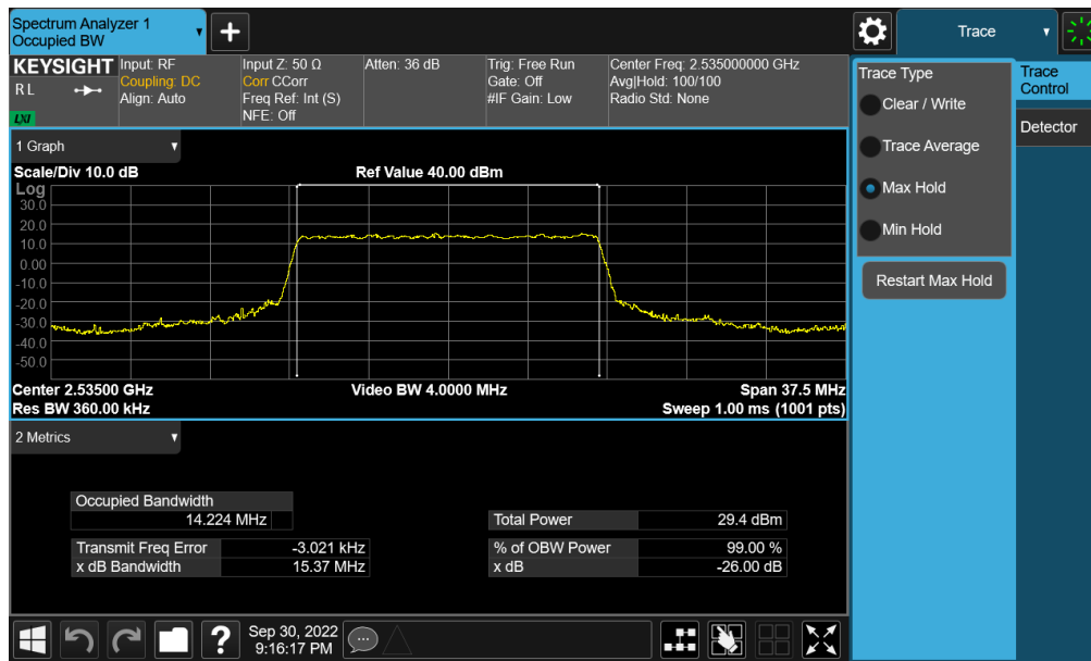
Plot 7-107. Occupied Bandwidth Plot (NR Band n7 - 15MHz QPSK - Full RB - Ant F)
