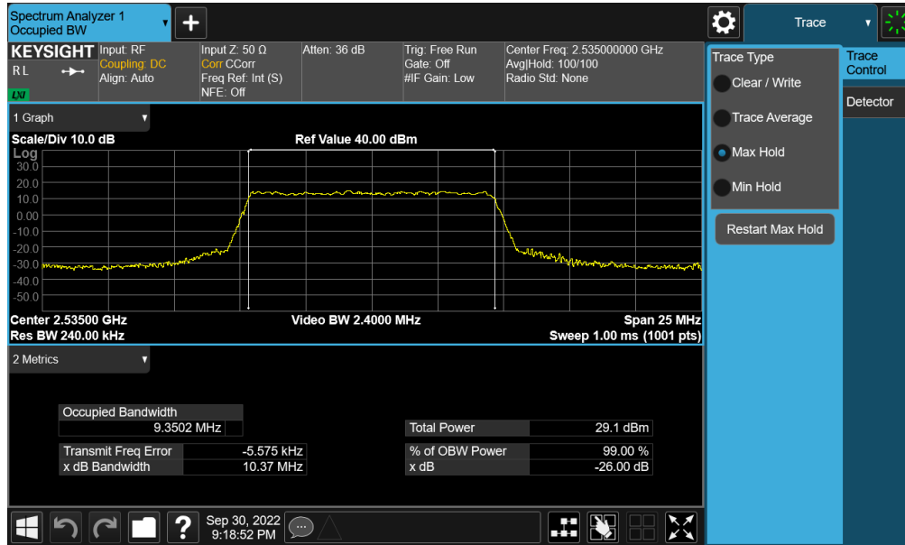
Plot 7-110. Occupied Bandwidth Plot (NR Band n7 - 10MHz QPSK - Full RB - Ant F)
