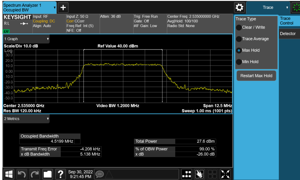
Plot 7-114. Occupied Bandwidth Plot (NR Band n7 - 5MHz 16-QAM - Full RB - Ant F)
