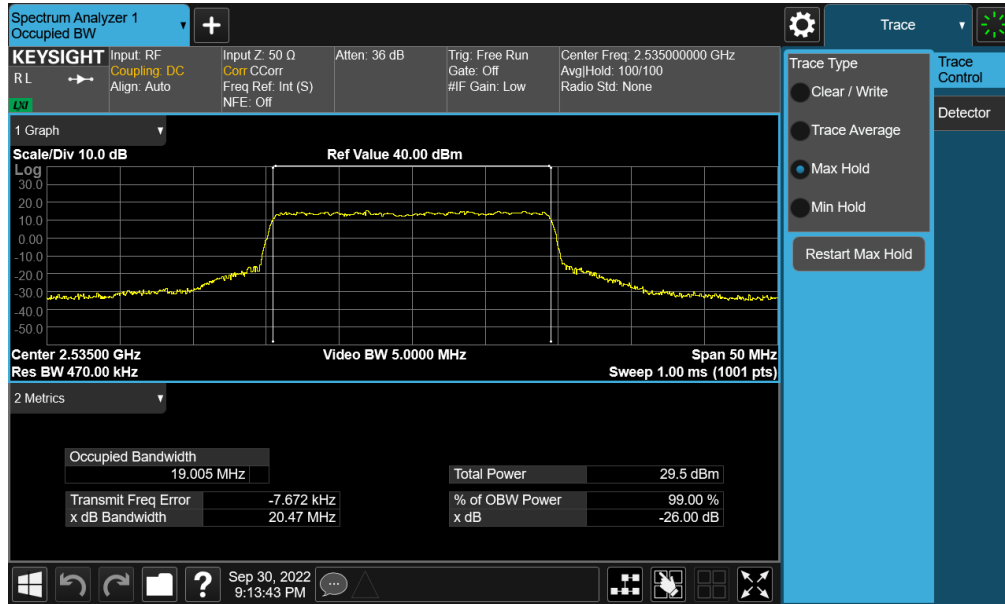
Plot 7-104. Occupied Bandwidth Plot (NR Band n7 - 20MHz QPSK - Full RB - Ant F)
